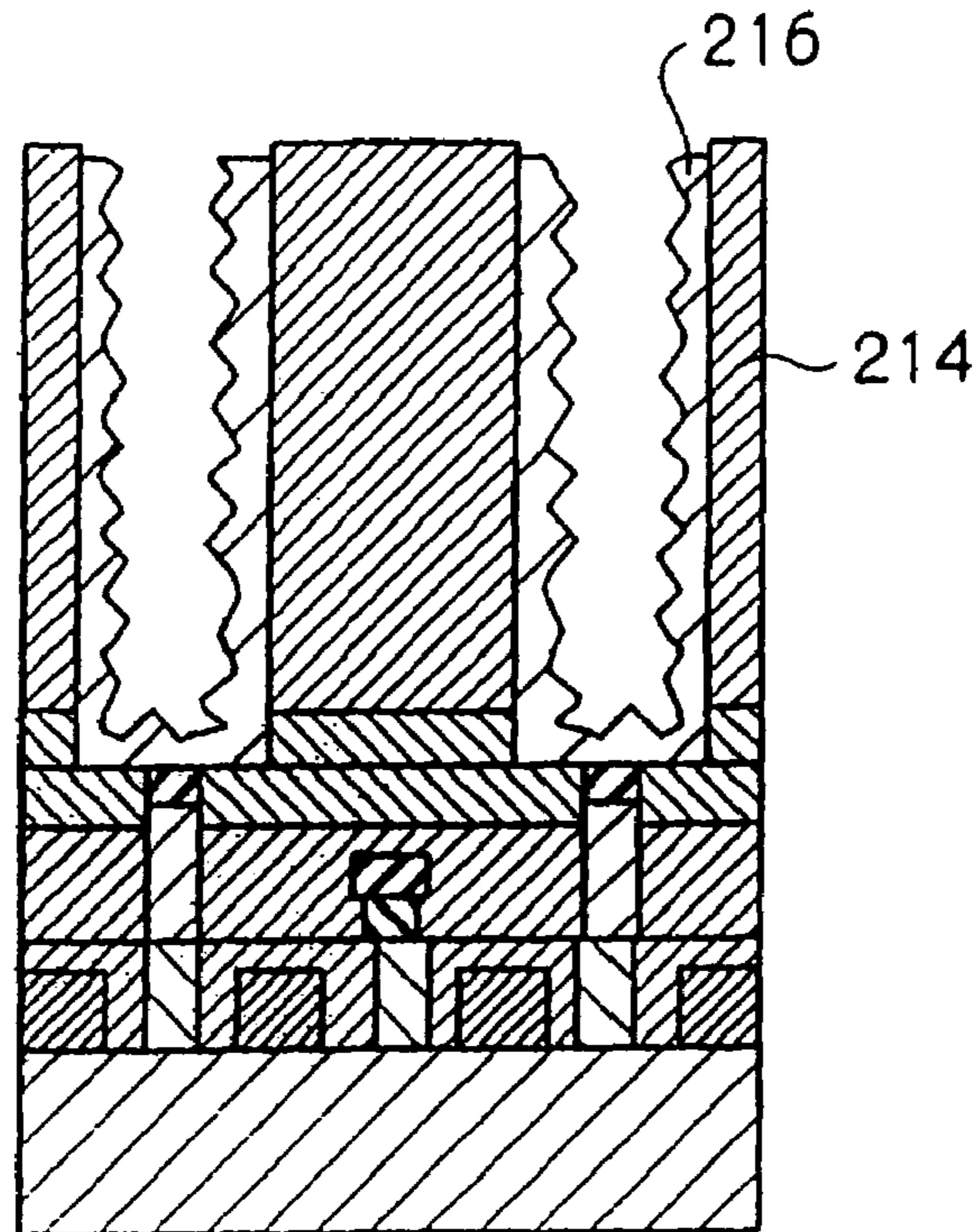
FIG. 2F (PRIOR ART)
