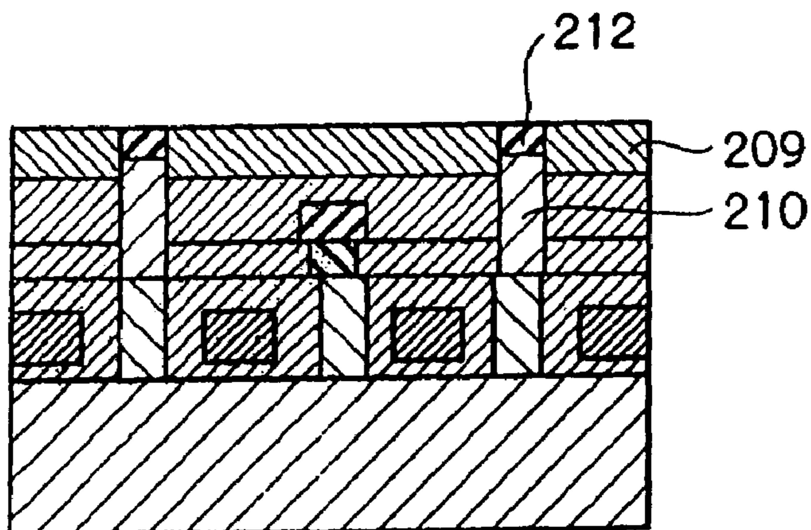
FIG. 2C (PRIOR ART)
