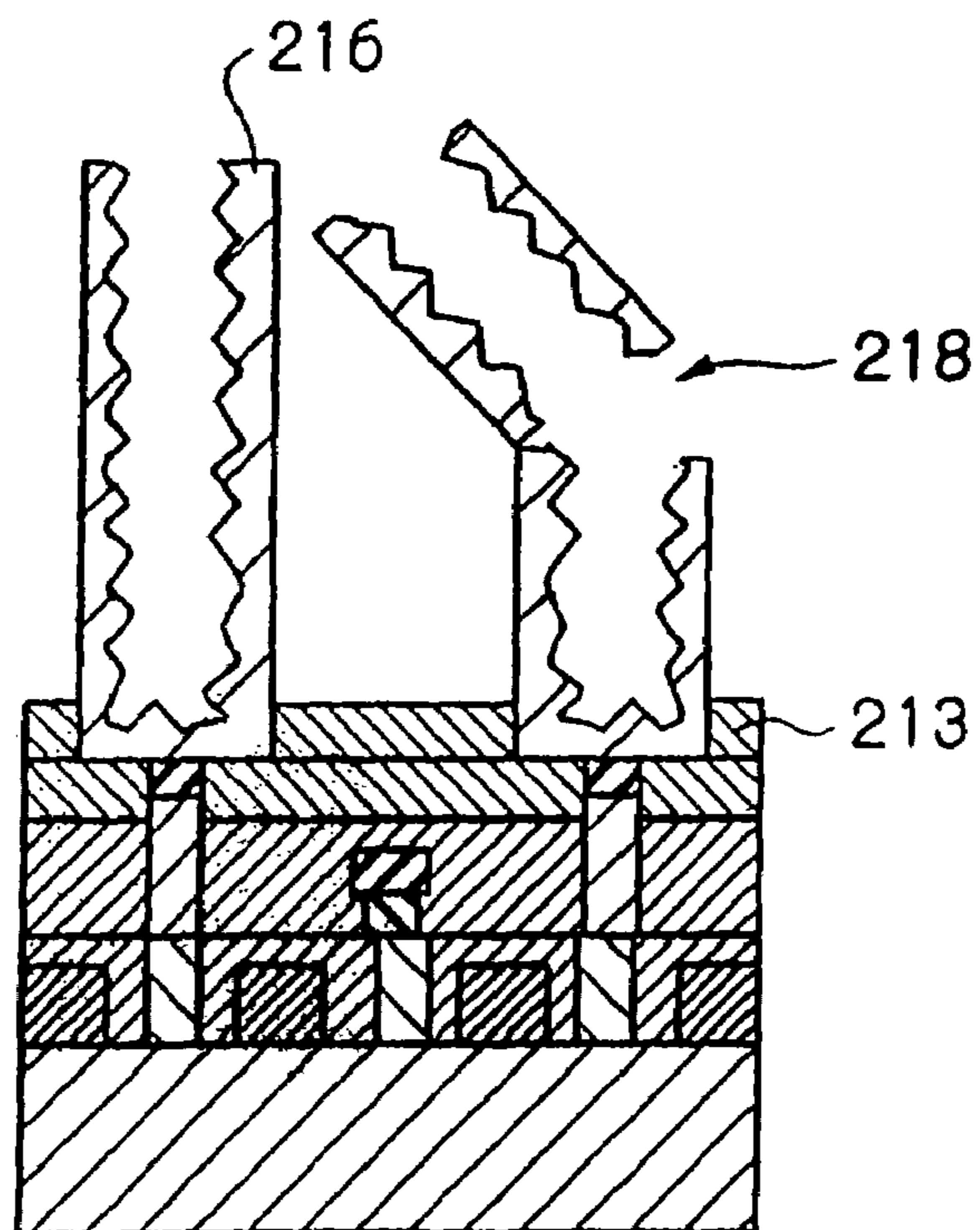
FIG. 2G (PRIOR ART)
