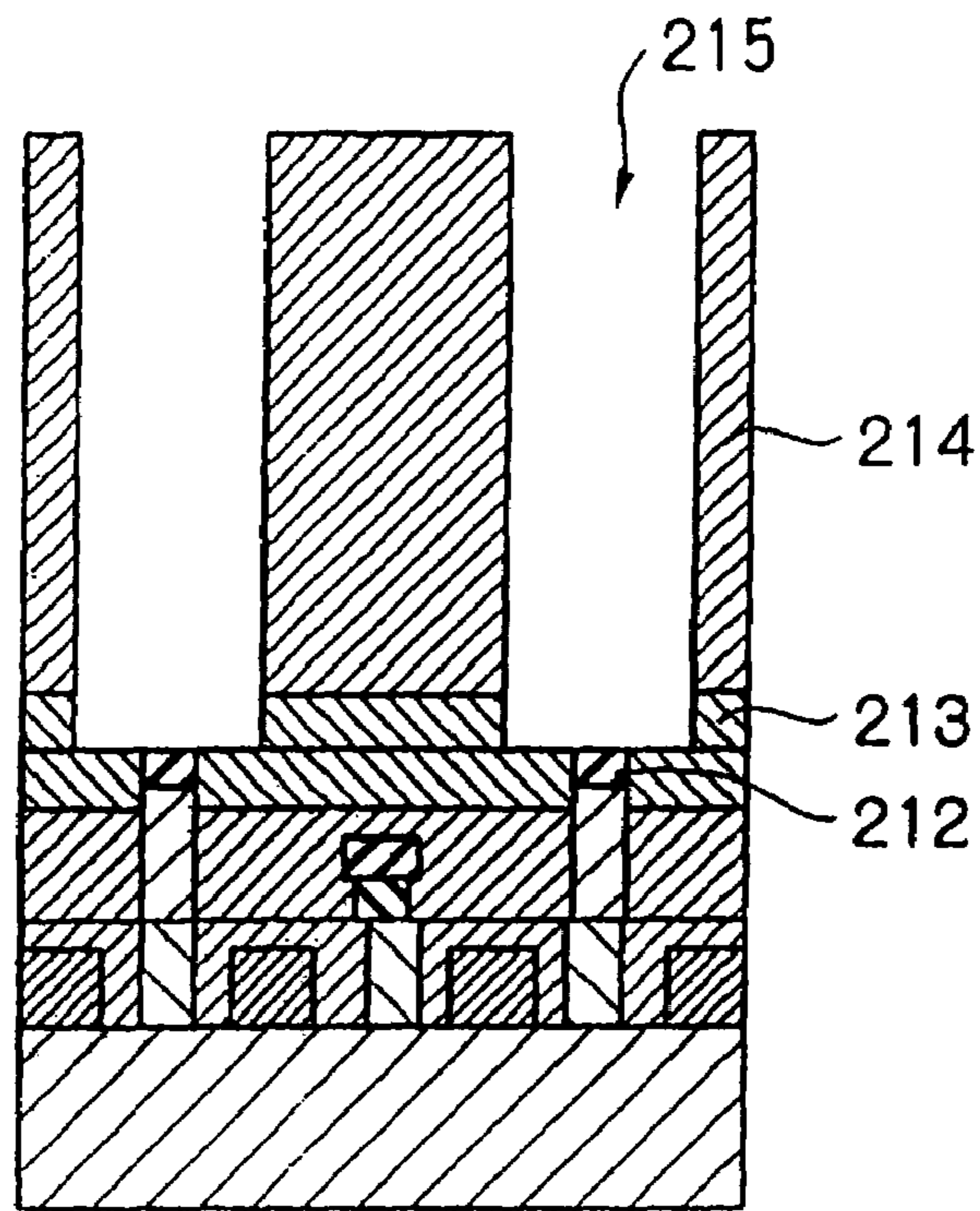
FIG. 2D (PRIOR ART)
