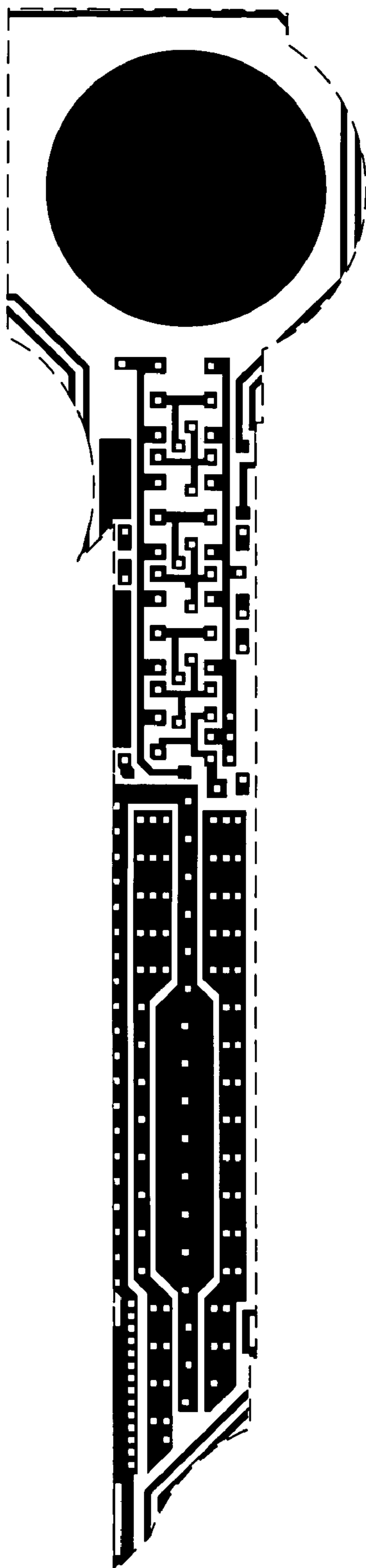
Metal 1 mask
