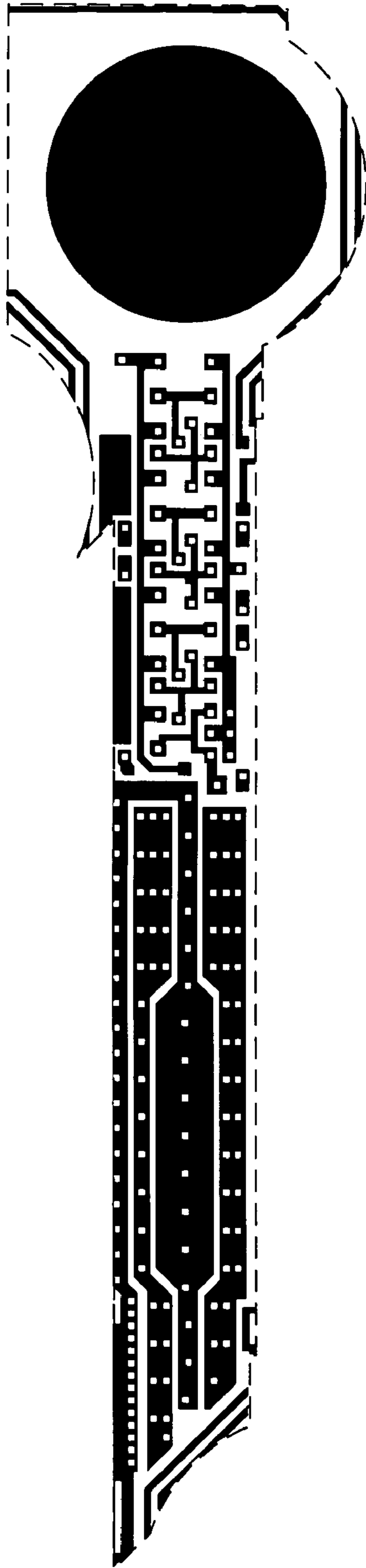
Metal 1 mask
