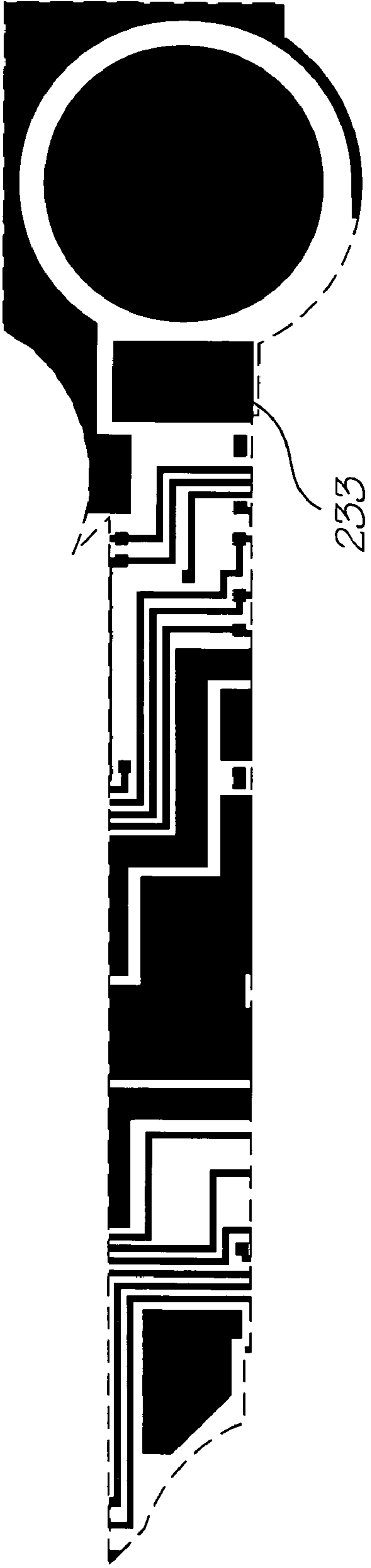
Metal 2 mask
