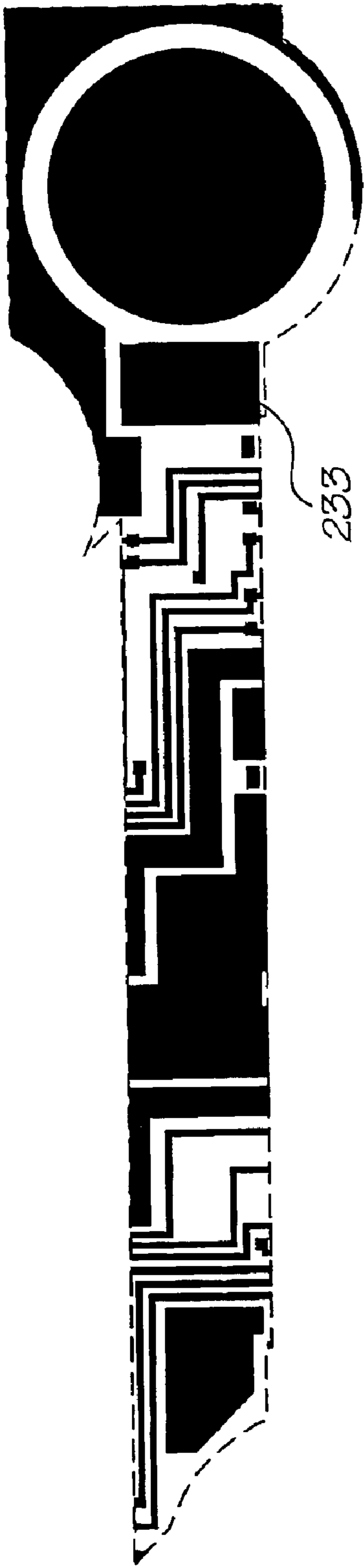
Metal 2 mask
