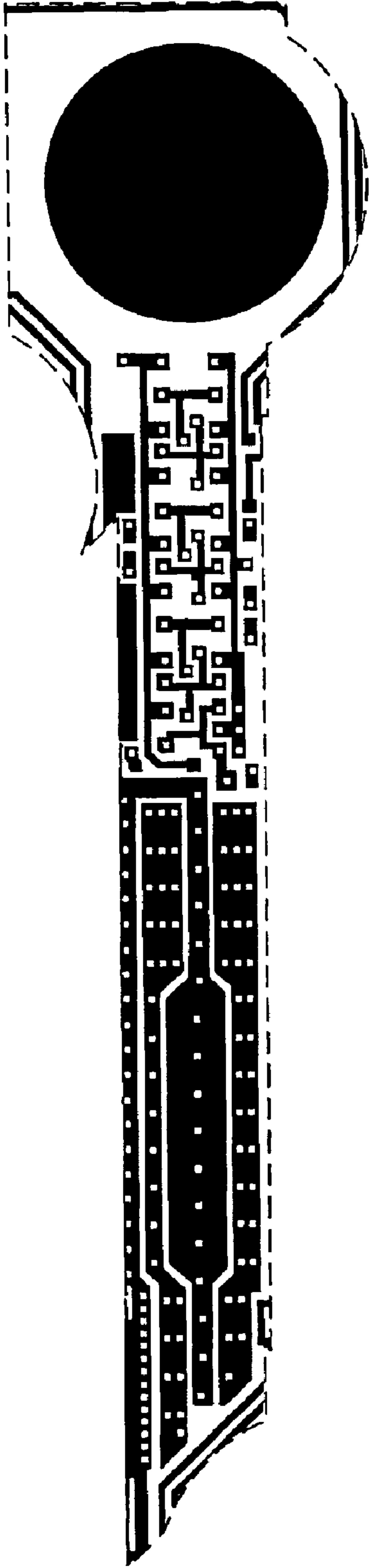
Metal 1 mask
