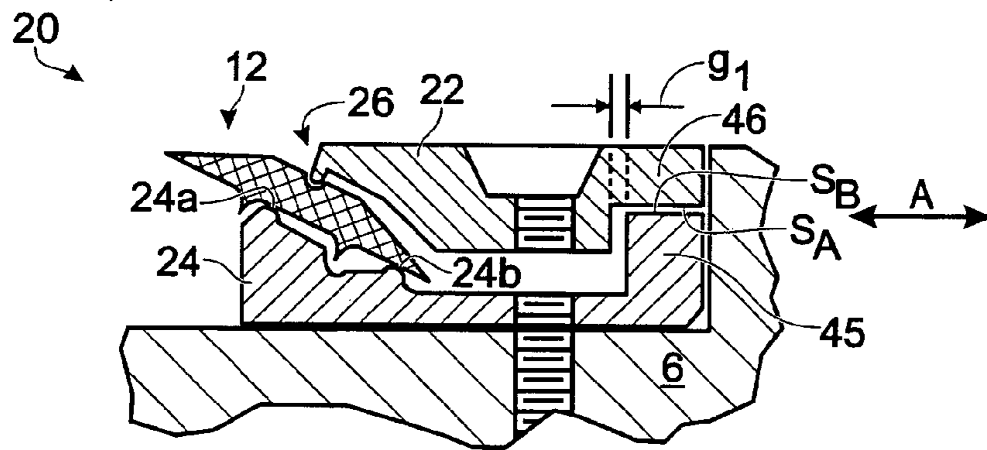
Fig. 5 (PRIOR ART)
