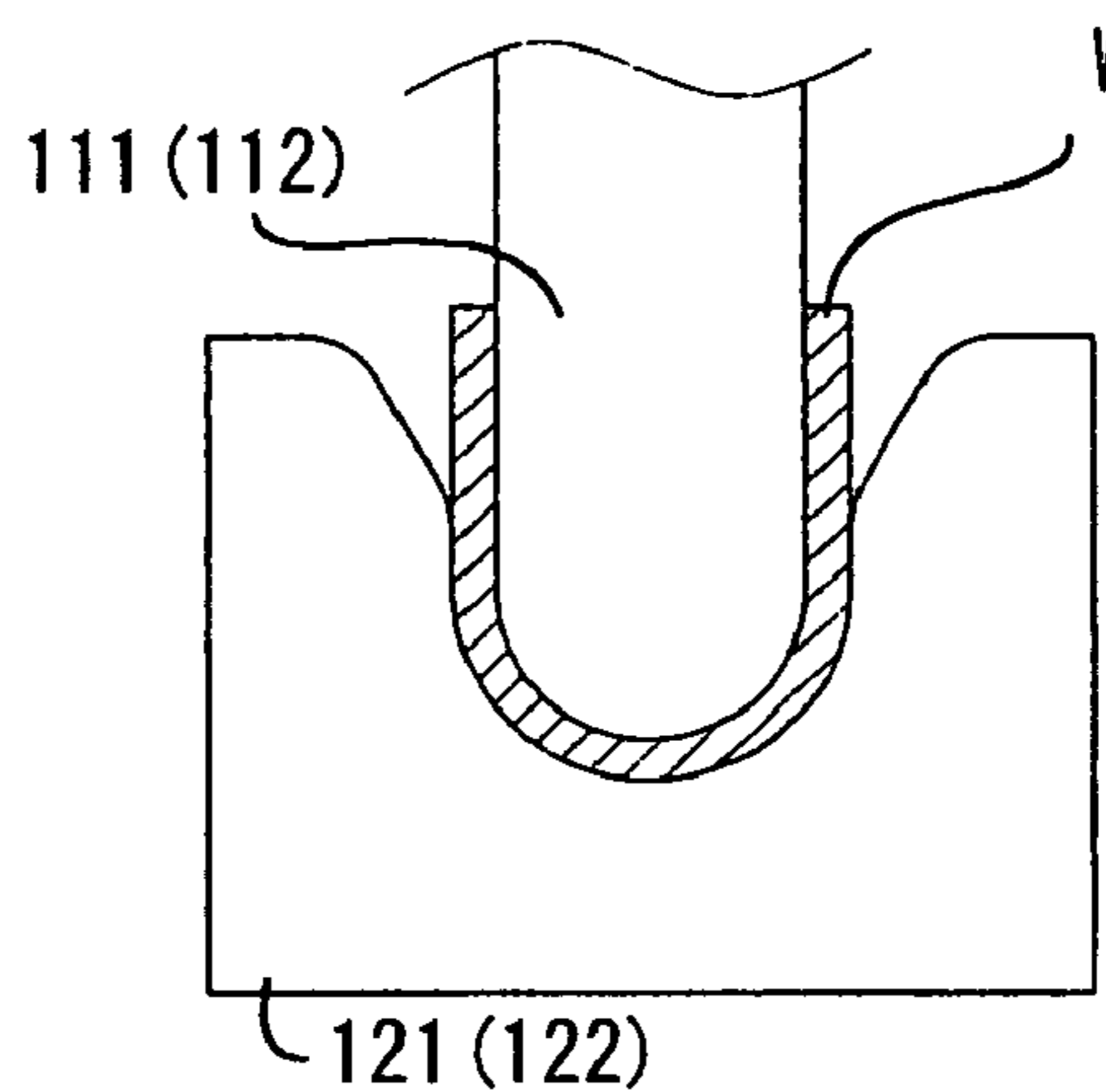
Fig. 1c PRIOR ART
