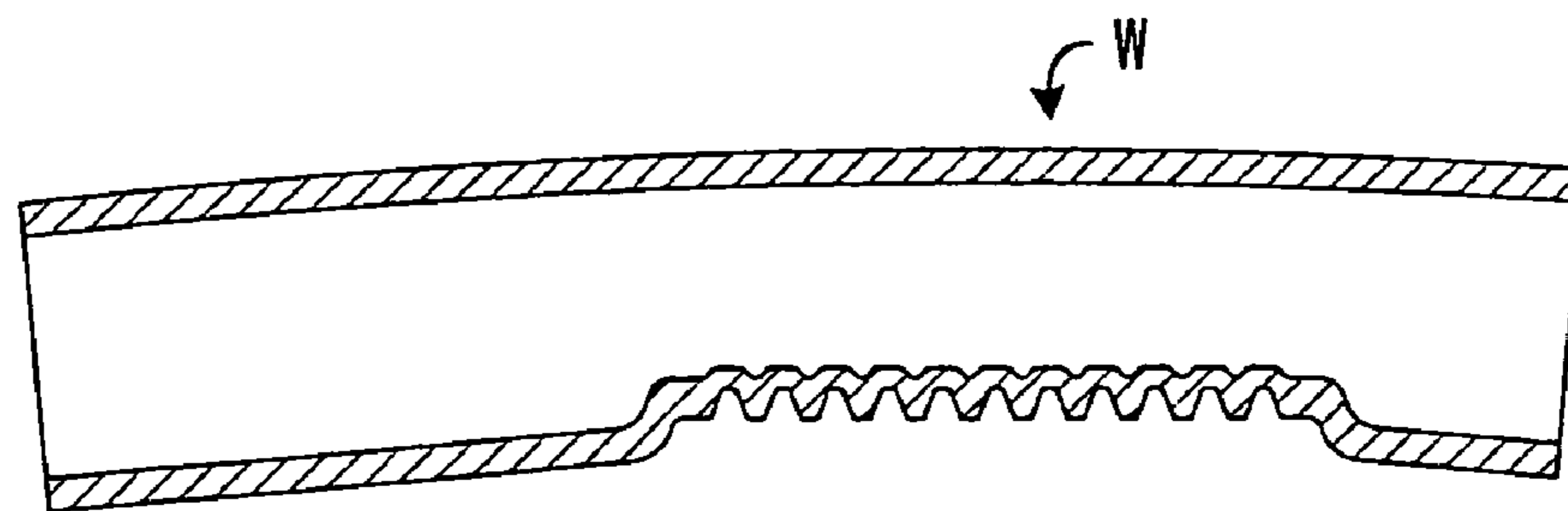
Fig. 5 PRIOR ART
