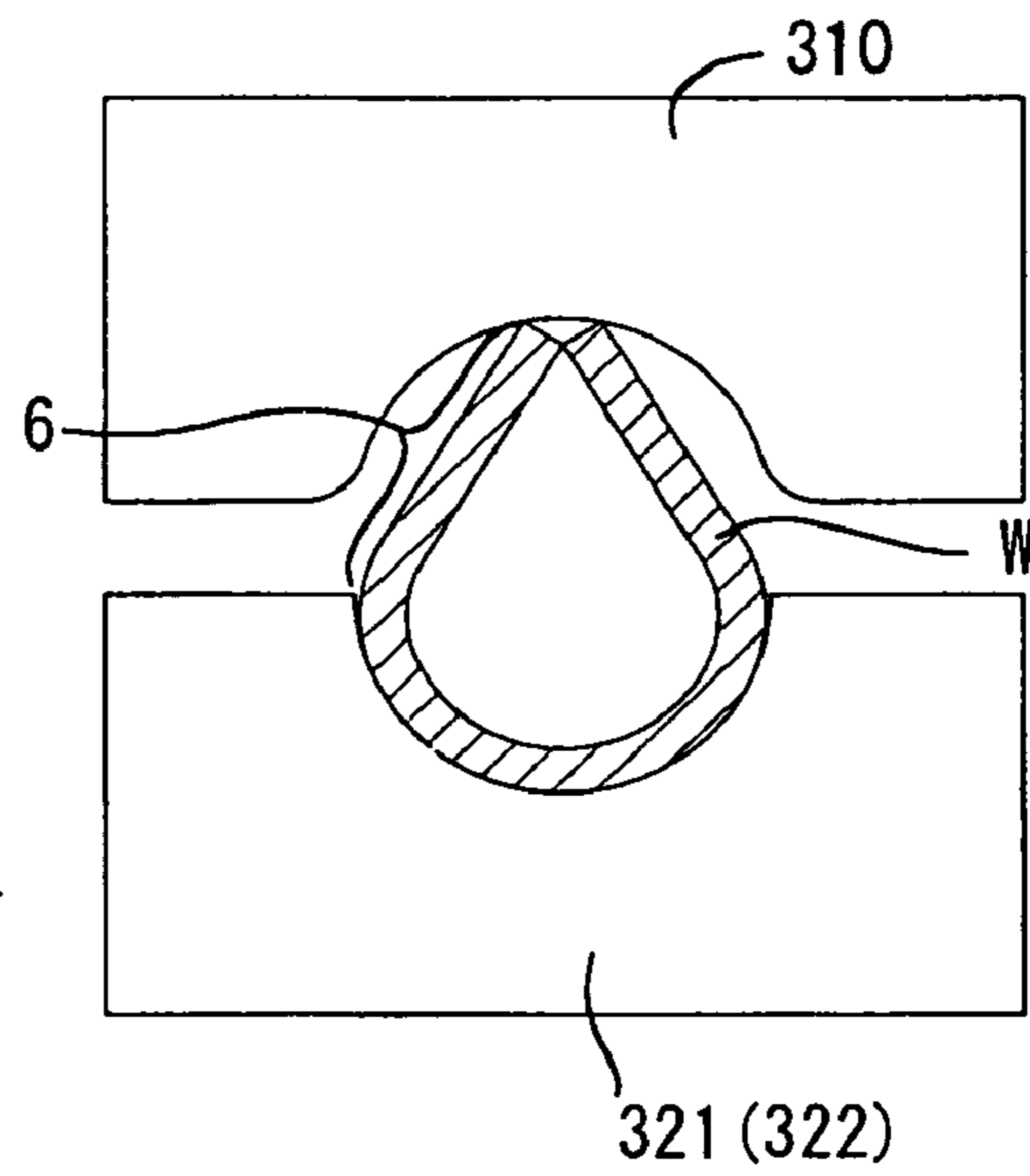
Fig.8c PRIOR ART
