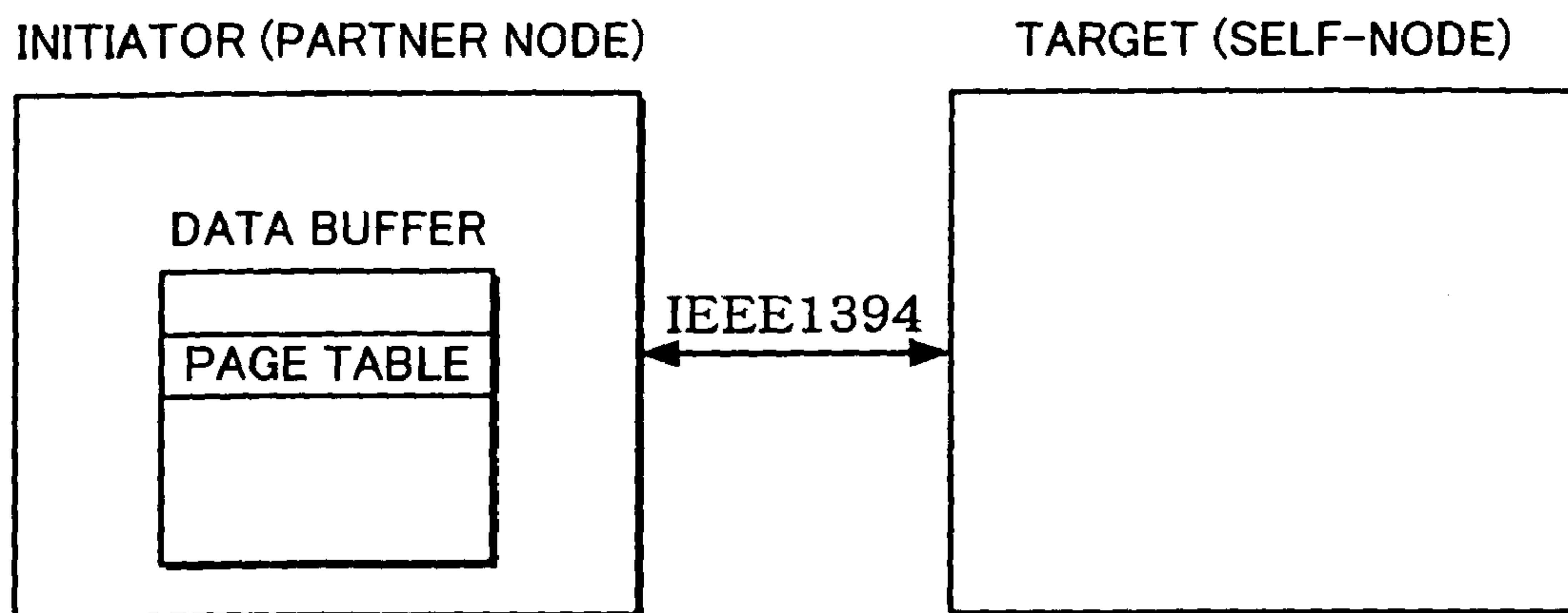
FIG. 5B PAGE TABLE IS PRESENT
