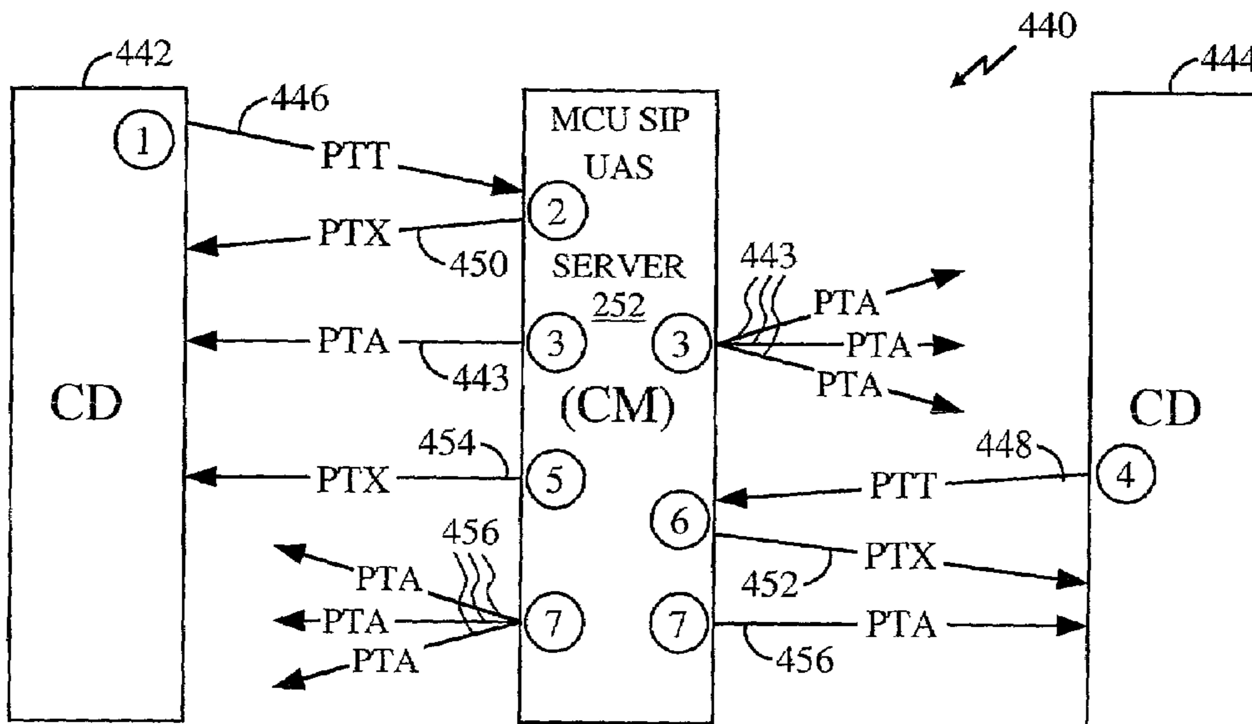
MEDIA SIGNALING MESSAGE SEQUENCE (PRIORITY ARBITRATION)
