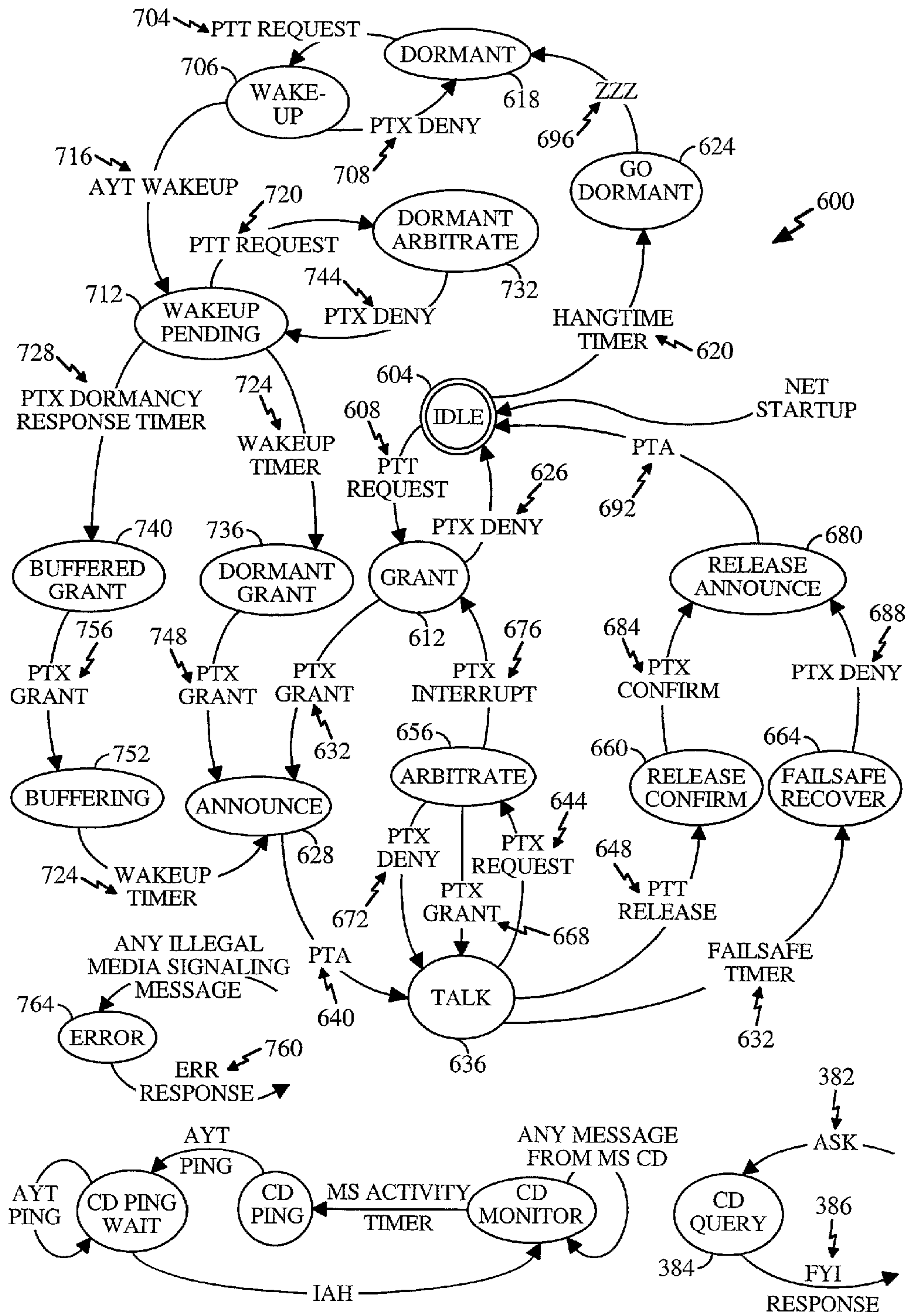
FIG. 15 MEDIA SIGNALING STATE DIAGRAM
