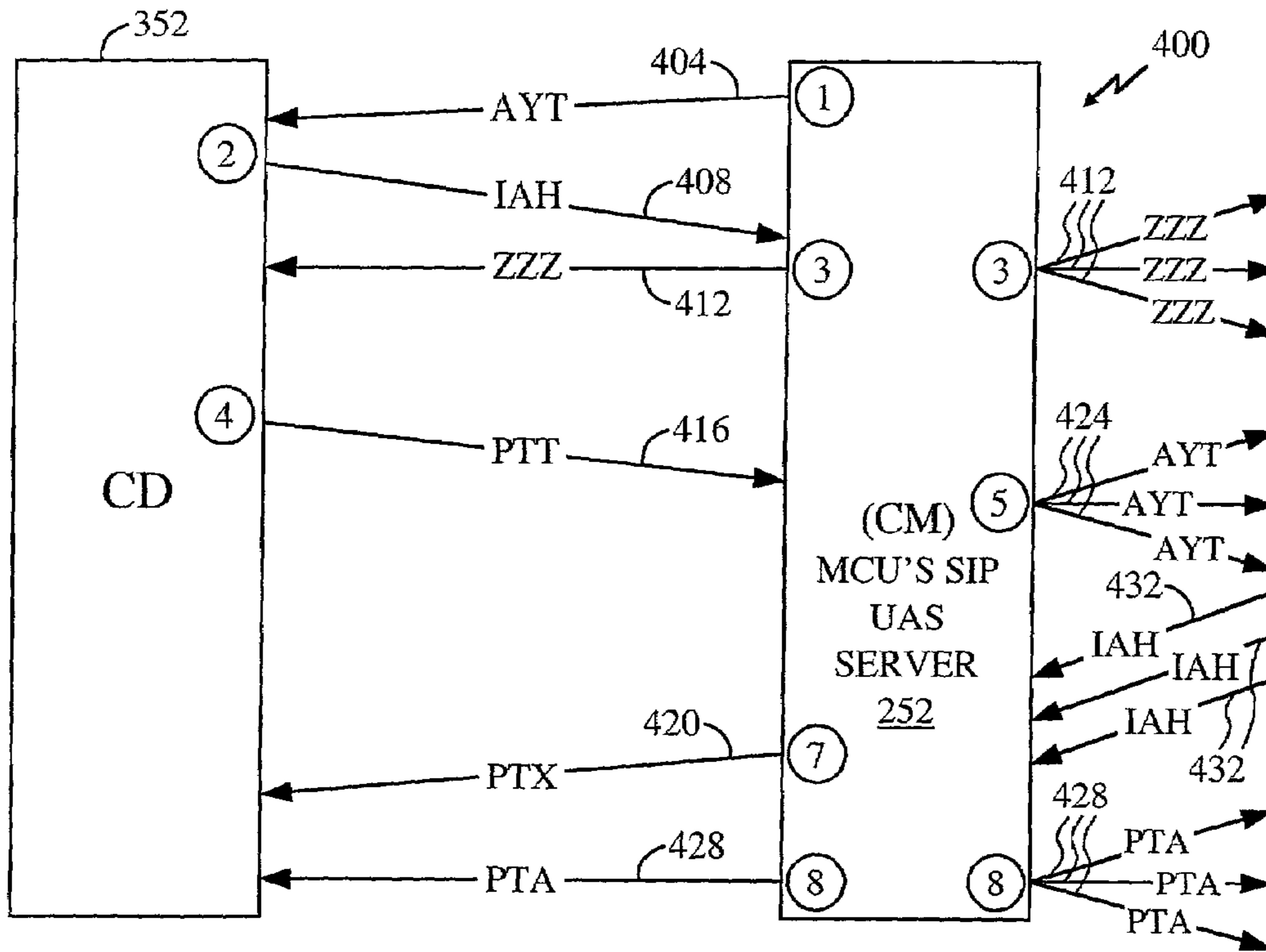
MEDIA SIGNALING MESSAGE SEQUENCE (DORMANCY)
