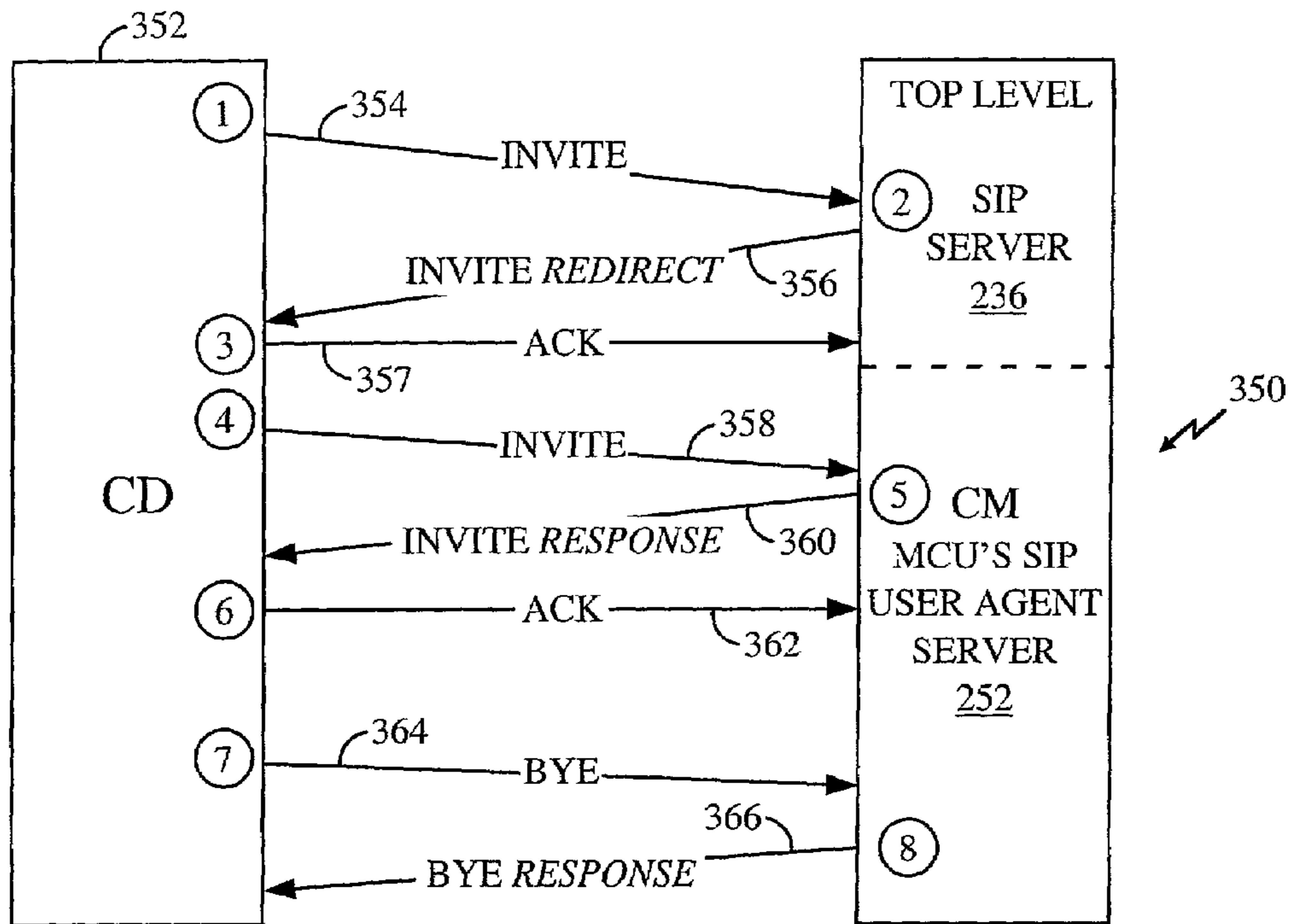
FIG. 11 SIP CALL SIGNALING
