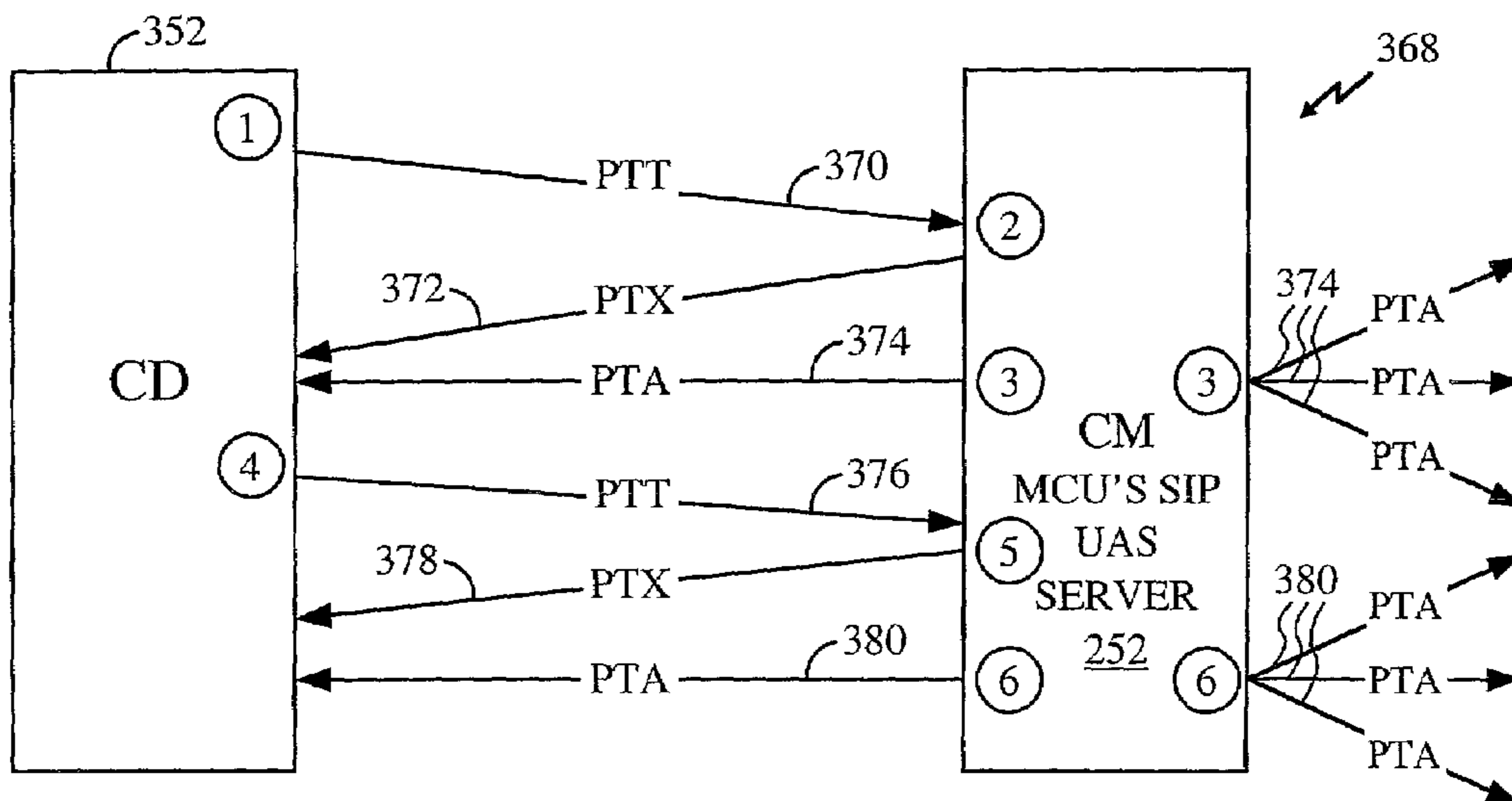
FIG. 12 MEDIA SIGNALING MESSAGE SEQUENCE (PTT)
