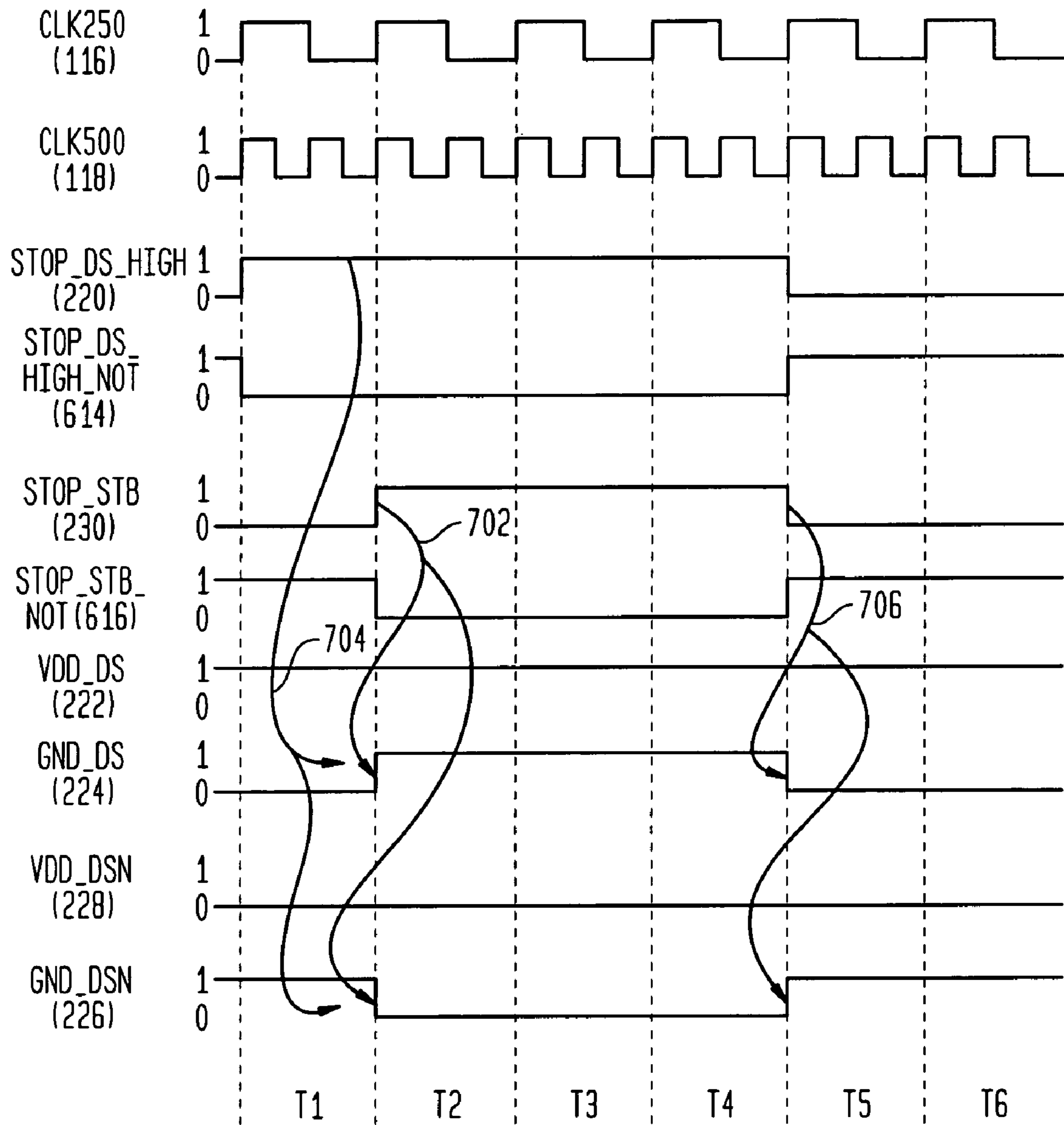
700 DIFFERENTIAL DATA STROBE CONTROL TIMING RELATIONSHIPS
