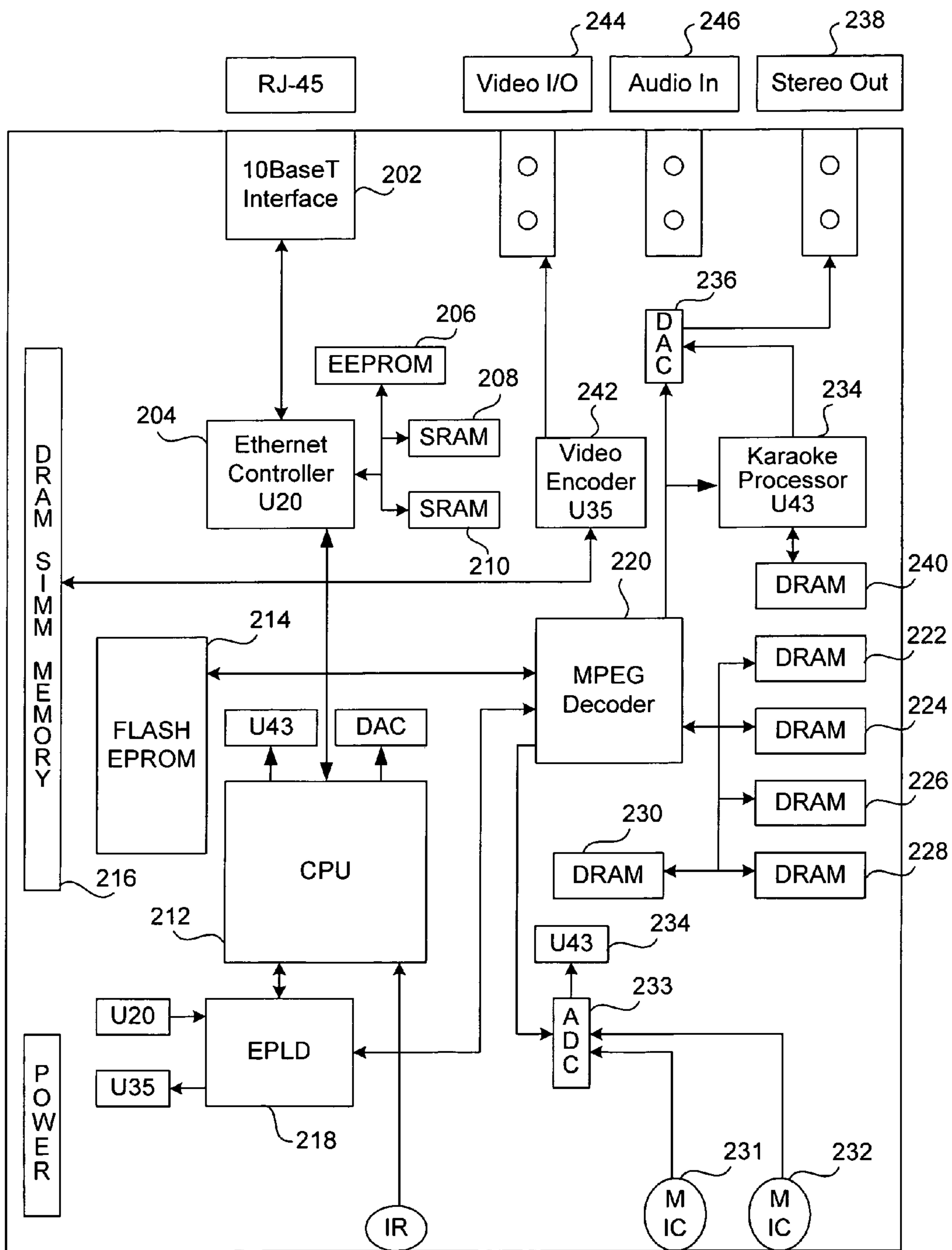
NEVCO VOD/KTV Set-top Box Board Layout
