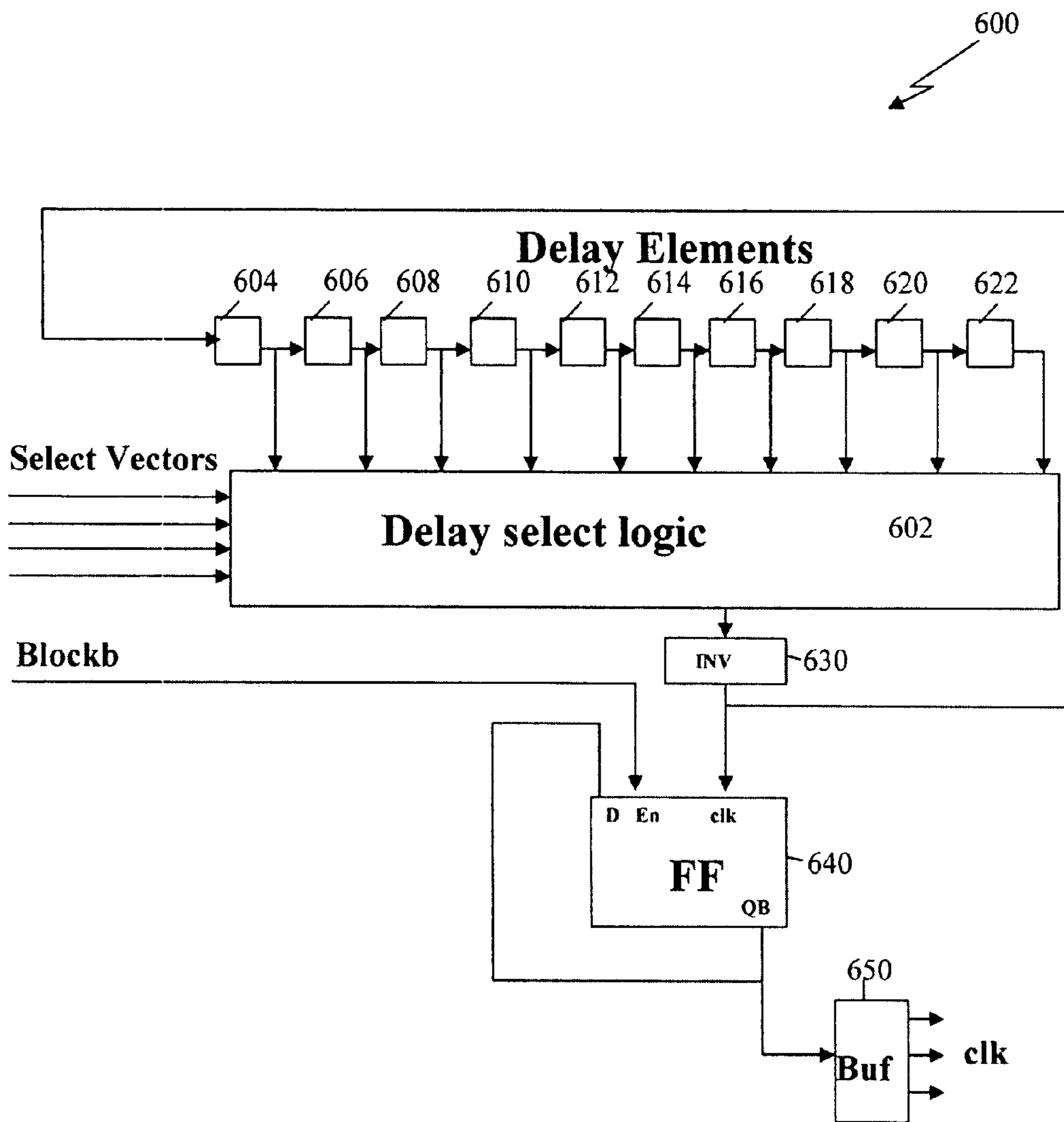
Fig 6 - Adjustable Ring Oscillator
