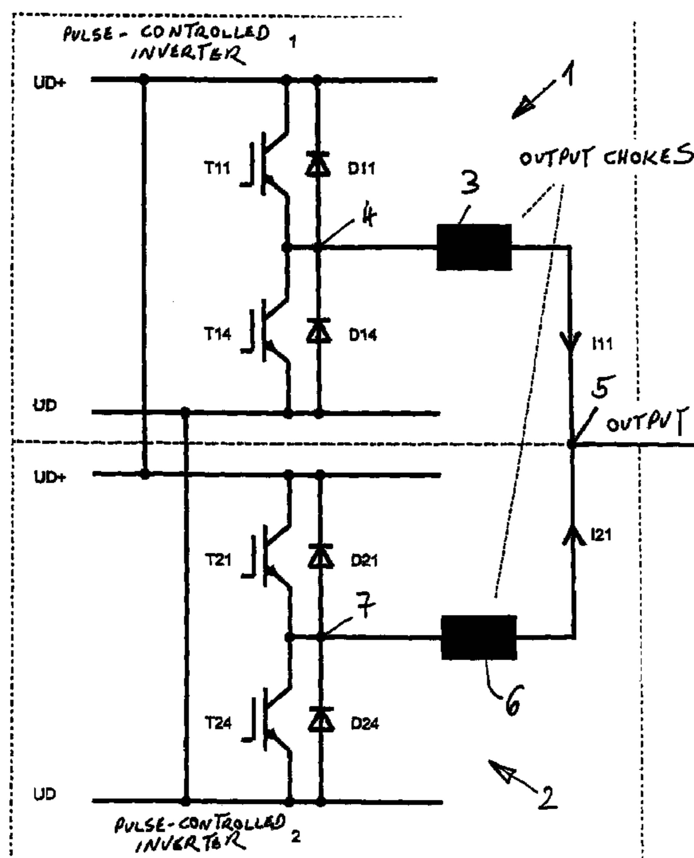
CIRCUIT DIAGRAM PROVIDING AN EXAMPLE OF A PARALLEL-CONNECTED CIRCUIT FOR TWO SINGLE-PHASE PULSE-CONTROLLED INVERTERS WITH IGBTs, FREE-WHEELING DIODES, AND OUTPUT CHOKES
