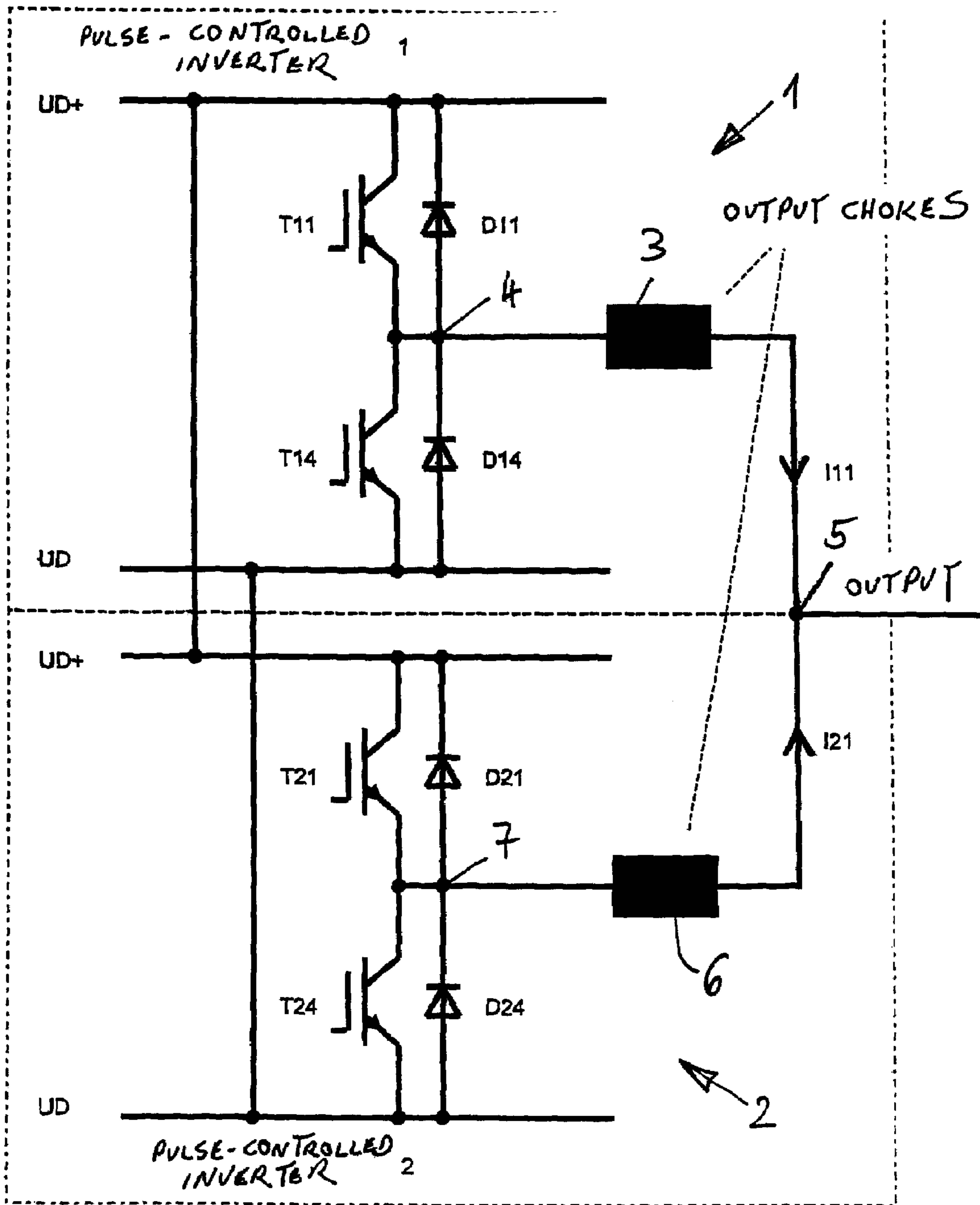
FIG. 1 CIRCUIT DIAGRAM PROVIDING AN EXAMPLE OF A PARALLEL-CONNECTED CIRCUIT FOR TWO SINGLE-PHASE PULSE-CONTROLLED INVERTERS WITH IGBTs, FREE-WHEELING DIODES, AND OUTPUT CHOKES
