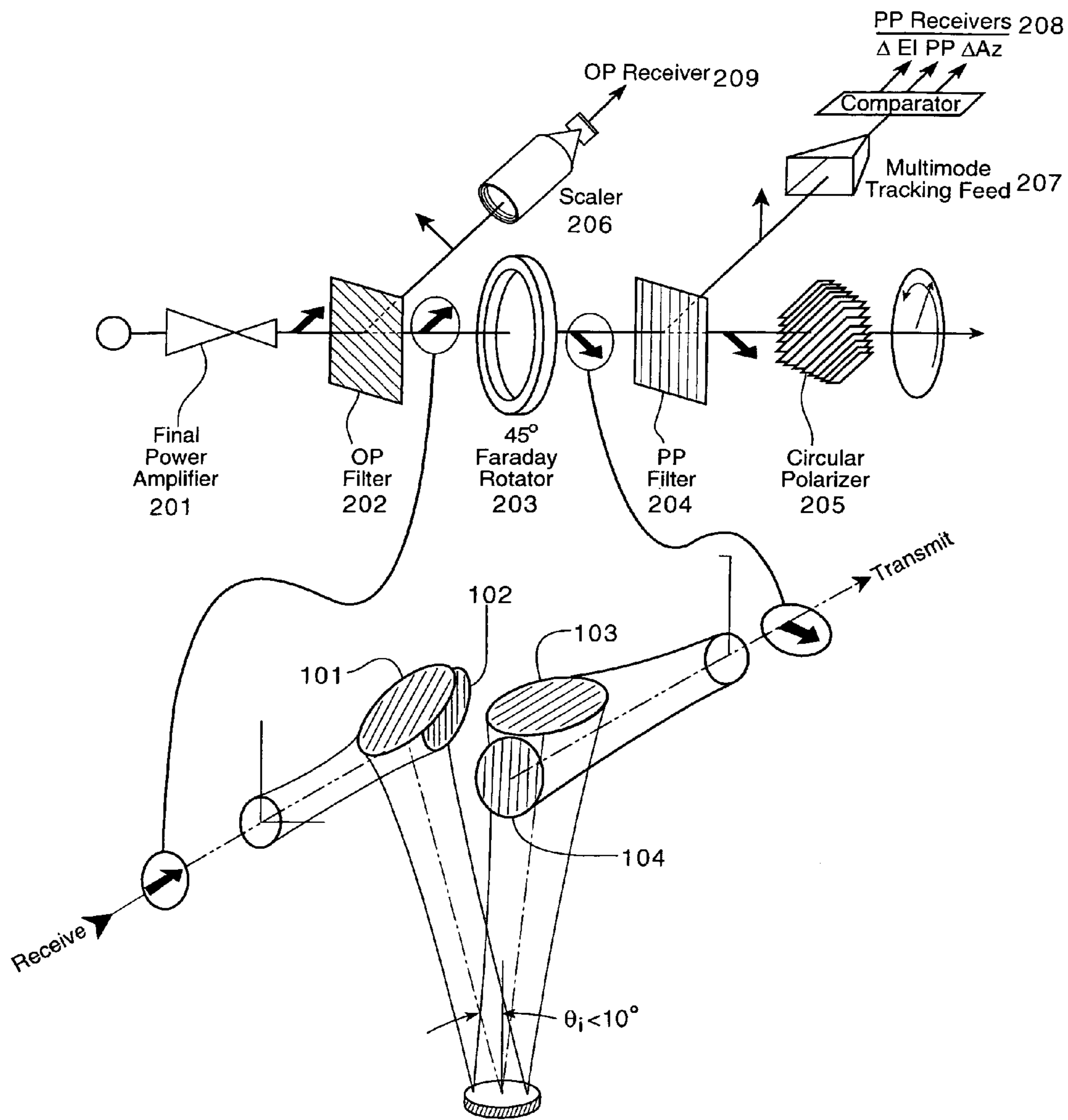
Fig. 2 BWG System Schematic
