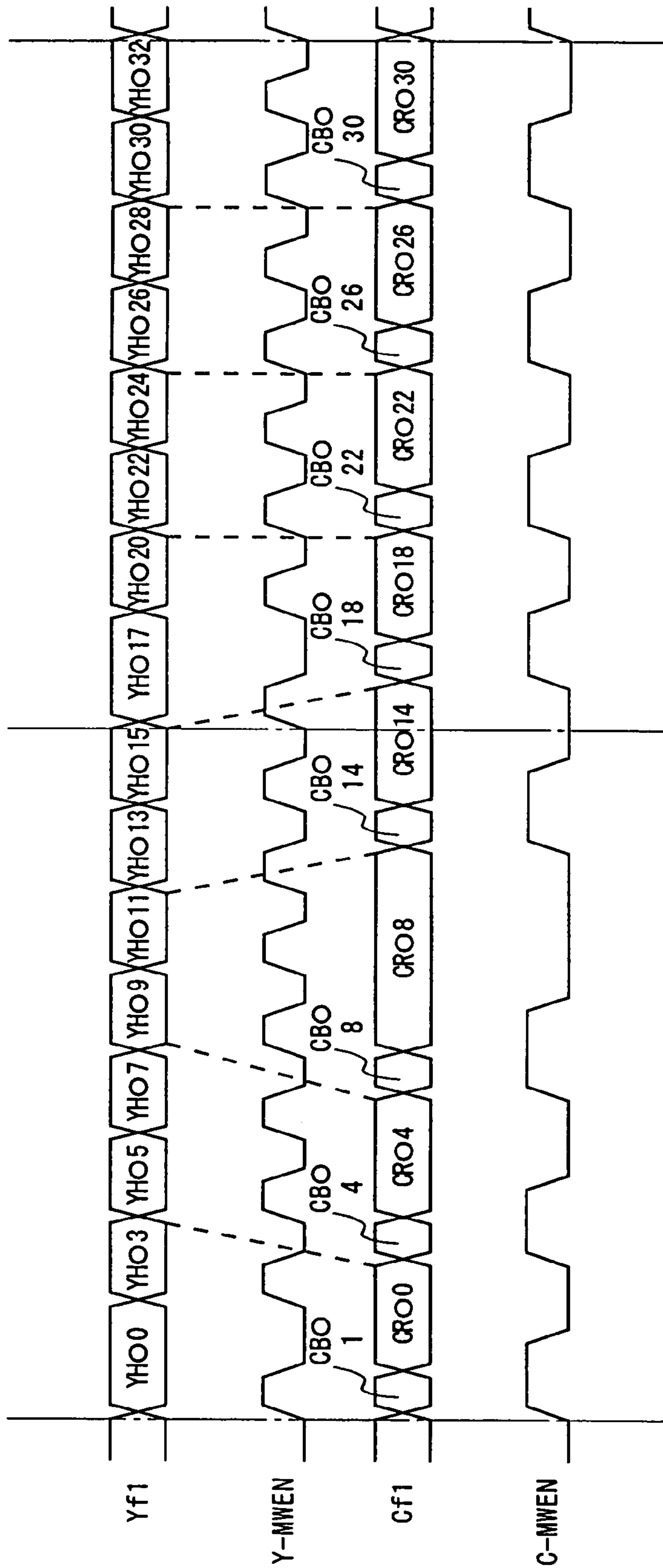
OUTPUT TIMING OF Y-, C-HORIZONTAL FILTERS
