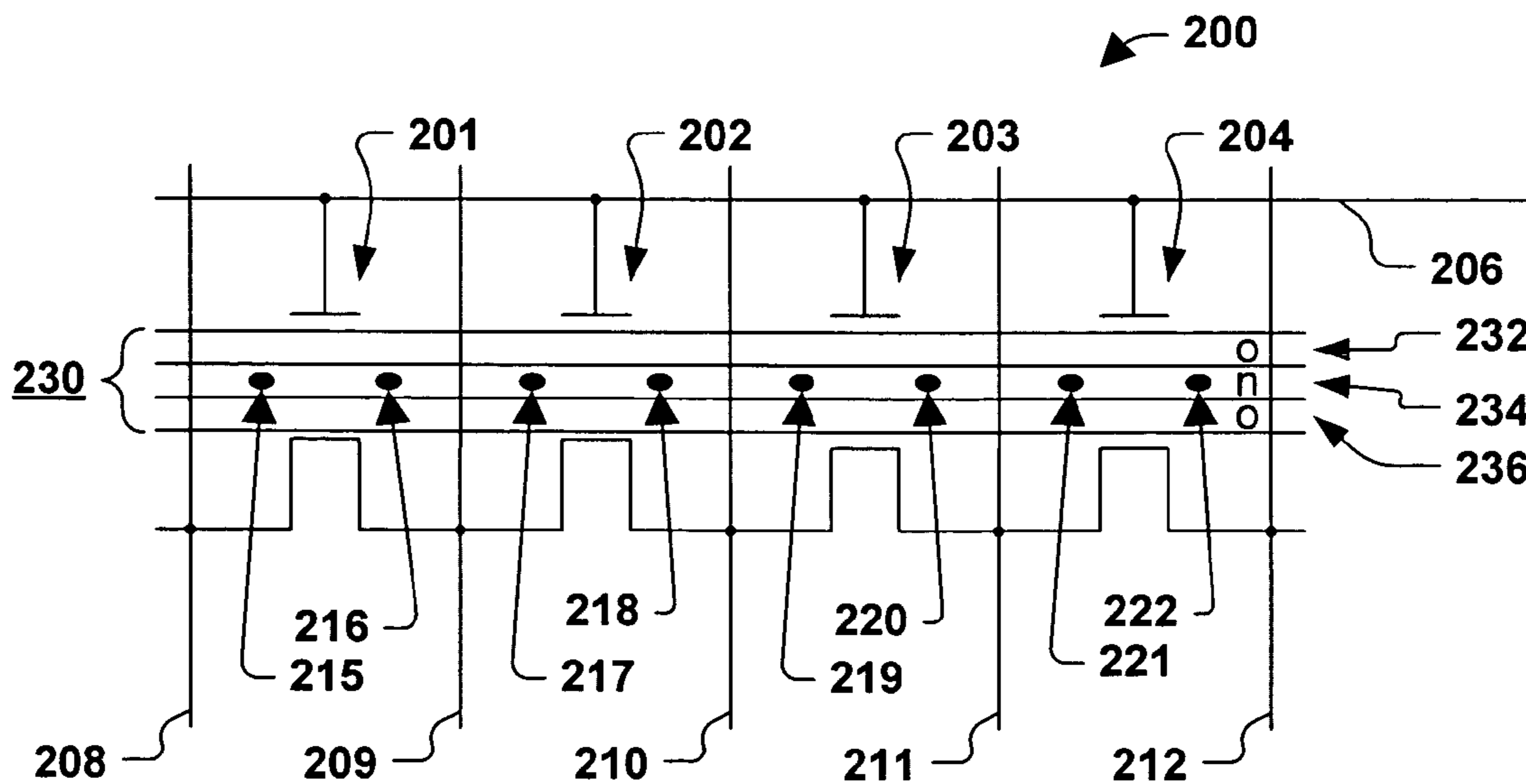
Fig. 2 (PRIOR ART)
