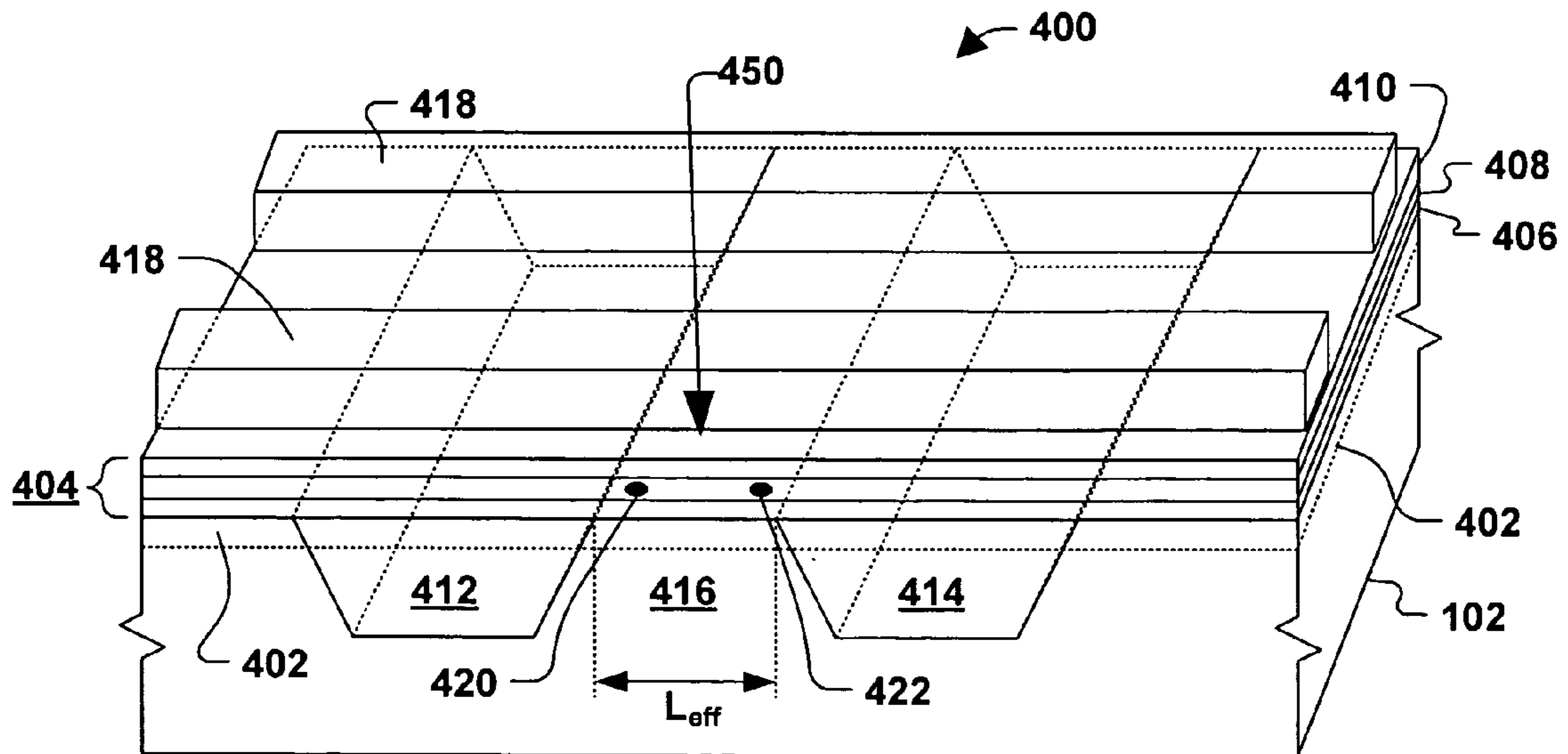
Fig. 4 (PRIOR ART)
