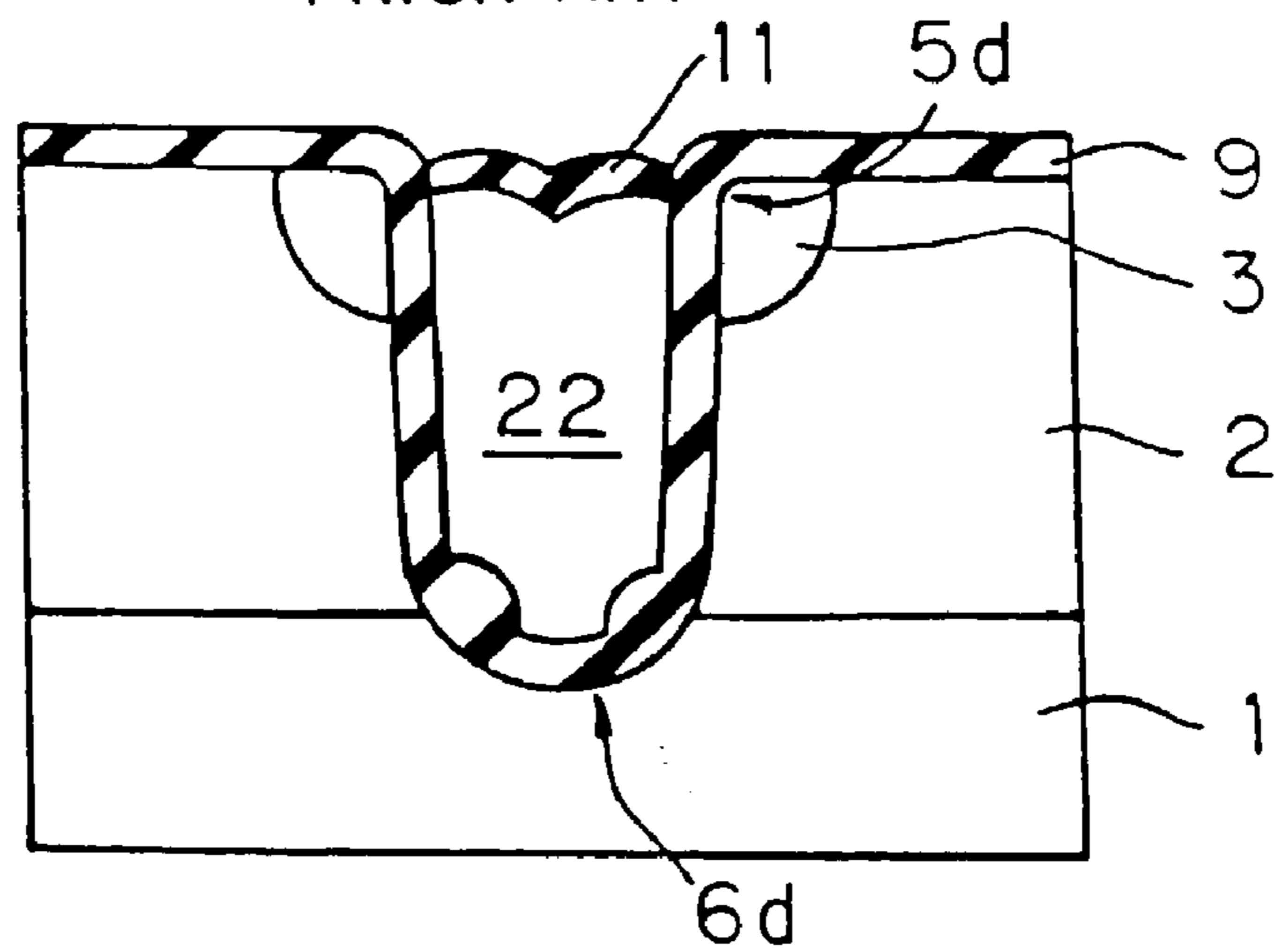
FIG. 70 PRIOR ART
