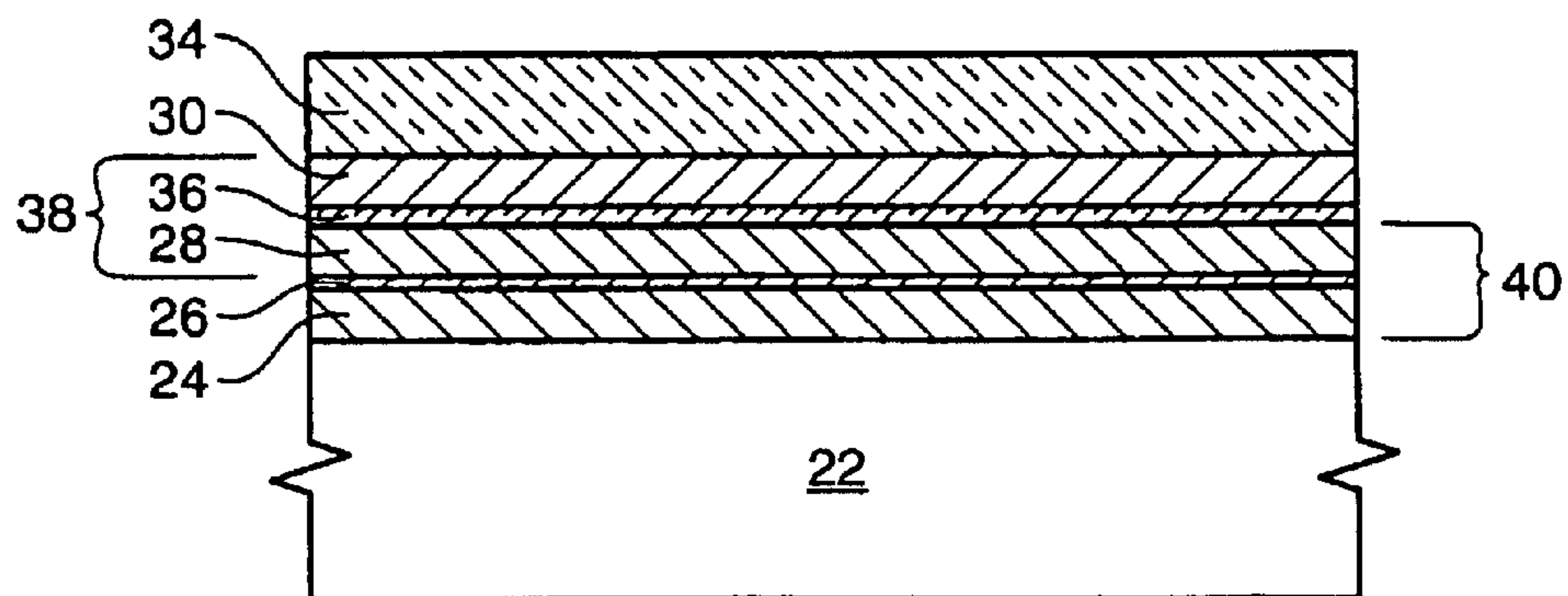
FIG. 3 (PRIOR ART)
