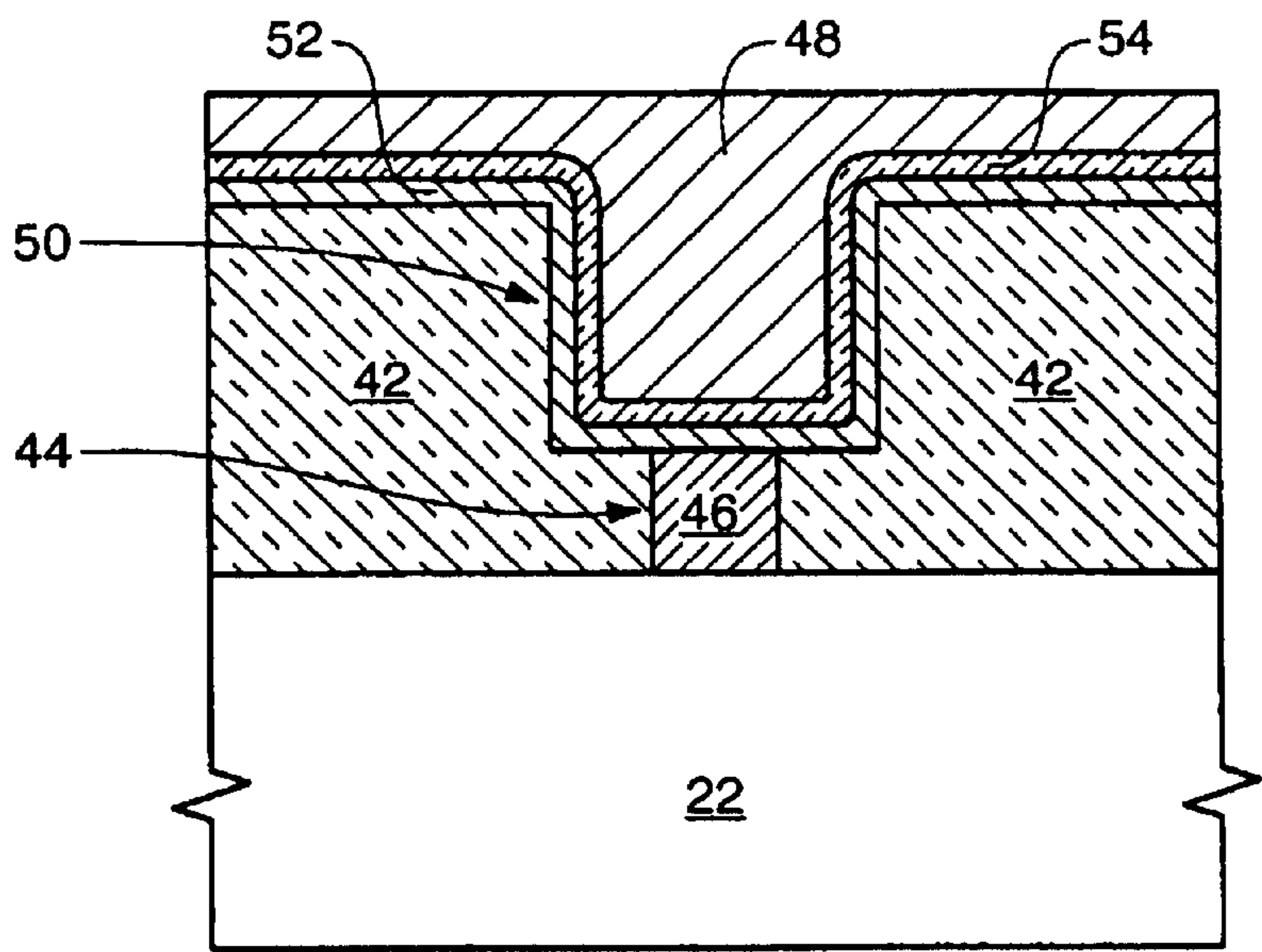
FIG. 8 (PRIOR ART)
