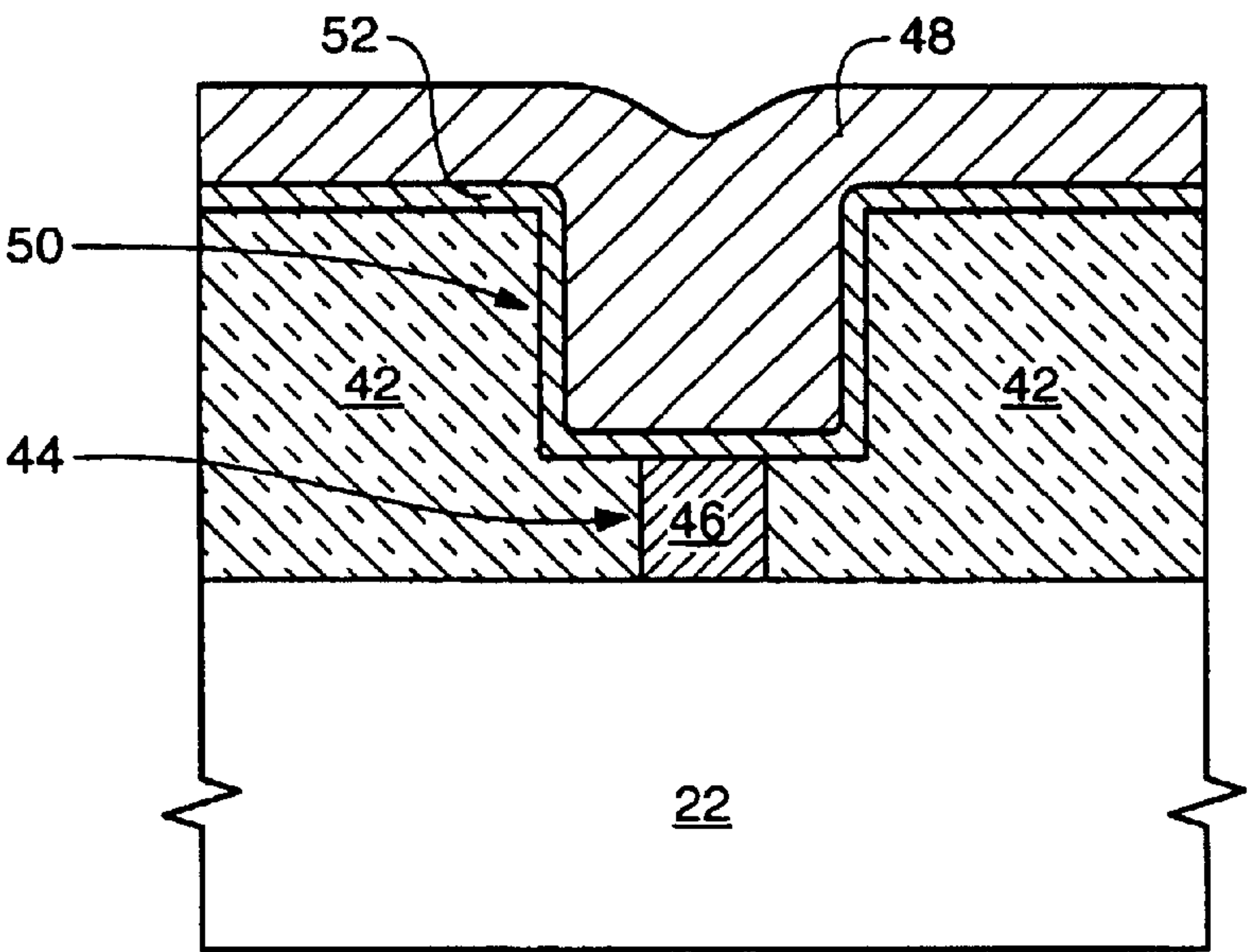
FIG. 7 (PRIOR ART)
