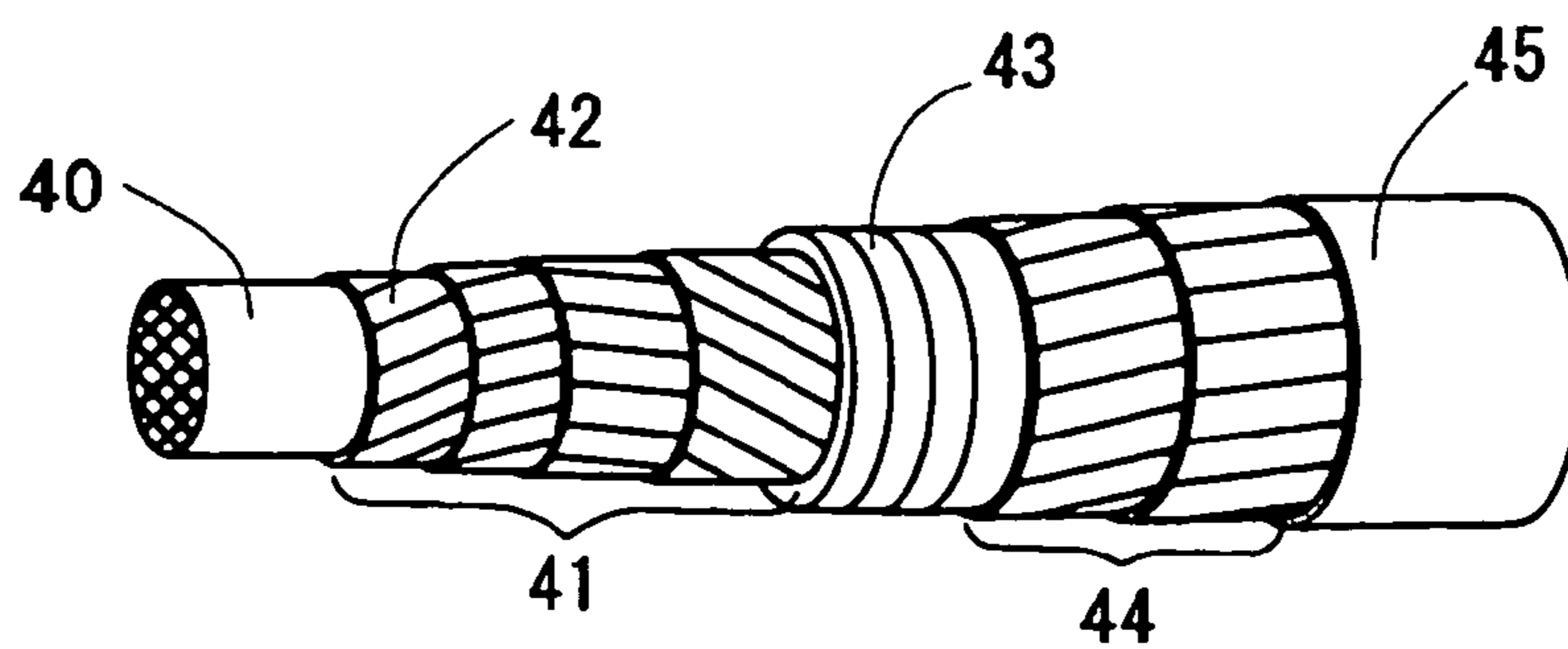
FIG.6 PRIOR ART
