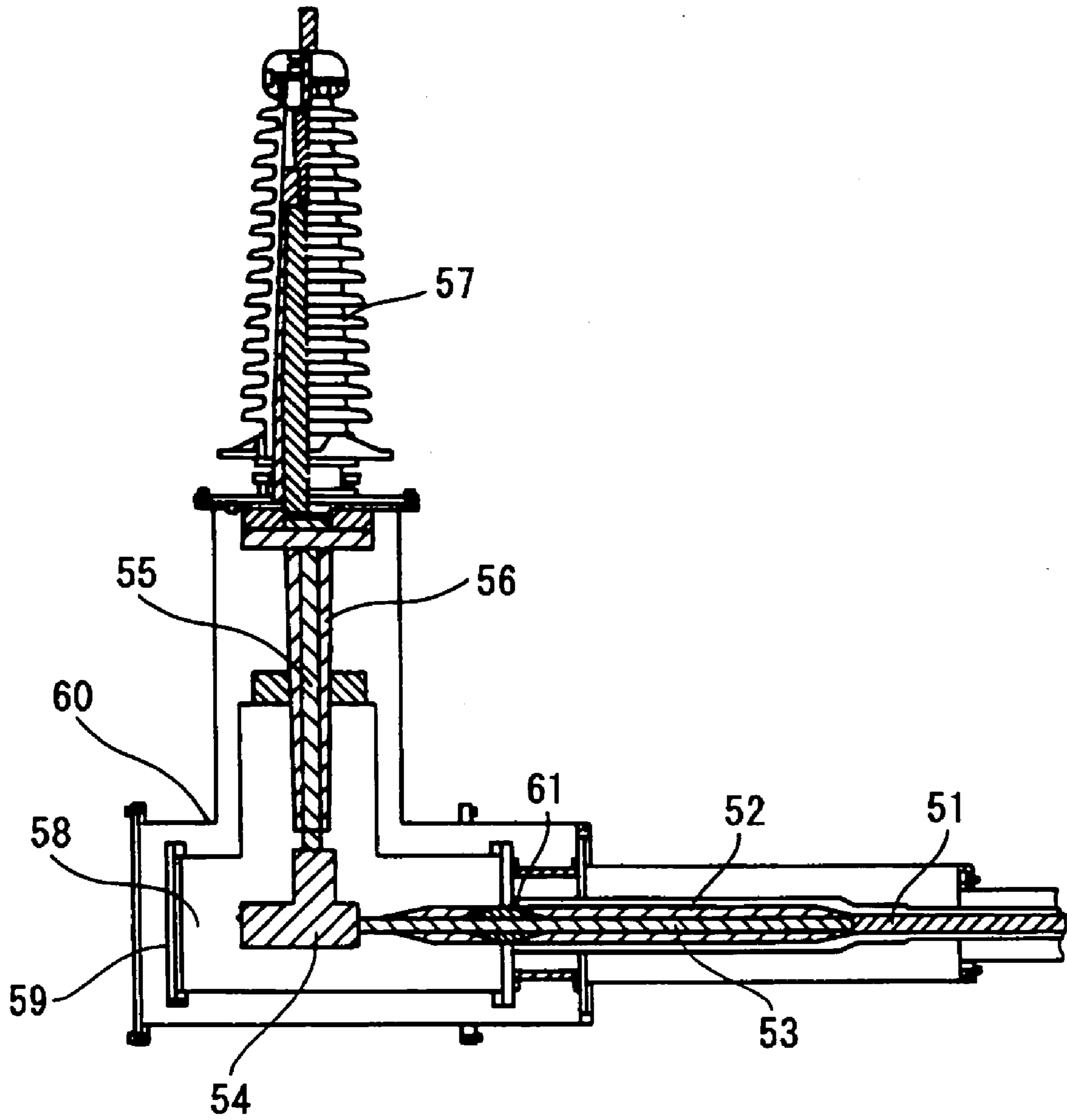
FIG. 7 PRIOR ART
