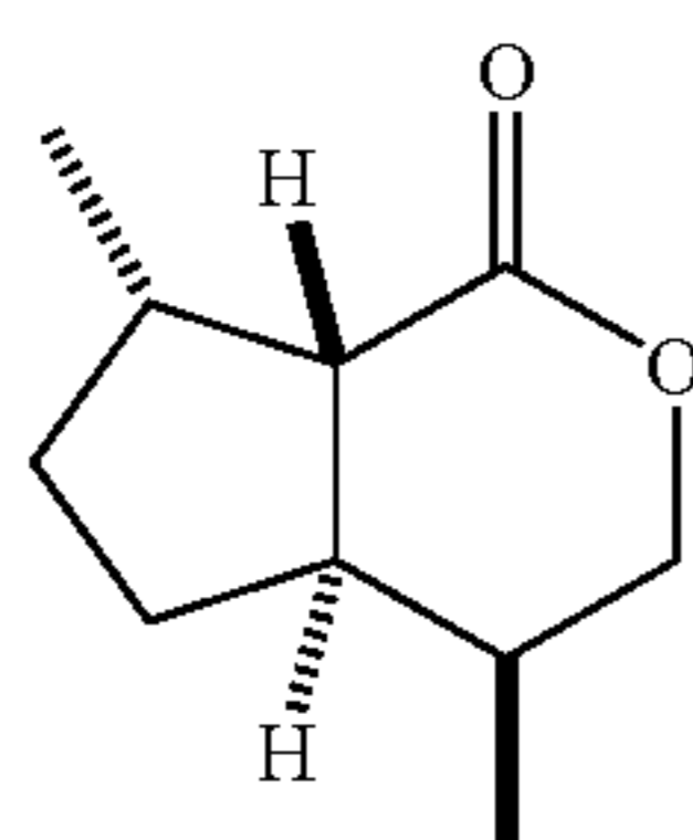
(1S,5S,9S,6R)-5,9-dimethyl-3-oxabicyclo[4.3.0]nonan-2-one
