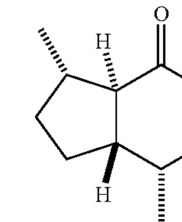
(9S,6S,1R,5R)-5,9-dimethyl-3-oxabicyclo[4.3.0]nonan-2-one
