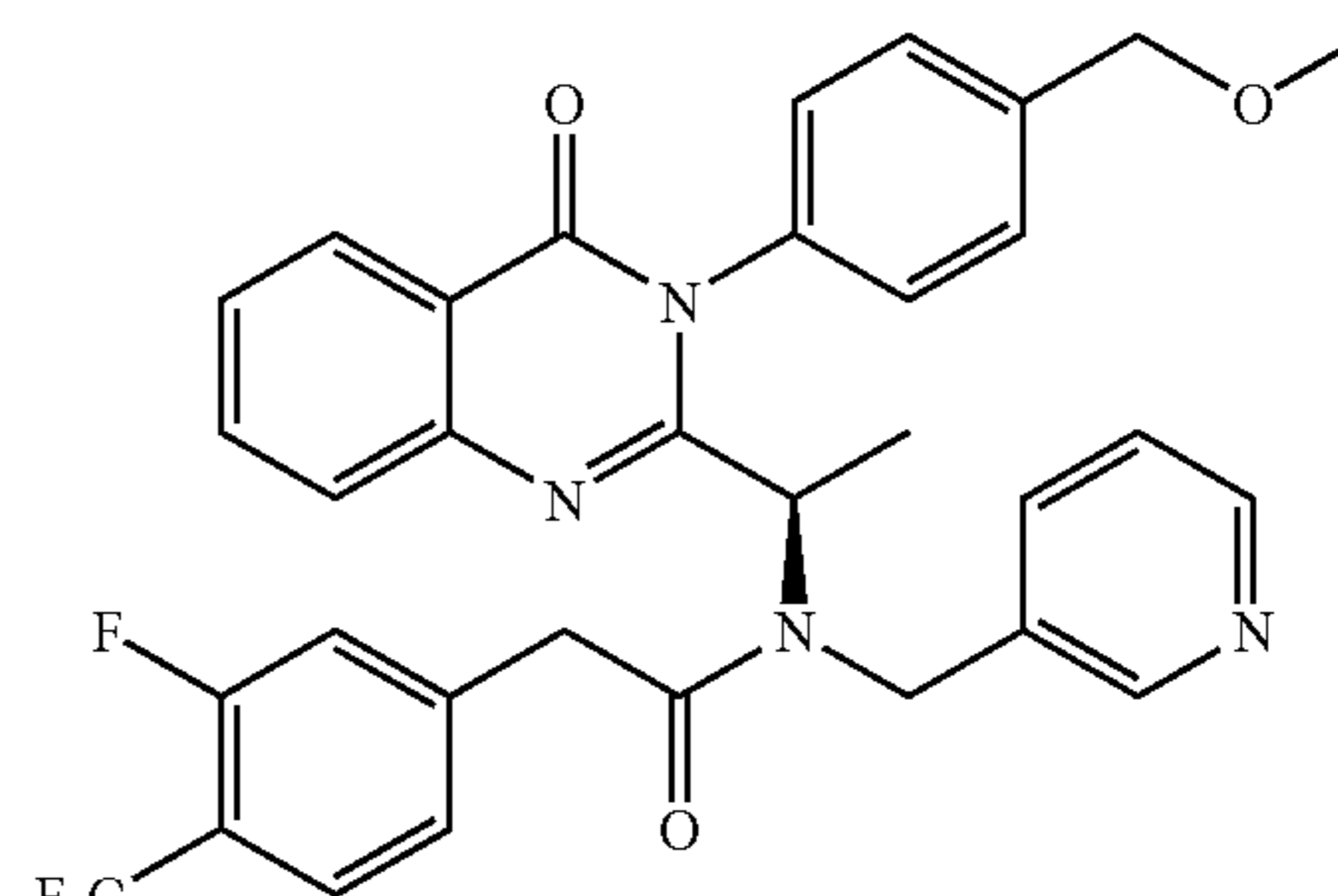
2-(3-Fluoro-4-trifluoromethyl-phenyl)-N-{1-[3-(4-methoxymethyl-phenyl)-4-oxo-3,4-dihydro-quinazolin-2-yl]-ethyl}-N-pyridin-3-ylmethyl-acetamide 3.57
