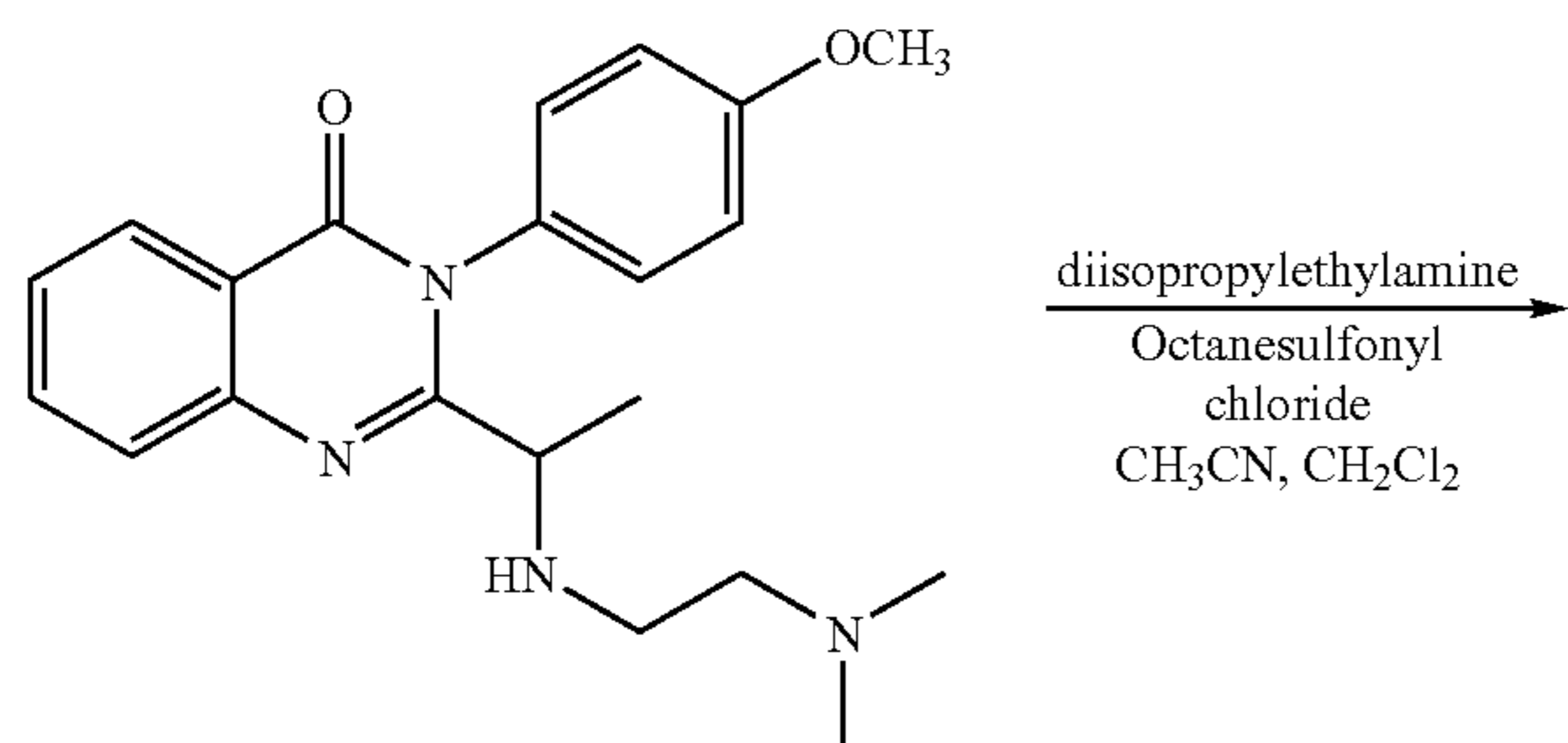
2-[1-(2-Dimethylamino-ethylamino)-ethyl]-3-(4-methoxy-phenyl)-3H-quinazolin-4-one
