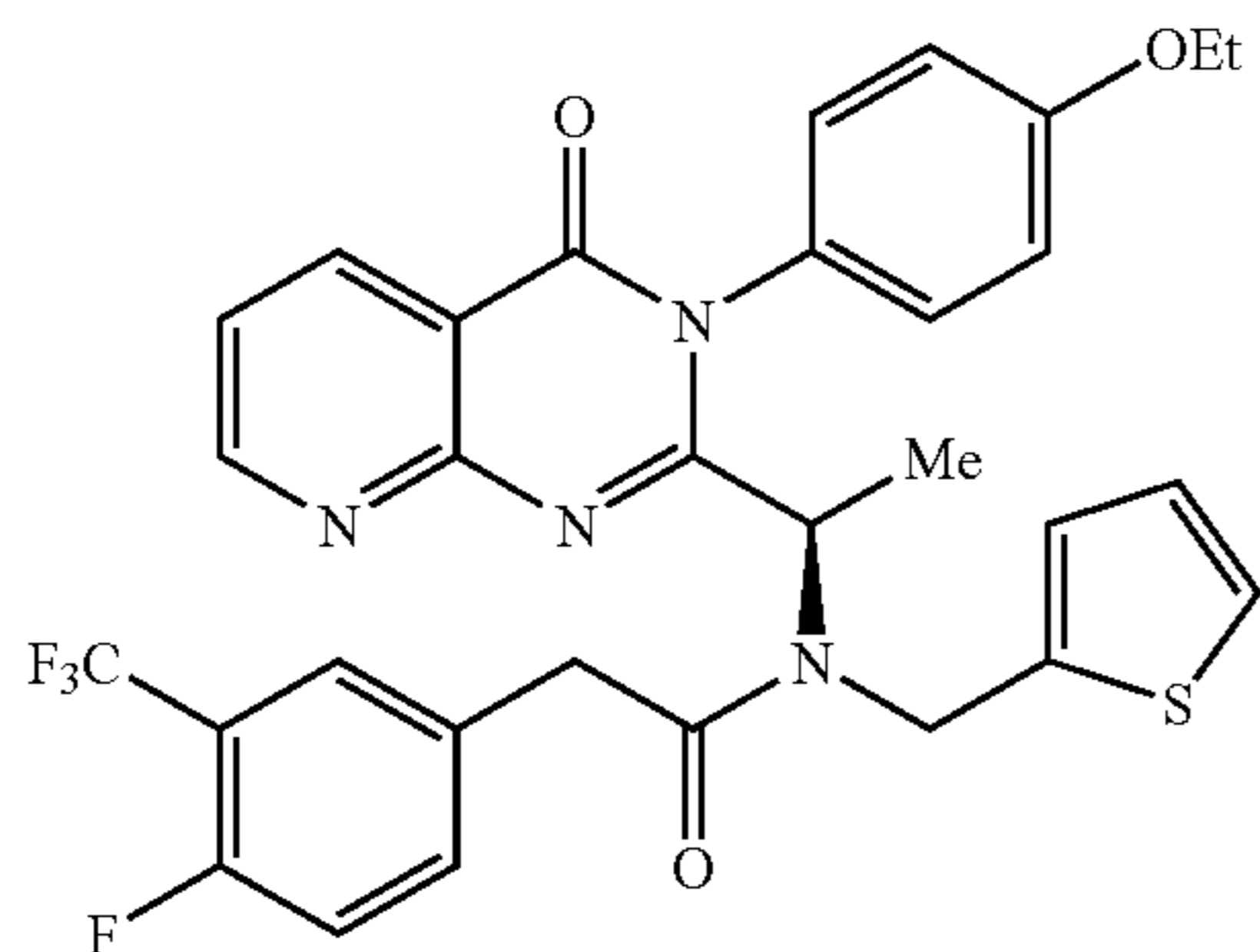
(R)-N-({1-[3-(4-Ethoxy-phenyl)-4-oxo-3,4-dihydro-pyrido[2,3-d]pyrimidin-2-yl]-ethyl}-2-(4-fluoro-3-trifluoromethyl-phenyl)-N-thiophen-2-ylmethyl-acetamide 3.65
