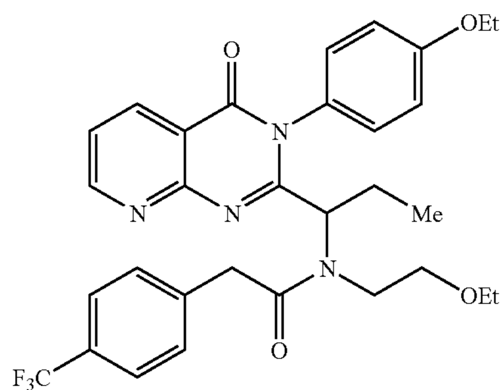
N-(2-Ethoxy-ethyl)-N-{1-[3-(4-ethoxy-phenyl)-4-oxo-3,4-dihydro-pyrido[2,3-o]pyrimidin-2-yl]-ethyl}-2-(4-trifluoromethyl-phenyl)-acetamide
