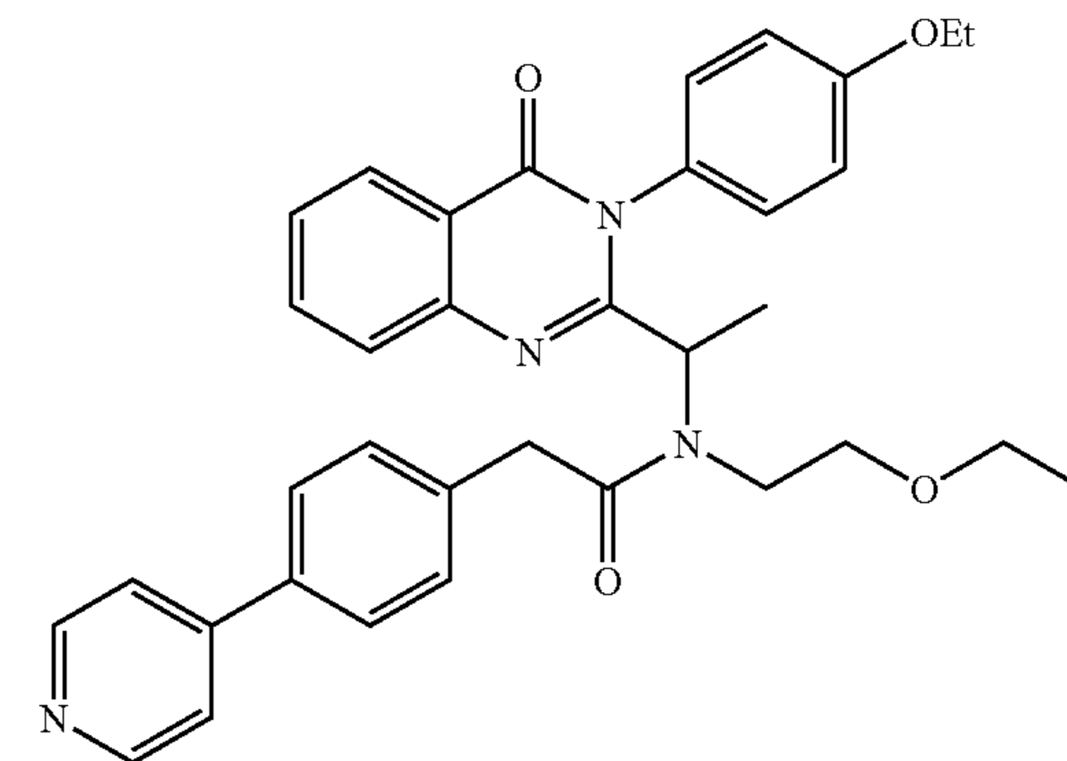
N-(2-Ethoxy-ethyl)-N-(1-[3-(4-ethoxy-phenyl)-4-oxo-3,4-dihydro-quinazolin-2-yl]-ethyl)-2-(4-pyridin-4-yl-phenyl)-acetamide 1.53
