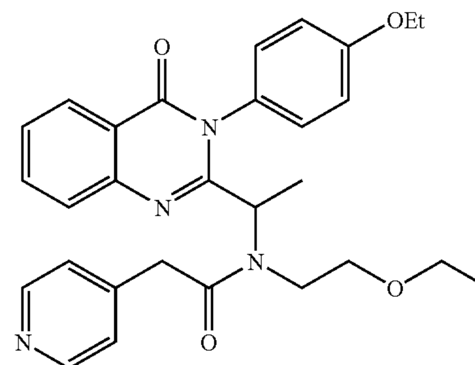
N-(2-Ethoxy-ethyl)-N-{1-[3-(4-ethoxy-phenyl)-4-oxo-3,4-dihydro-quinazolin-2-yl]-ethyl}-2-pyridin-4-yl-acetamide
