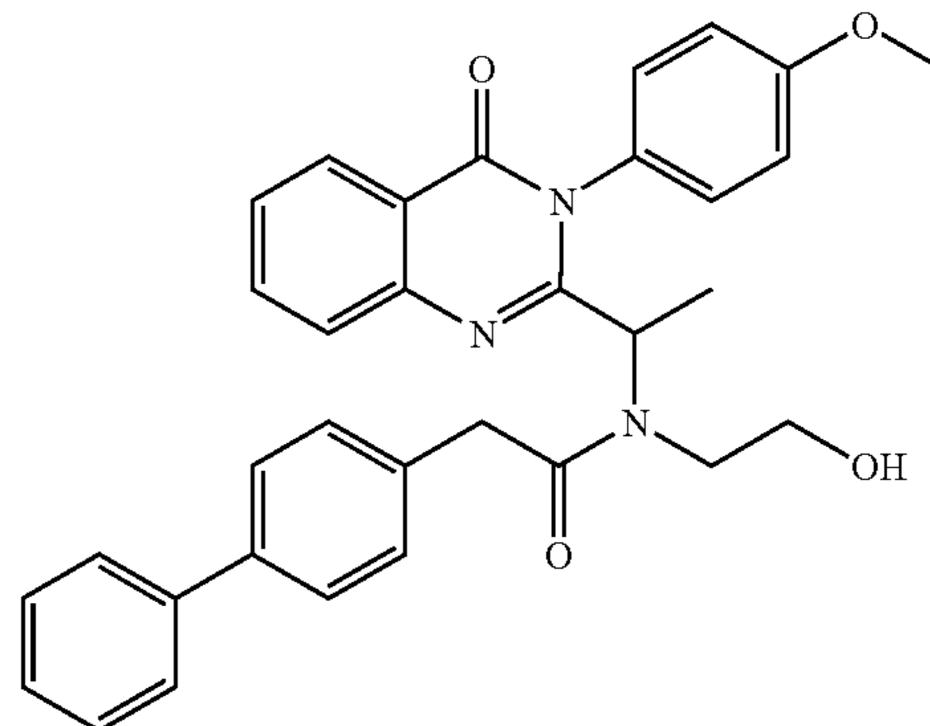
2-Biphenyl-4-yl-N-(2-hydroxy-ethyl)-N-{1-[3-(4-methoxyphenyl)-4-oxo-3,4-dihydro-quinazolin-2-yl]-ethyl}-acetamide
