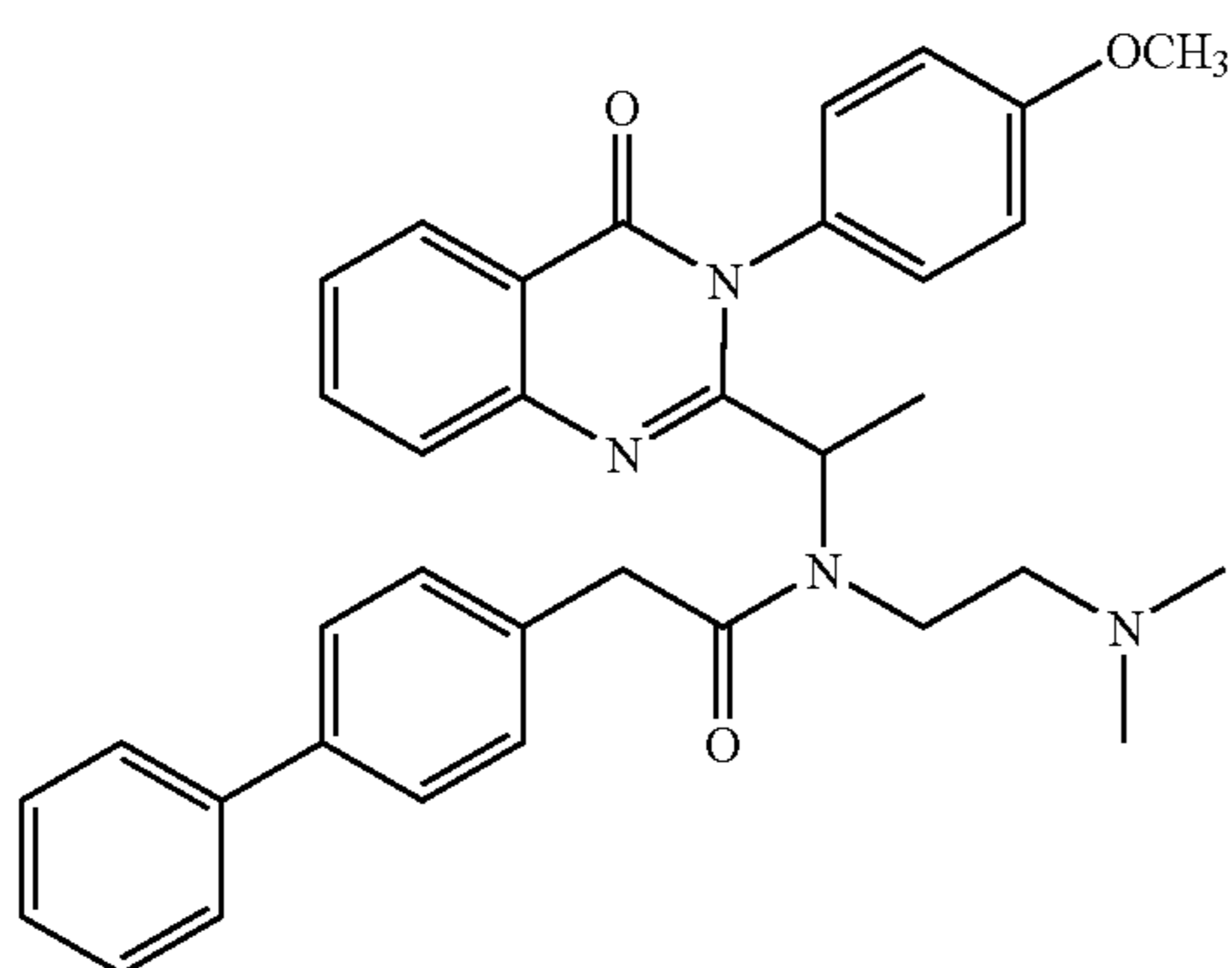
2-Biphenyl-4-yl-N-(2-dimethylamino-ethyl)-N-{1-[3-(4-methoxy-phenyl)-4-oxo-3,4-dihydro-quinazolin-2-yl]-ethyl}-acetamide
