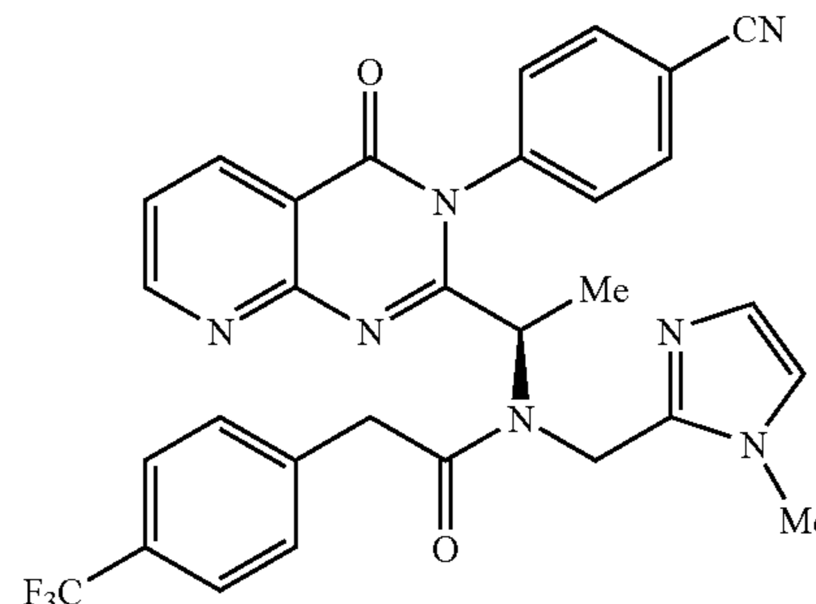
{1R-[3-(4-Cyano-phenyl)-4-oxo-3,4-dihydro-pyrido[2,3-d]pyrimidin-2-yl]-ethyl}-N-(1-methyl-1H-imidazol-2-ylmethyl)-2-(4-trifluoromethyl-phenyl)-acetamide(3.21)
