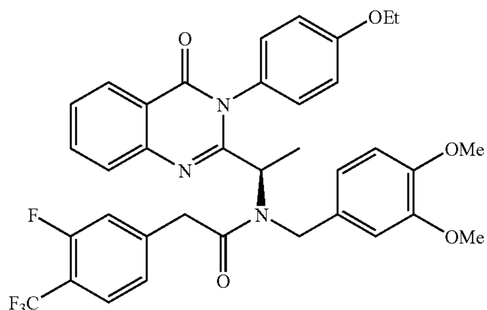
N-(3,4-Dimethoxy-benzyl)-N-{1-[3-(4-ethoxy-phenyl)-4-oxo-3,4-dihydro-quinazolin-2-yl]-ethyl}-2-(3-fluoro-4-trifluoromethyl-phenyl)-acetamide 3.55
