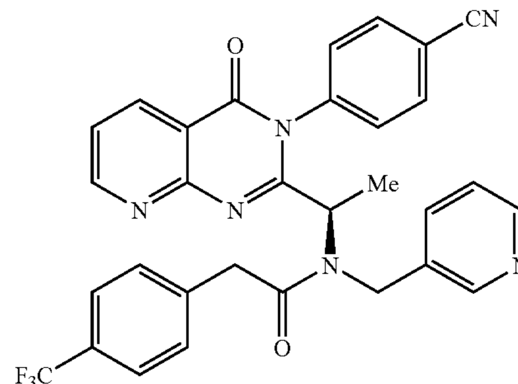
N-{1R-[3-(4-Cyano-phenyl)-4-oxo-3,4-dihydro-pyrido[2,3-d]pyrimidin-2-yl]-ethyl}-N-pyridin-3-ylmethyl-2-(4-trifluoromethyl-phenyl)-acetamide 3.20
