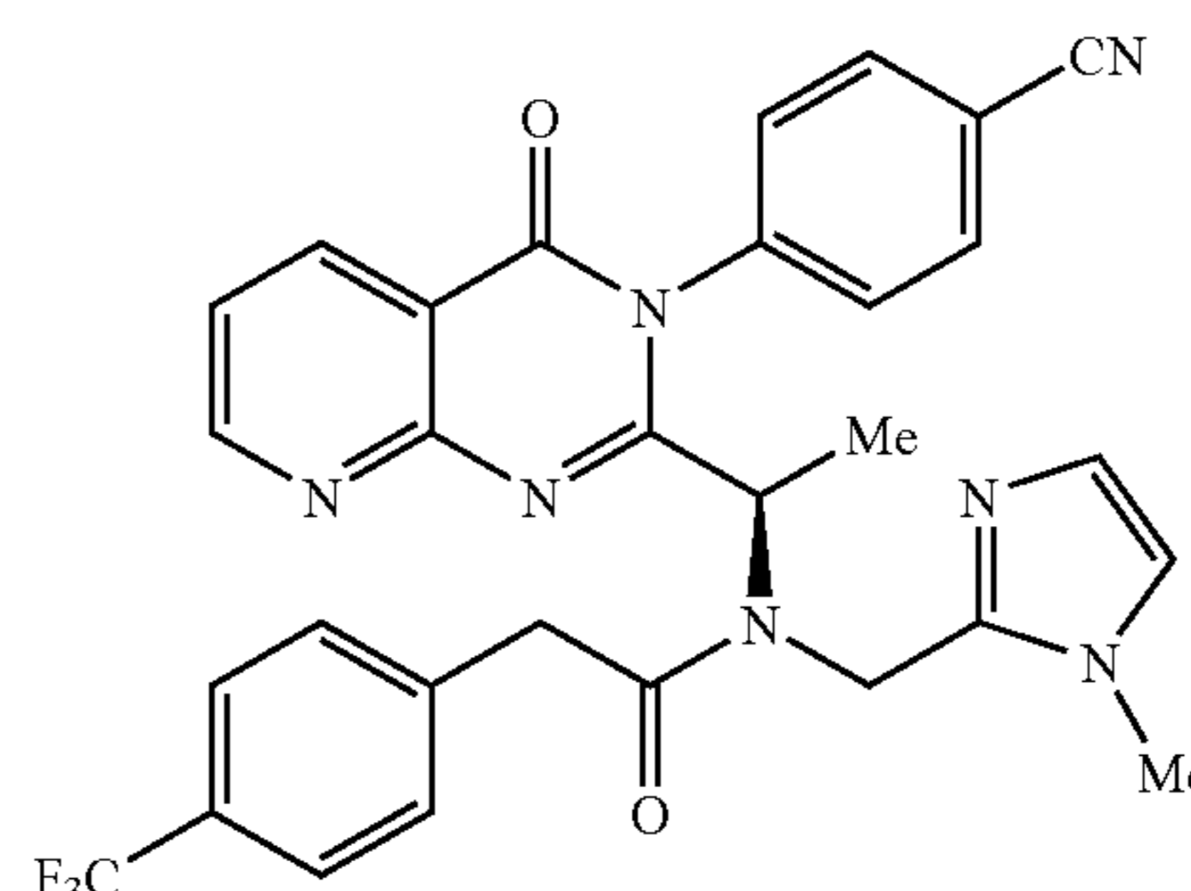
{1R-[3-(4-Cyano-phenyl)-4-oxo-3,4-dihydro-pyrido[2,3-d]pyrimidin-2-yl]-ethyl}-N-(1-methyl-1H-imidazol-2-ylmethyl)-2-(4-trifluoromethyl-phenyl)-acetamide(3.21)
