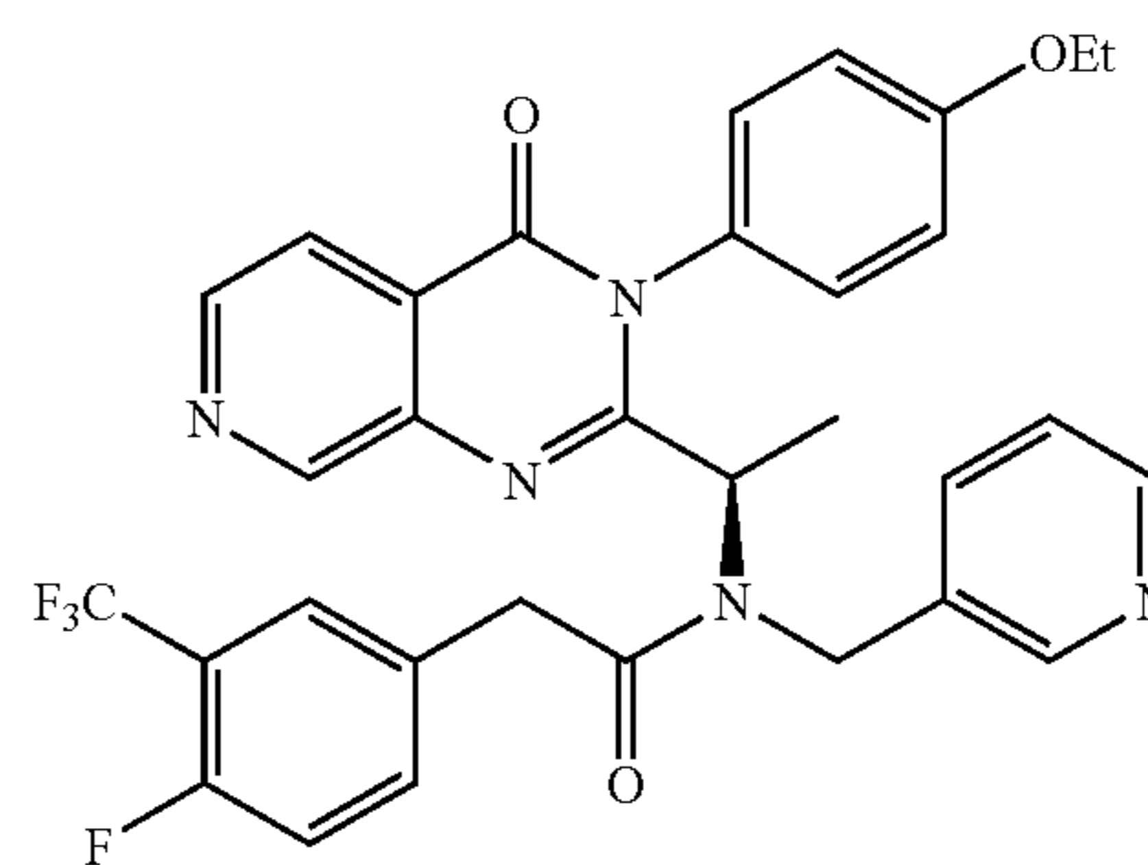
N-{1-[3-(4-Ethoxy-phenyl)-4-oxo-3,4-dihydro-pyrido[3,4-d]pyrimidin-2-yl]-ethyl}-2-(4-fluoro-3-trifluoromethyl-phenyl)-N-pyridin-3-ylmethyl-acetamide 3.56
