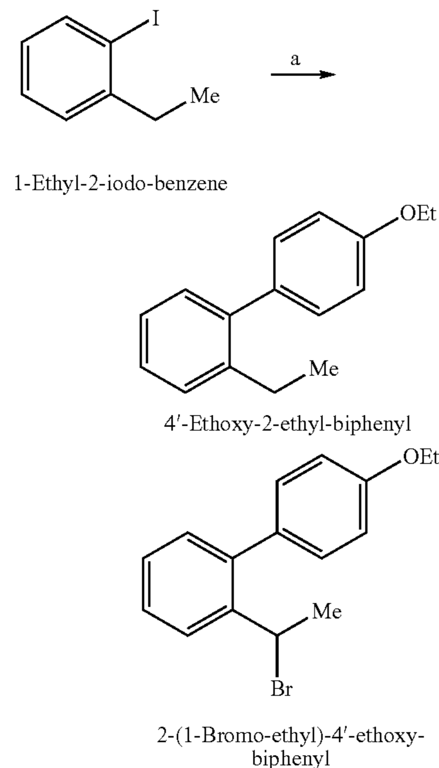
Scheme 13
