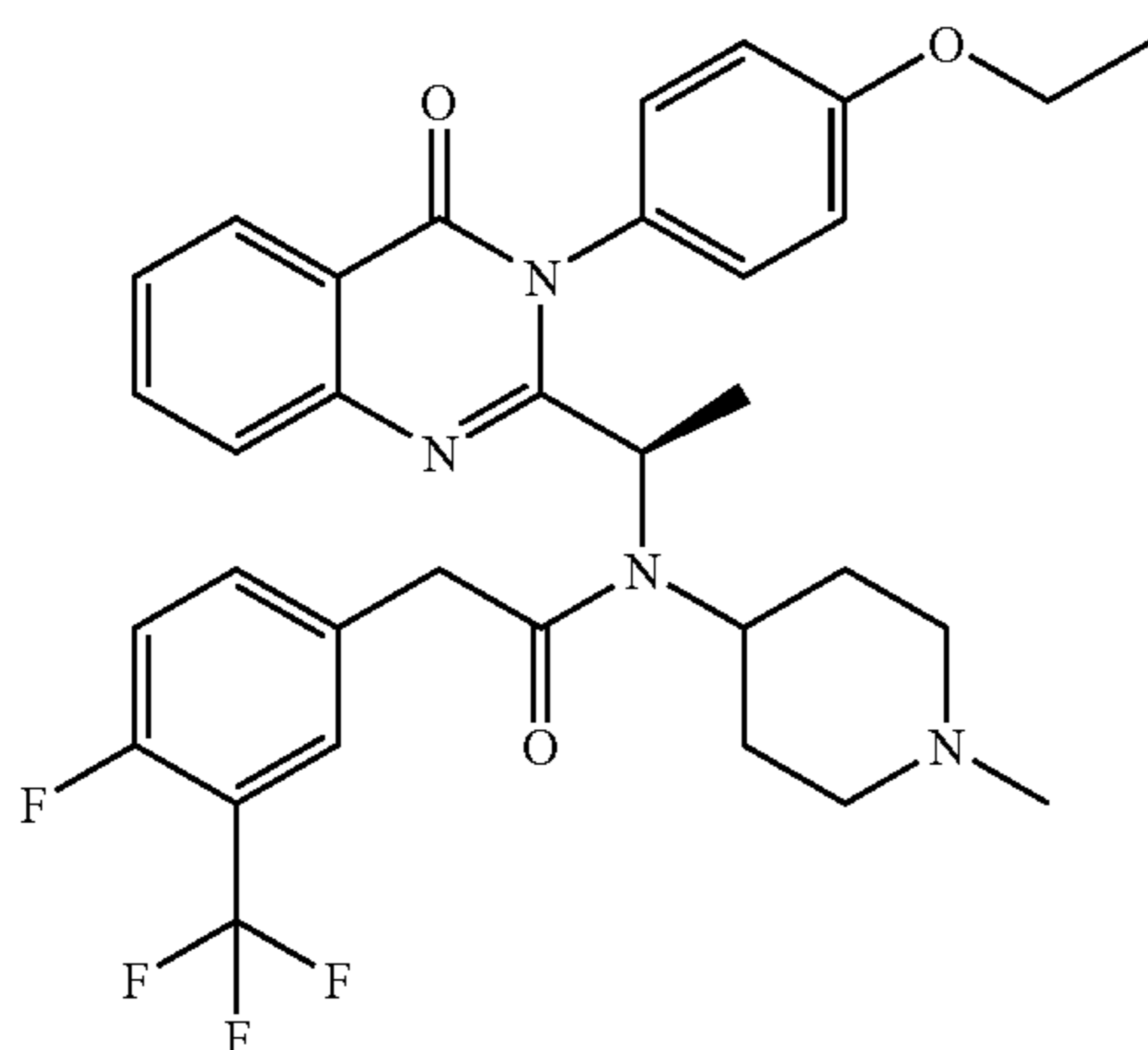
N-{1-[3-(4-Ethoxy-phenyl)-4-oxo-3,4-dihydro-quinazolin-2-yl]-ethyl}-2-(4-fluoro-3-trifluoromethyl-phenyl)-N-(1-methyl-piperidin-4-yl)-acetamide
