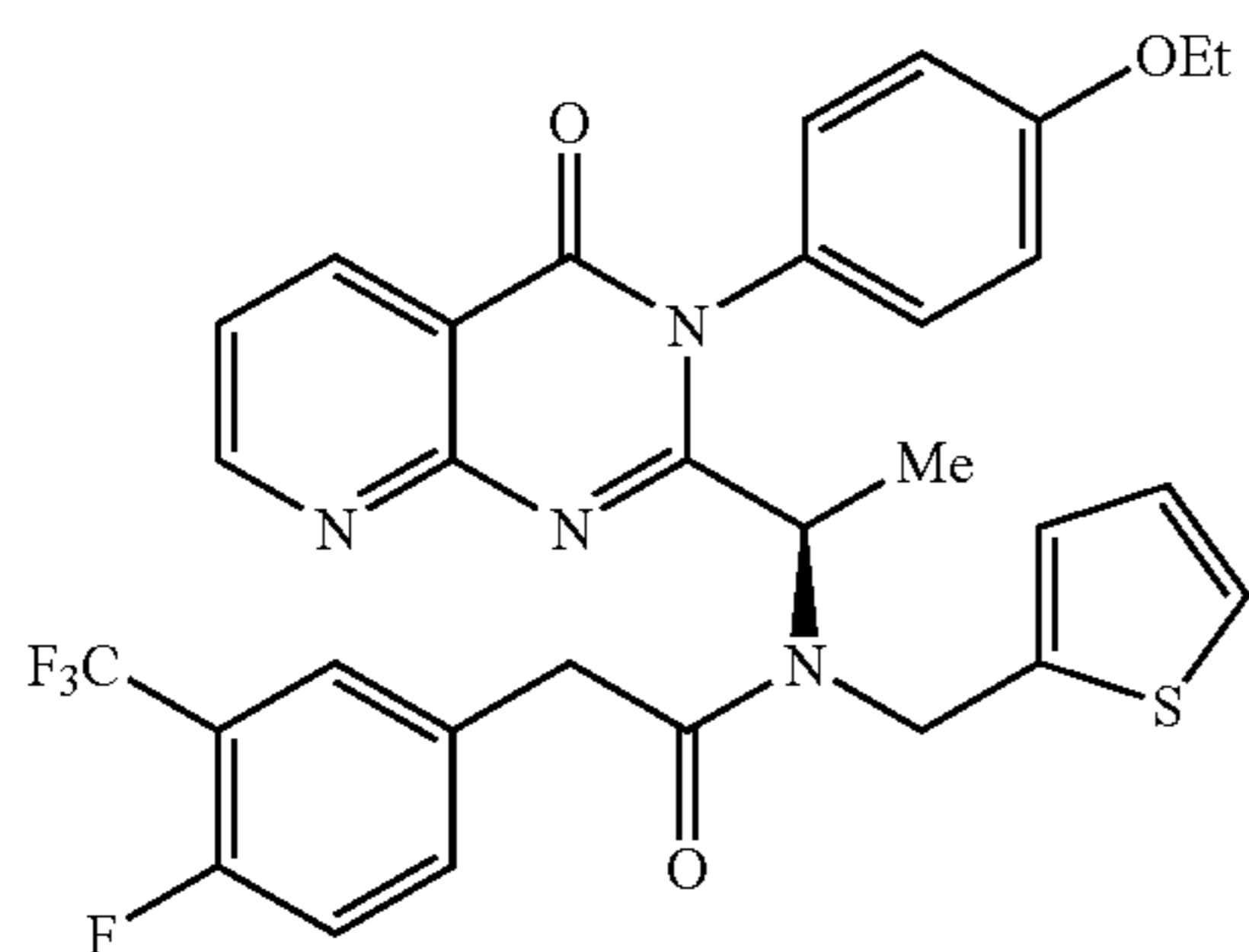
(R)-N-(1-[3-(4-Ethoxy-phenyl)-4-oxo-3,4-dihydro-pyrido[2,3-d]pyrimidin-2-yl]-ethyl)-2-(4-fluoro-3-trifluoromethyl-phenyl)-N-thiophen-2-ylmethyl-acetamide 3.65
