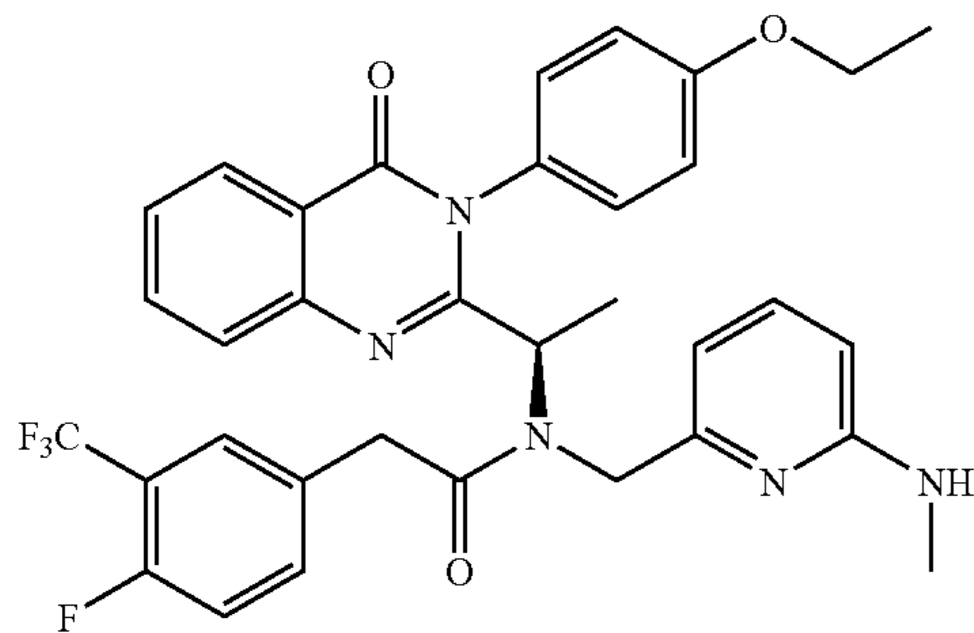
(-)-(R)-N-({1-[3-(4-Ethoxy-phenyl)-4-oxo-3,4-dihydroquinazolin-2-yl]-ethyl}-2-(4-fluoro-3-trifluoromethyl-phenyl)-N-(6-methylamino-pyridin-2-ylmethyl)-acetamide 3.73
