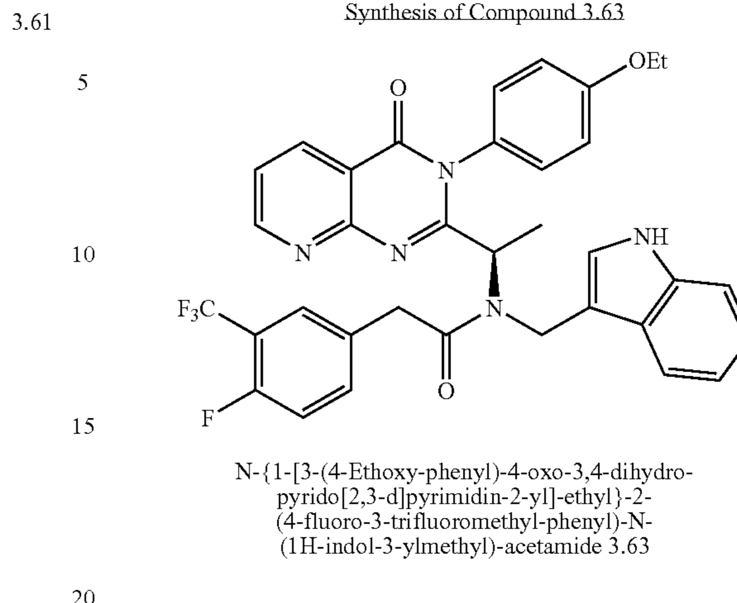
Synthesis of Compound 3.63
