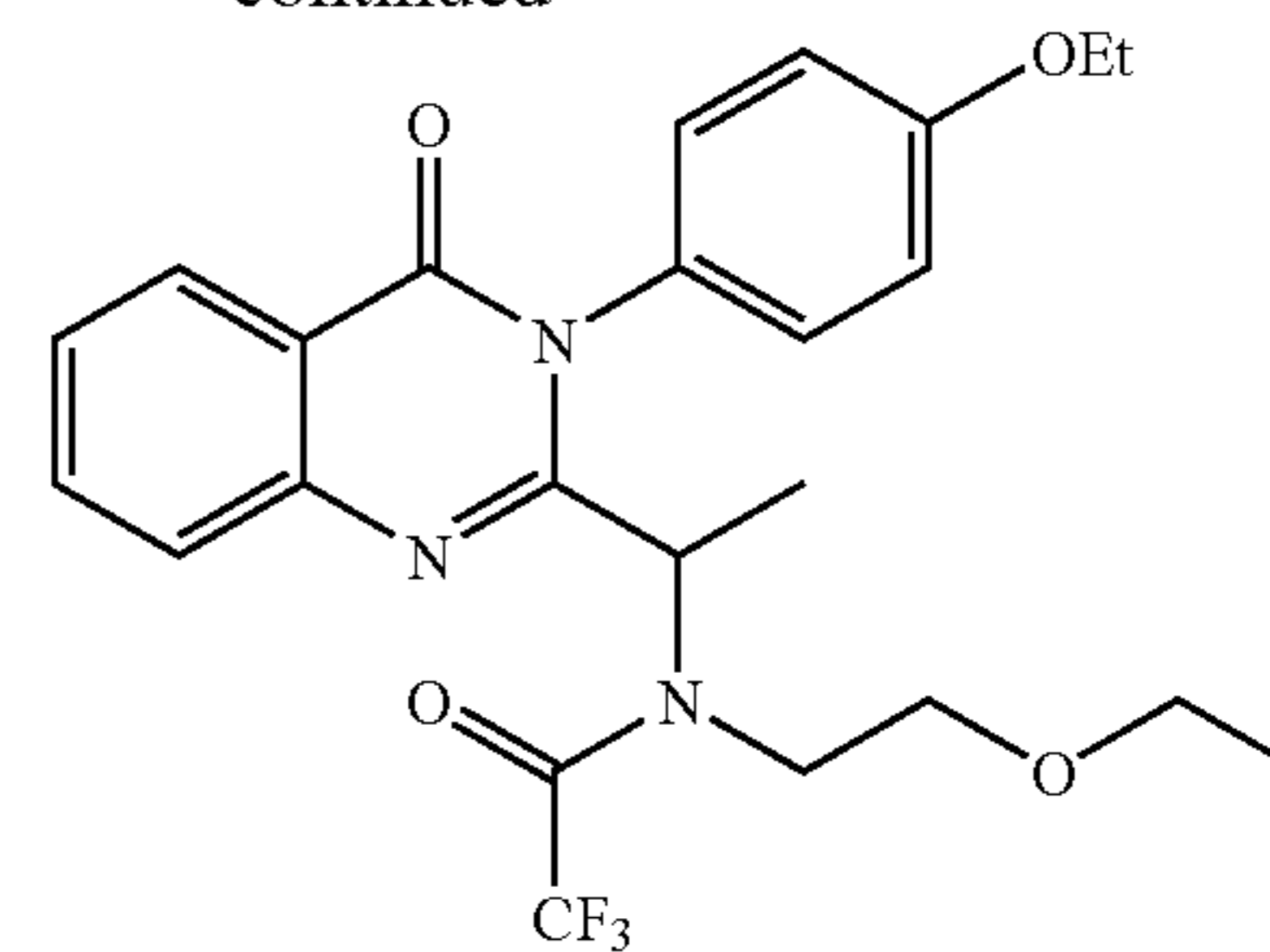
N-(2-Ethoxy-ethyl)-N-{1-[3-(4-ethoxy-phenyl)-4-oxo-3,4-dihydro-quinazolin-2-yl]-ethyl}-2,2,2-trifluoroacetamide 1.55
