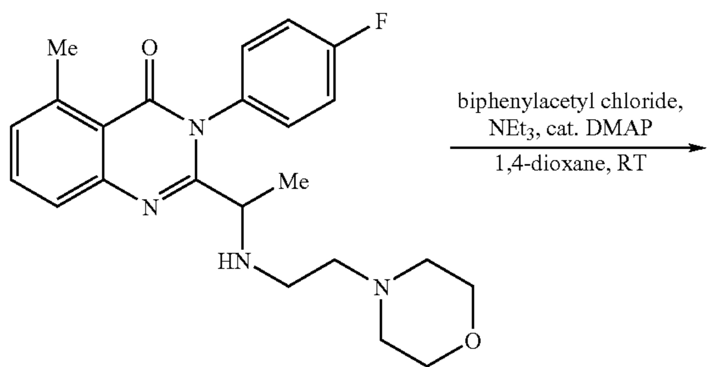
3-(4-fluoro-phenyl)- 5-methyl-2-[1-(2-morpholin-4-yl-ethylamino)- ethyl]-3H-quinazolin-4-one (XI)
