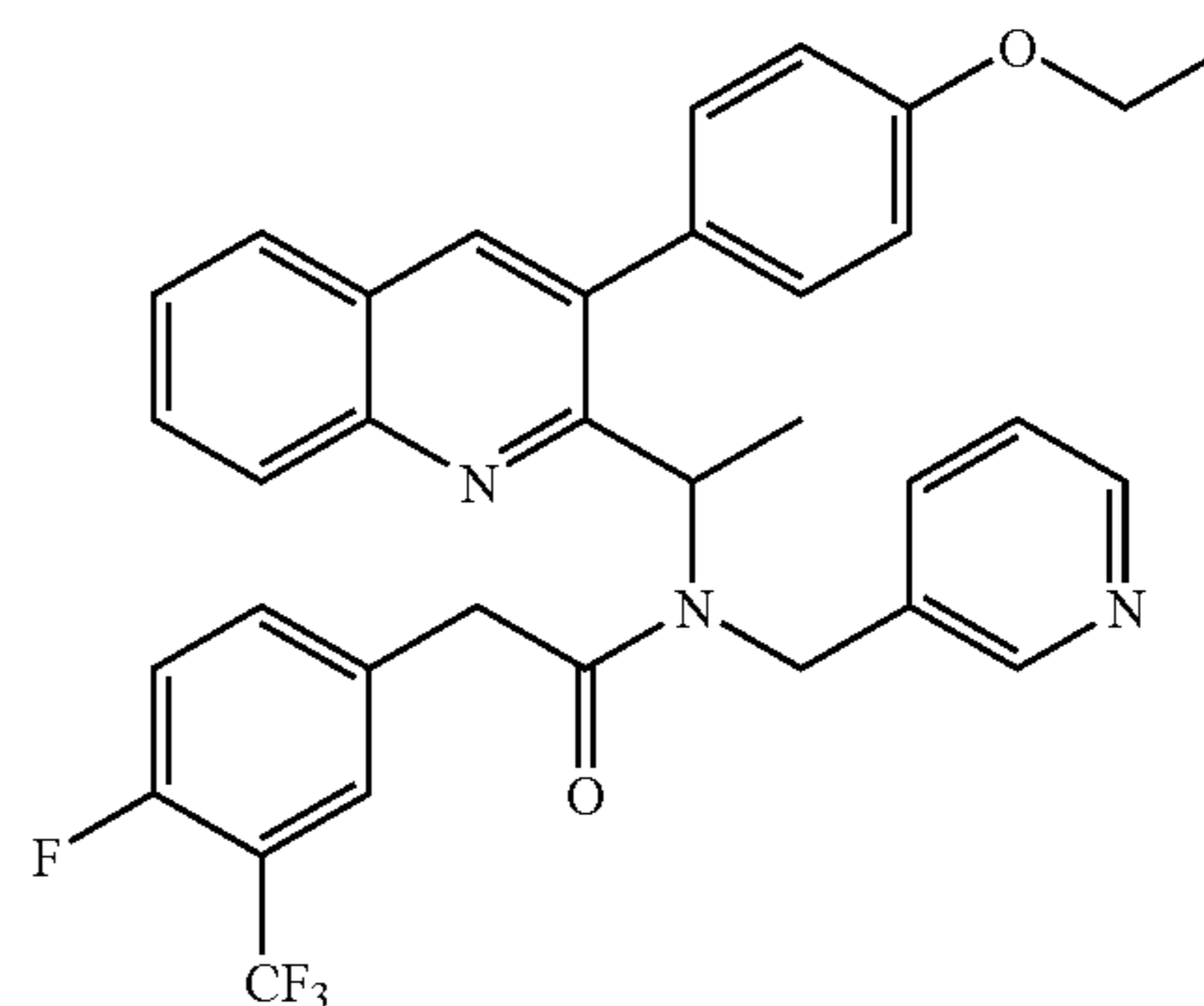
N-{1-[3-(4-Ethoxy-phenyl)-quinolin-2-yl]-ethyl}-2-(4-fluoro-3-trifluoromethyl-phenyl)-N-pyridin-3-ylmethyl-acetamide
