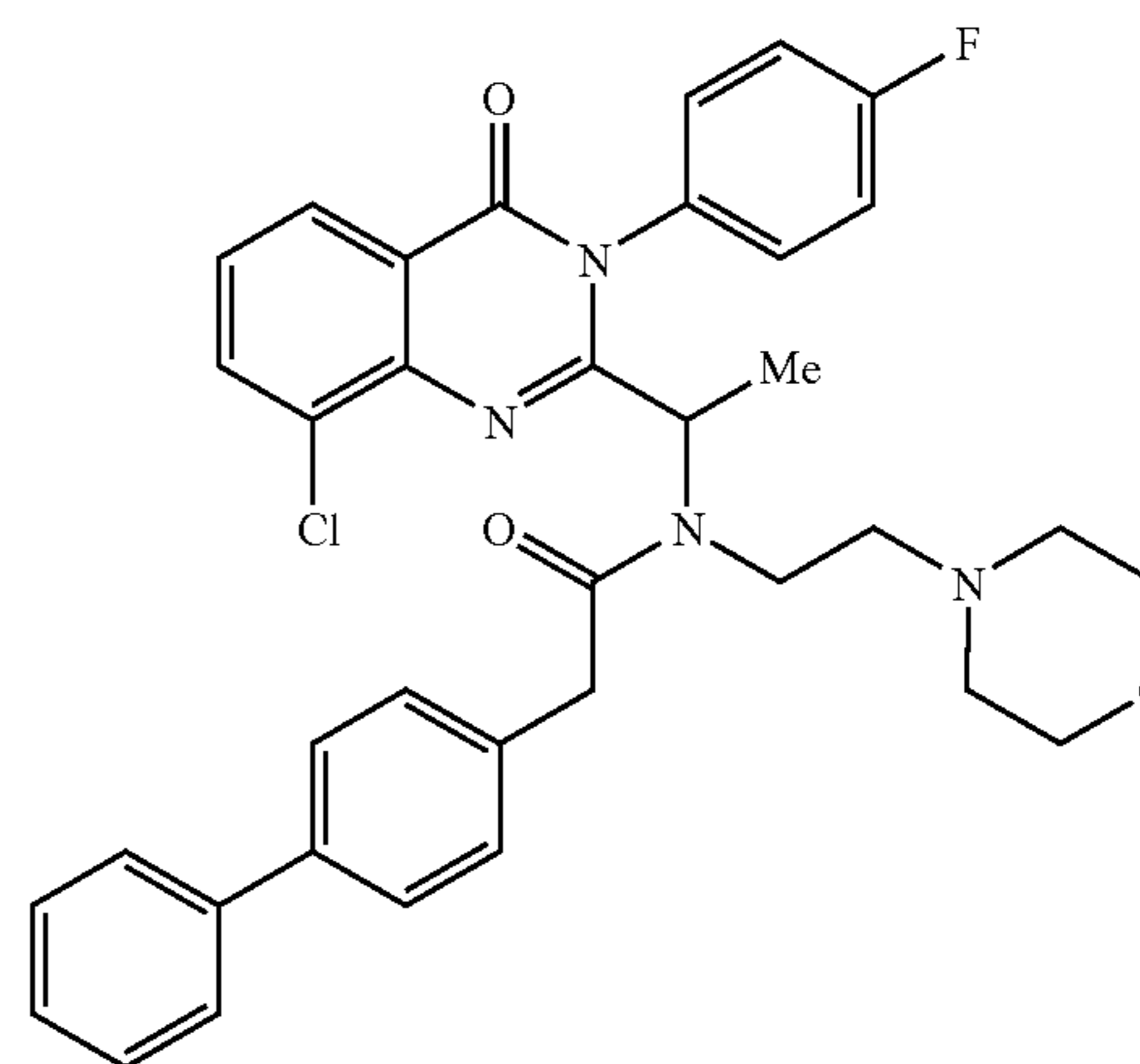
2-Biphenyl-4-yl-N-{1-[8-chloro-3-(4-fluoro-phenyl)- 4-oxo-3,4-dihydro-quinazolin-2-yl]-ethyl}-N- (2-morpholin-4-yl-ethyl)-acetamide
