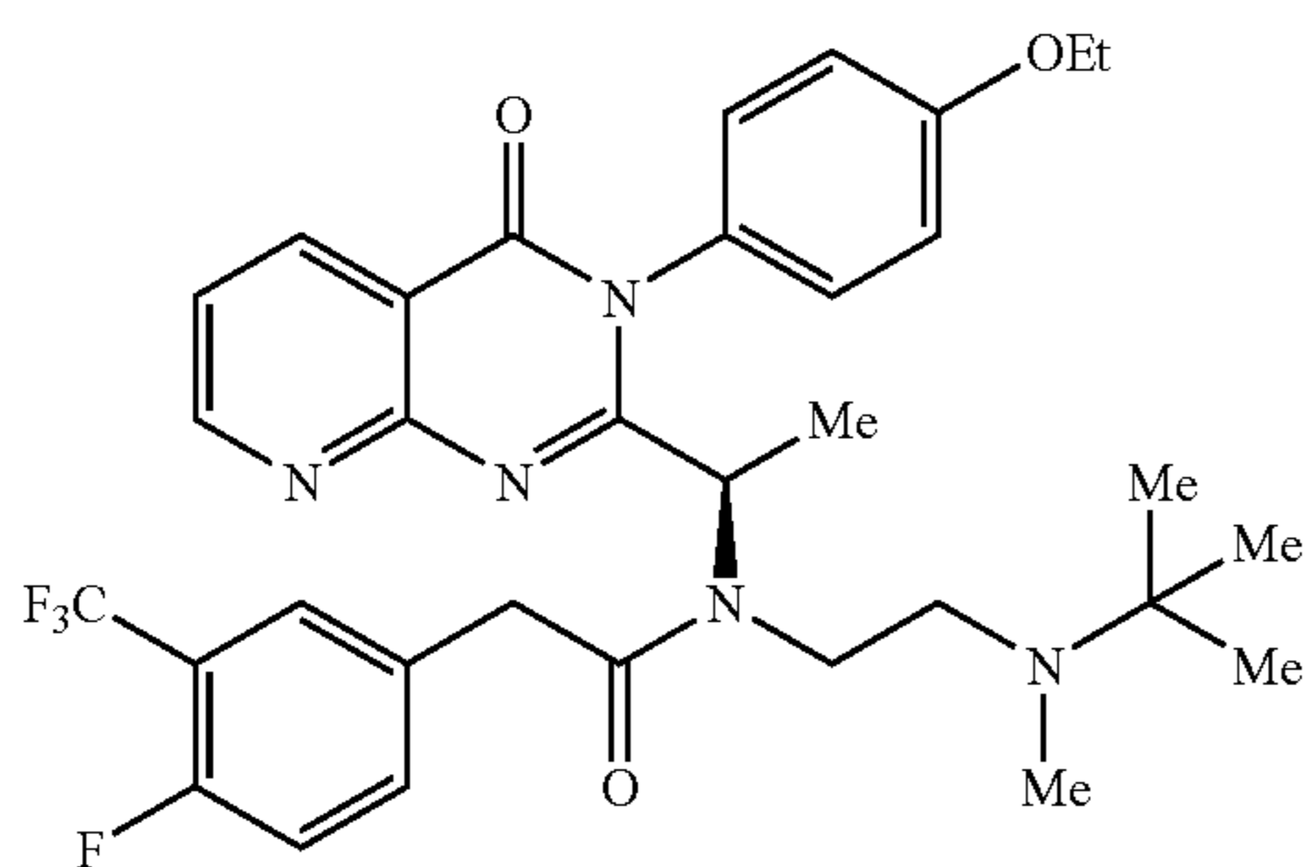
(R)-N-[2-(tert-Butyl-methyl-amino)-ethyl]-N-(1-[3-(4-ethoxy-phenyl)-4-oxo-3,4-dihydro-pyrido[2,3-d]pyrimidin-2-yl]-ethyl)-2-(4-fluoro-3-trifluoromethyl-phenyl)-acetamide 3.66
