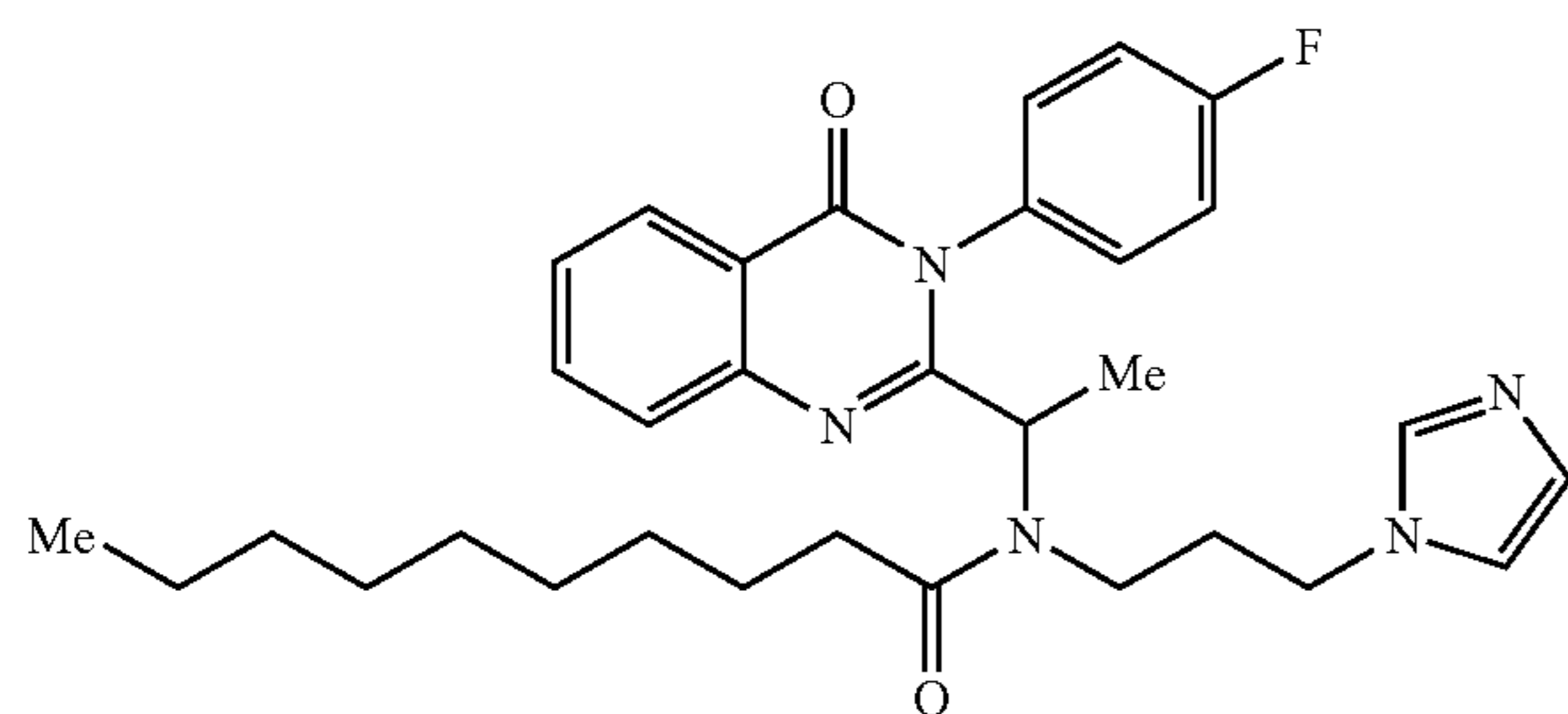
Decanoic acid {1-[3-(4-fluoro-phenyl)-4-oxo-3,4-dihydro-quinazolin-2-yl]-ethyl}-(3-imidazol-1-yl-propyl)-amide
