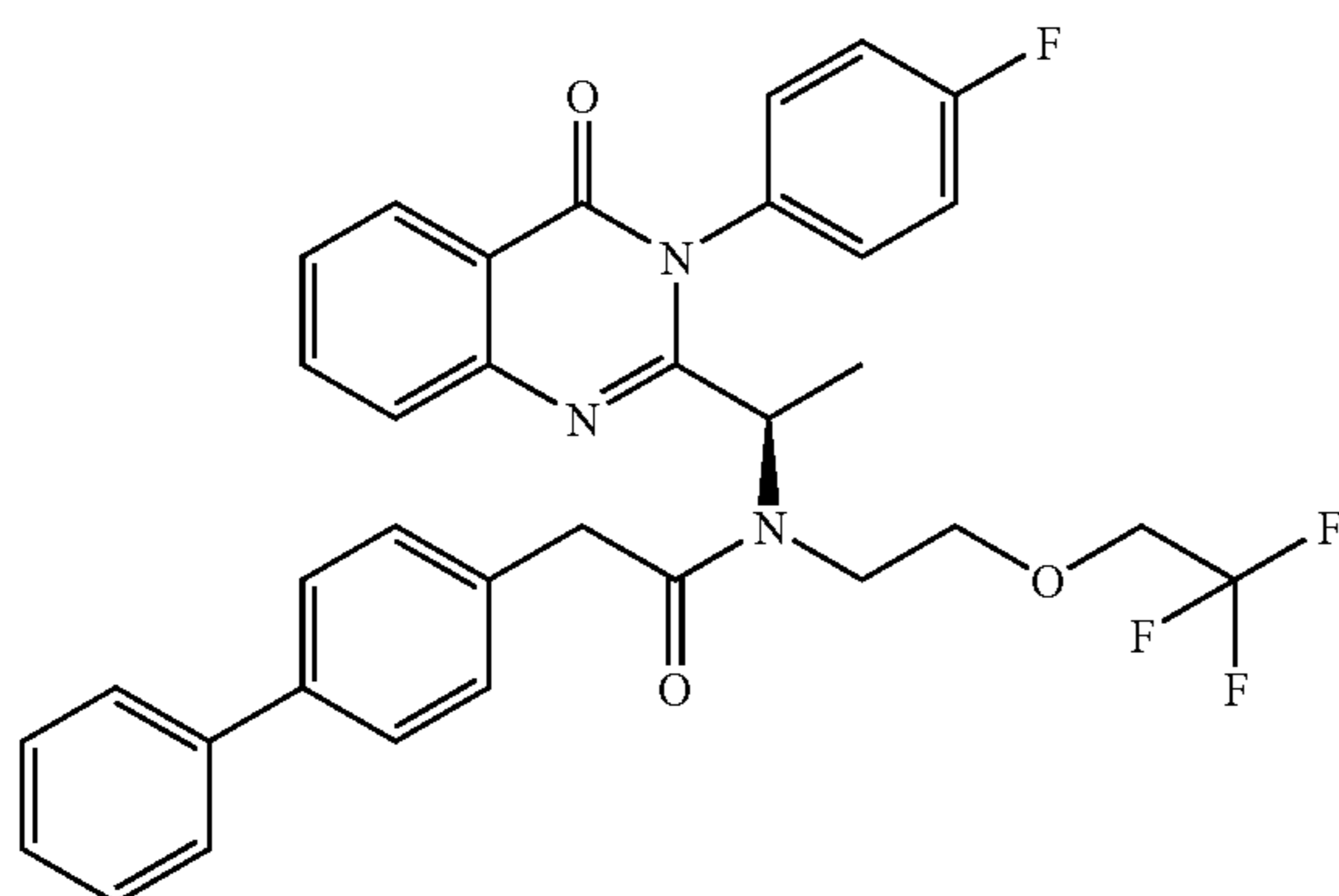
2-Biphenyl-4-yl-N-(1-[3-(4-fluoro-phenyl)-4-oxo-3,4-dihydro-quinazolin-2-yl]-ethyl)-N-[2-(2,2,2-trifluoro-ethoxy)-ethyl]-acetamide
