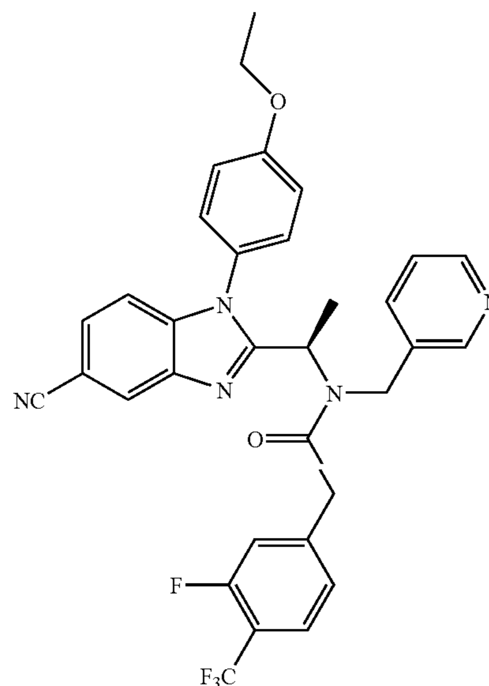
N-{1-[5-Cyano-1-(4-ethoxy-phenyl)-1H-benzimidazol-2-yl]-ethyl}-2-(3-fluoro-4-trifluoromethyl-phenyl)-N-pyridin-3-ylmethyl-acetamide
