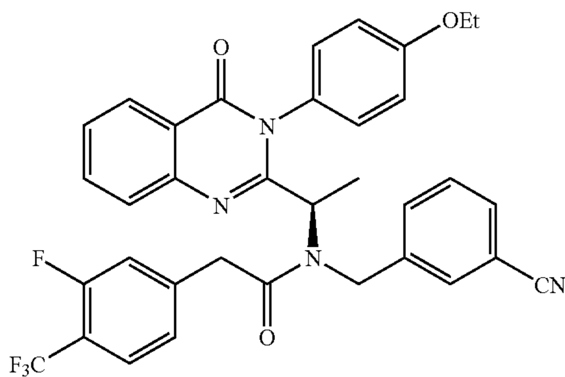
N-(3-Cyano-benzyl)-N-{1-[3-(4-ethoxy-phenyl)-4-oxo-3,4-dihydro-quinazolin-2-yl]-ethyl}-2-(3-fluoro-4-trifluoromethyl-phenyl)-acetamide 3.54
