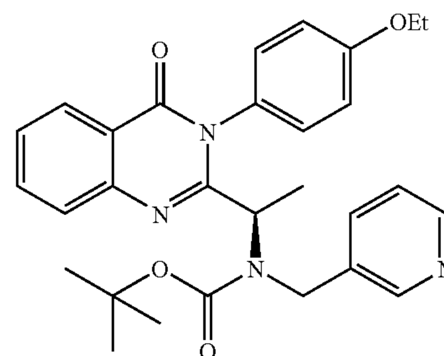
Synthesis of Compound 3.16
