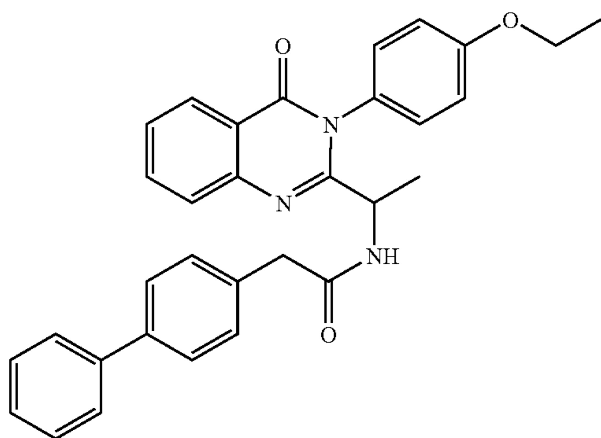
2-Biphenyl-4-yl-N-{1-[3-(4-ethoxy-phenyl)-4-oxo-3,4-dihydro-quinazolin-2-yl]-ethyl}-acetamide
