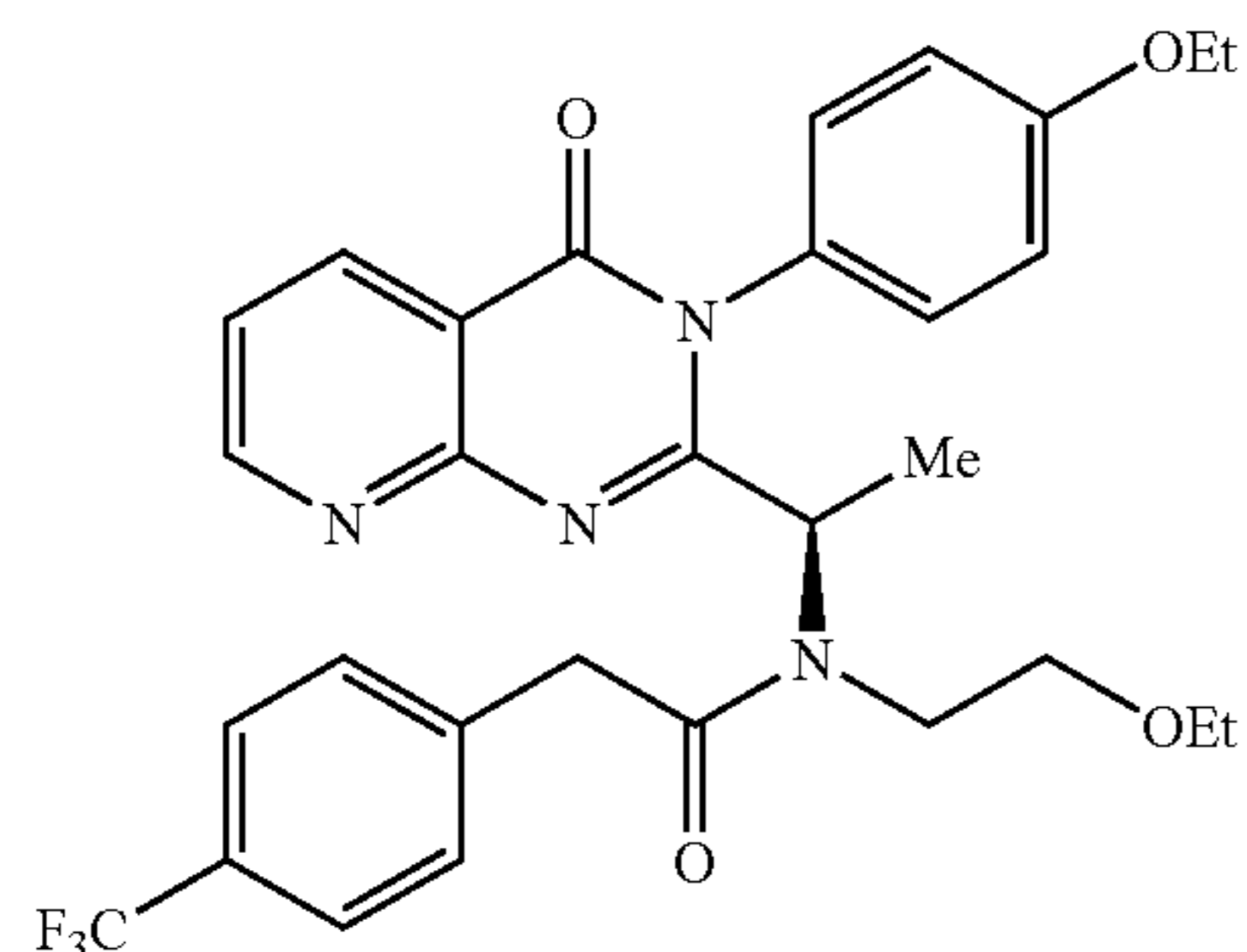
N-(2-Ethoxy-ethyl)-N-{1R-[3-(4-ethoxy-phenyl)-4-oxo-3,4-dihydro-pyrido[2,3-d]pyrimidin-2-yl]-ethyl}-2-(4-trifluoromethyl-phenyl)-acetamide(3.18)
