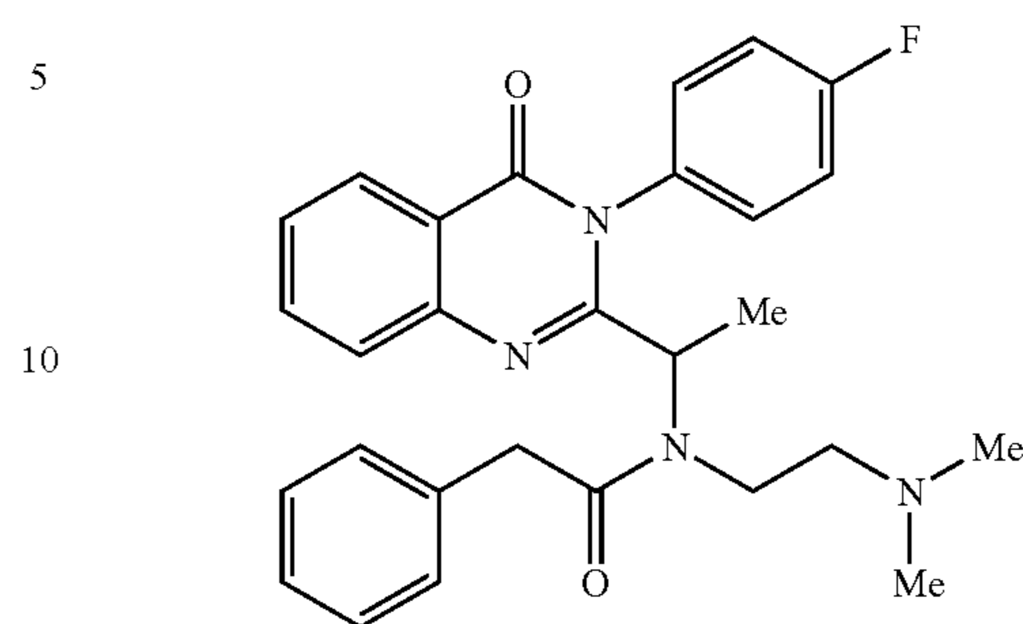
N-(2-Dimethylamino-ethyl)-N-{1-[3-(4-fluoro-phenyl)-4-oxo-3,4-dihydro-quinazolin-2-yl]-ethyl}-2-phenylacetamide(1.09)
