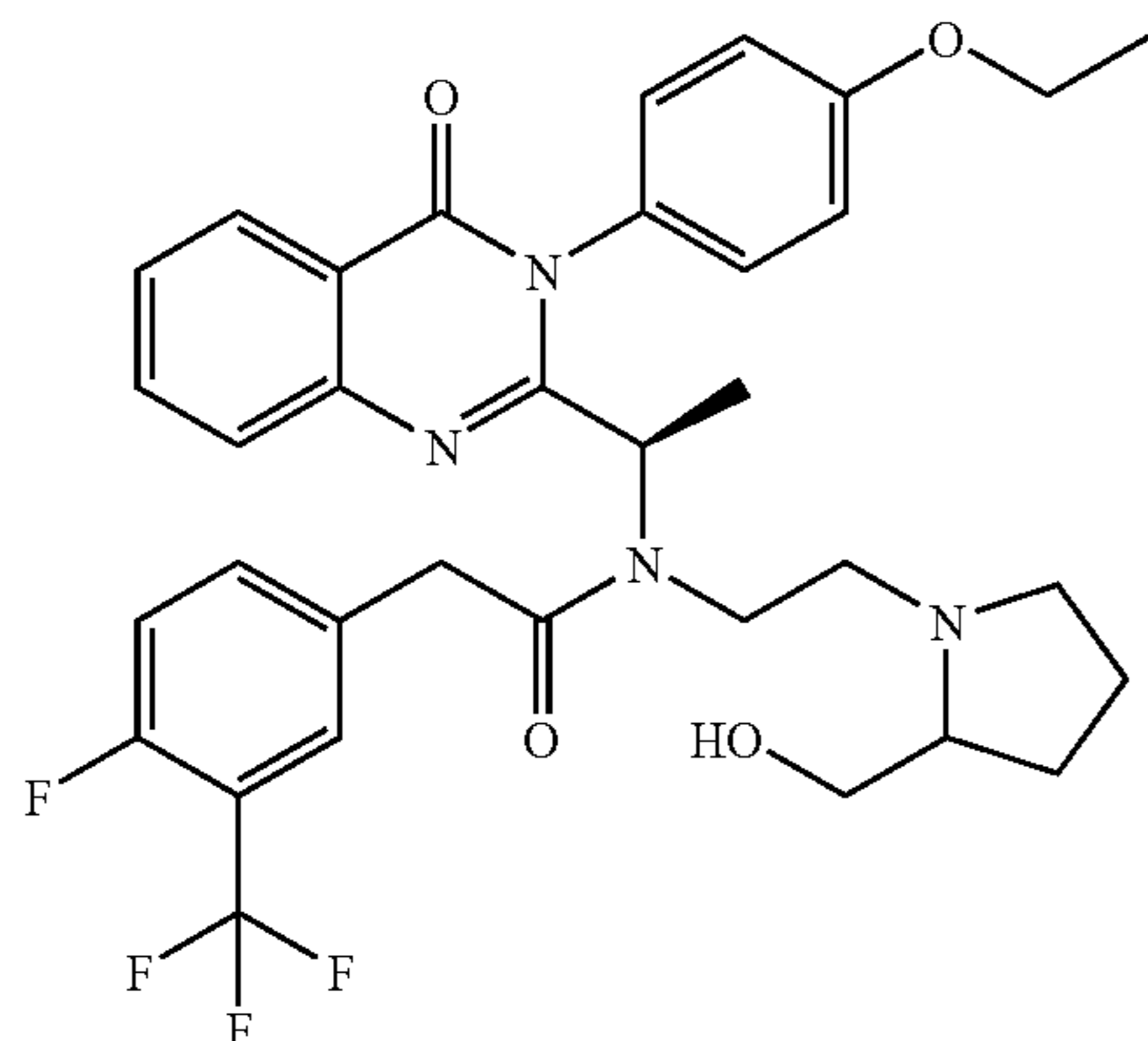
(s)-N-{1-[3-(4-Ethoxy-phenyl)-4-oxo-3,4-dihydroquinazolin-2-yl]-ethyl}-2-(4-fluoro-3-trifluoromethyl-phenyl)-N-[2-(2-hydroxymethyl-pyrrolidin-1-yl)ethyl]-acetamide
