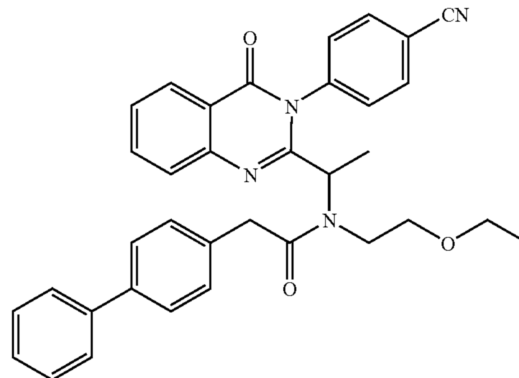
2-Biphenyl-4-yl-N-{1-[3-(4-cyano-phenyl)-4-oxo-3,4-dihydro-quinazolin-2-yl]-ethyl}-N-(2-ethoxy-ethyl)-acetamide
