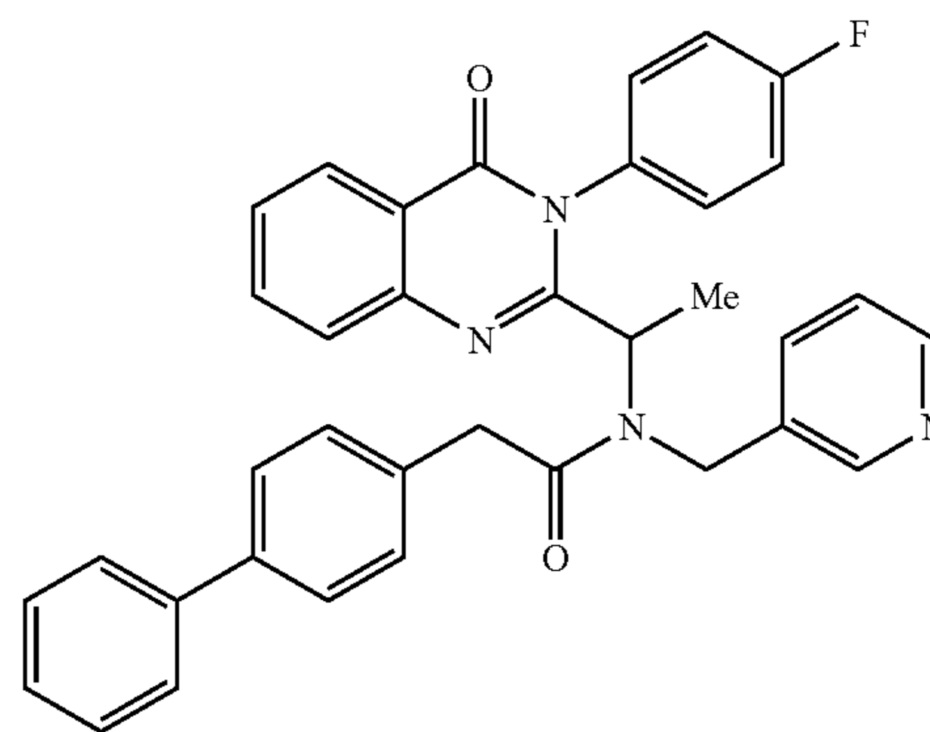
2-Biphenyl-4-yl-N-{1-[3-(4-fluoro-phenyl)-4-oxo-3,4-dihydro-quinazolin-2-yl]-ethyl}-N-pyridin-3-ylmethyl-acetamide
