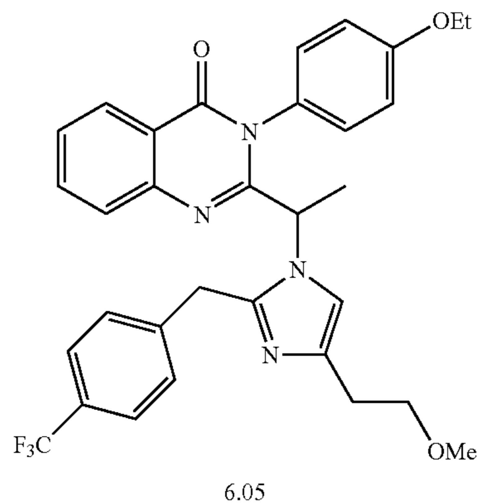
Preparation of Compound 6.05
