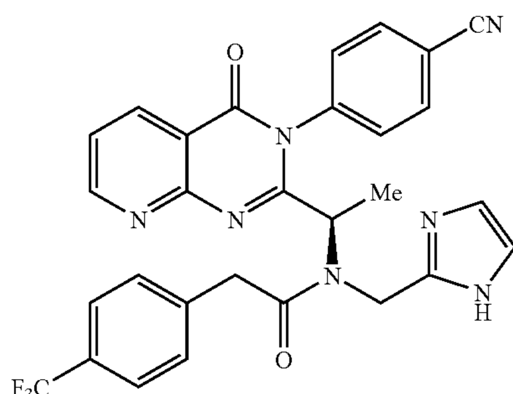
N-{1R-[3-(4-Cyano-phenyl)-4-oxo-3,4-dihydro-pyrido pyrimidin-2-yl]-ethyl}-(1H-imidazol-2-ylmethyl)-2-(4-trifluoromethyl-phenyl)-acetamide 3.19
