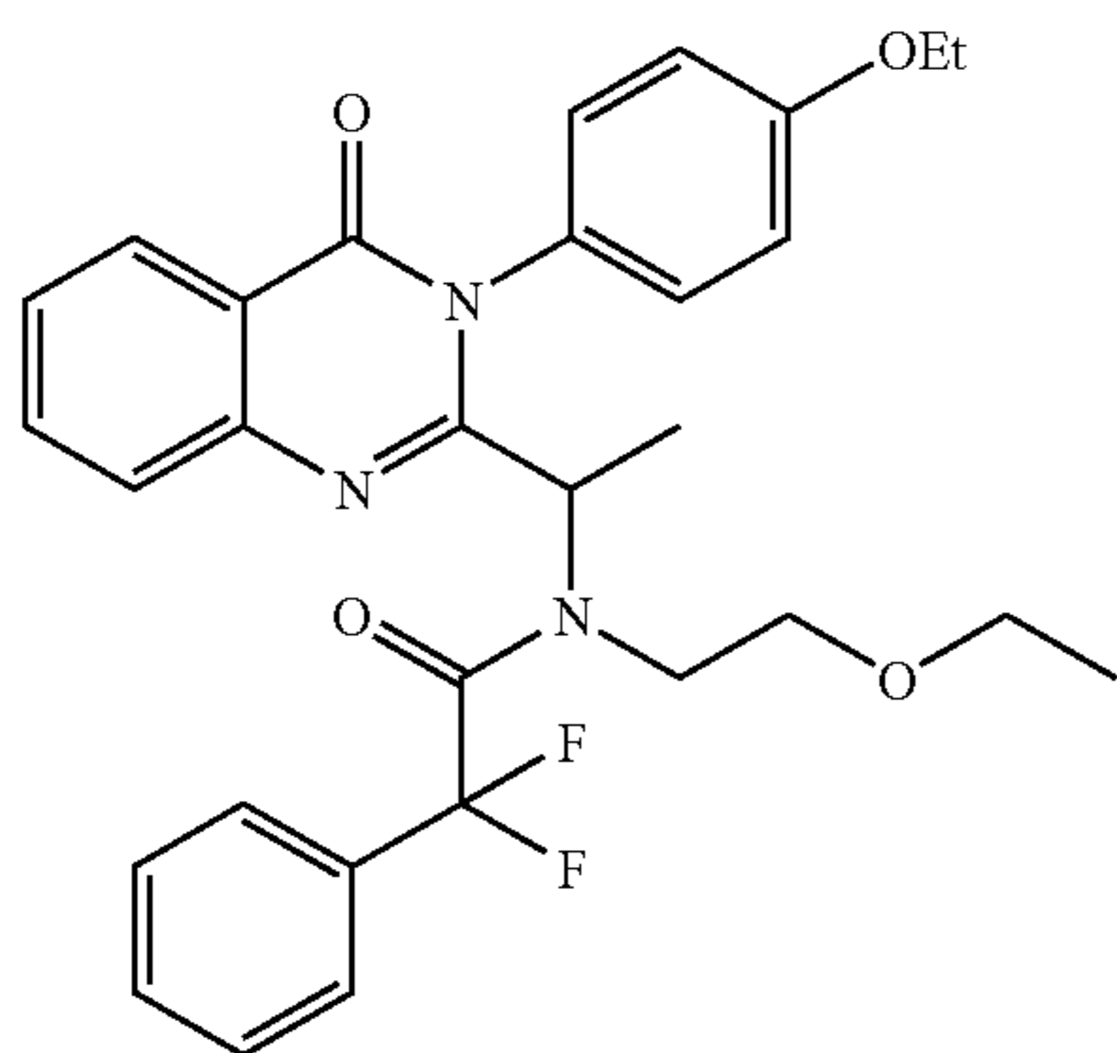
N-(2-Ethoxy-ethyl)-N-{1-[3-(4-ethoxy-phenyl)-4-oxo-3,4-dihydroquinolin-2-yl]-ethyl}-2,2-difluoro-2-phenyl-acetamide
