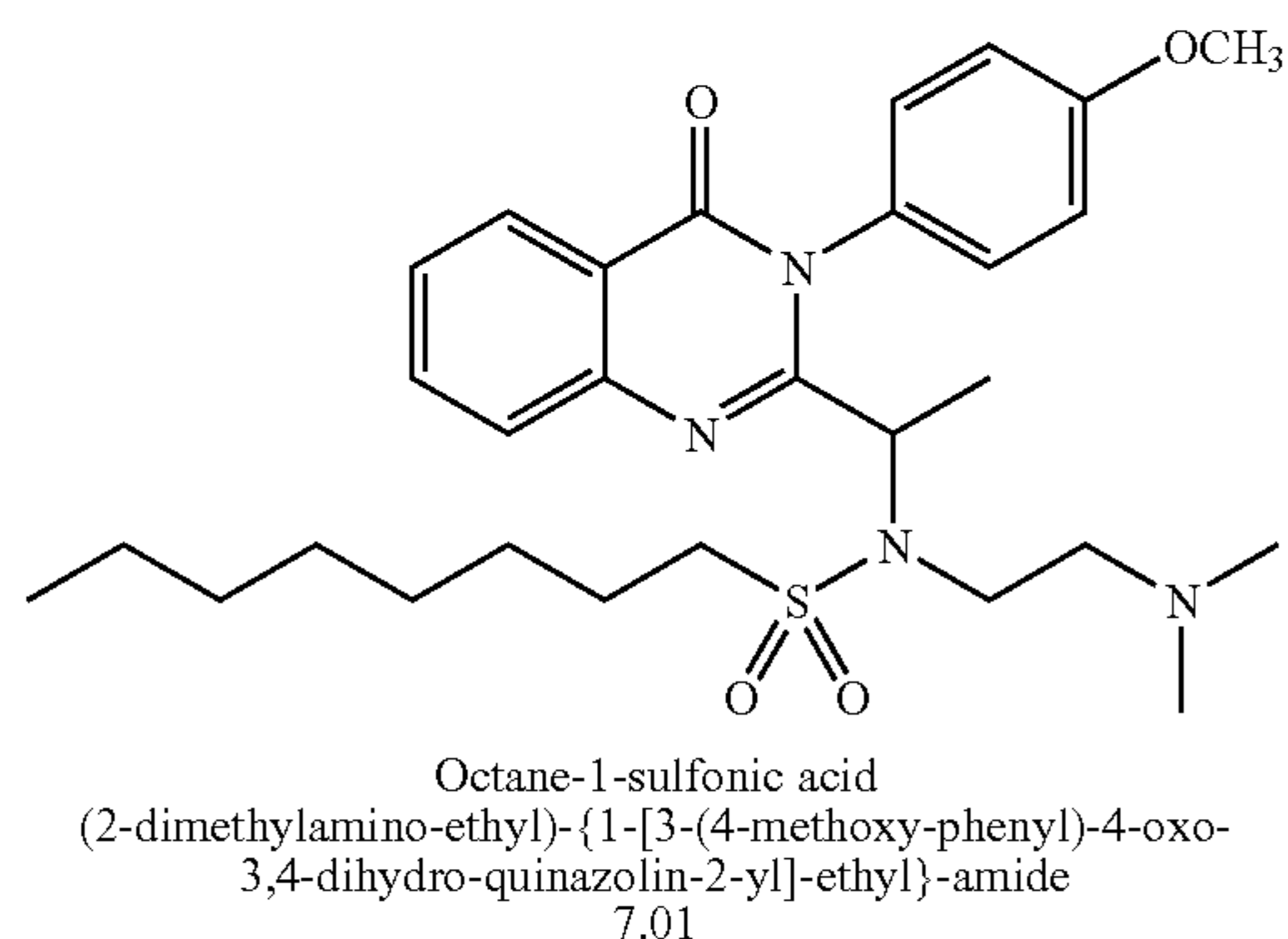
2-[1-(2-Dimethylamino-ethylamino)-ethyl]-3-(4-methoxy-phenyl)-3H-quinazolin-4-one
