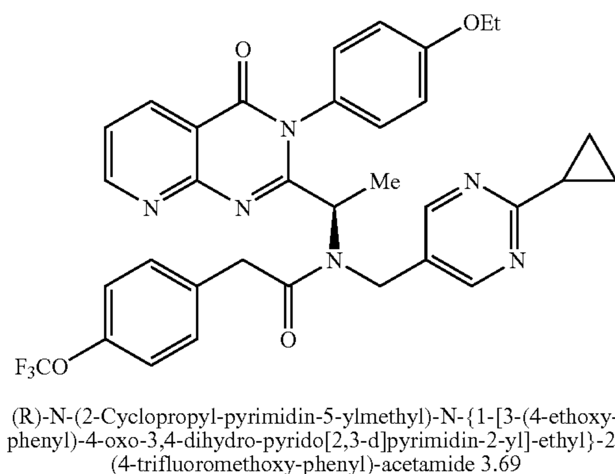
Synthesis of Compound 3.69
