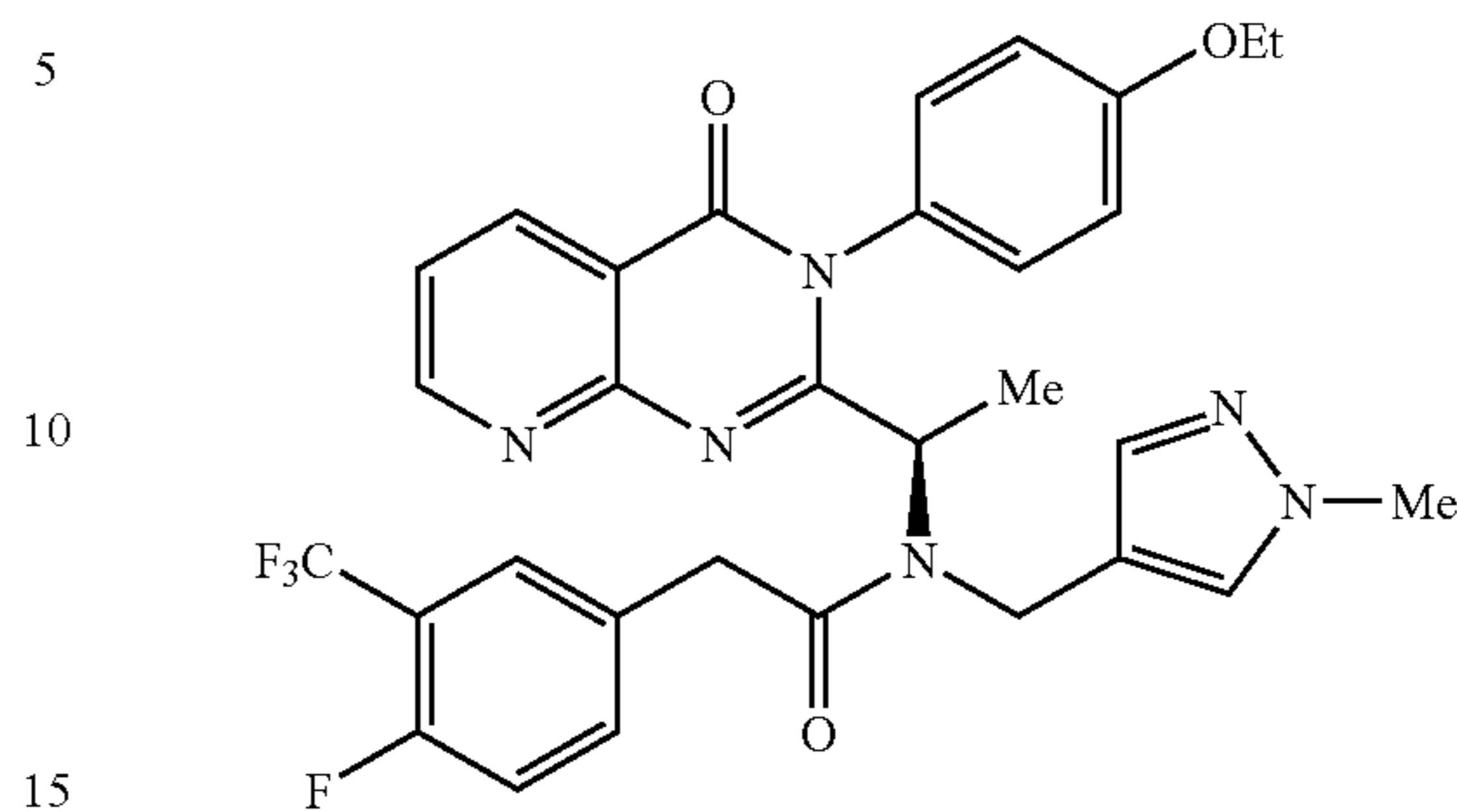
(R)-N-(1-[3-(4-Ethoxy-phenyl)-4-oxo-3,4-dihydro-pyrido[2,3-d]pyrimidin-2-yl]-ethyl)-2-(4-fluoro-3-trifluoromethyl-phenyl)-N-(1-methyl-1H-pyrazol-4-ylmethyl)-acetamide 3.67
