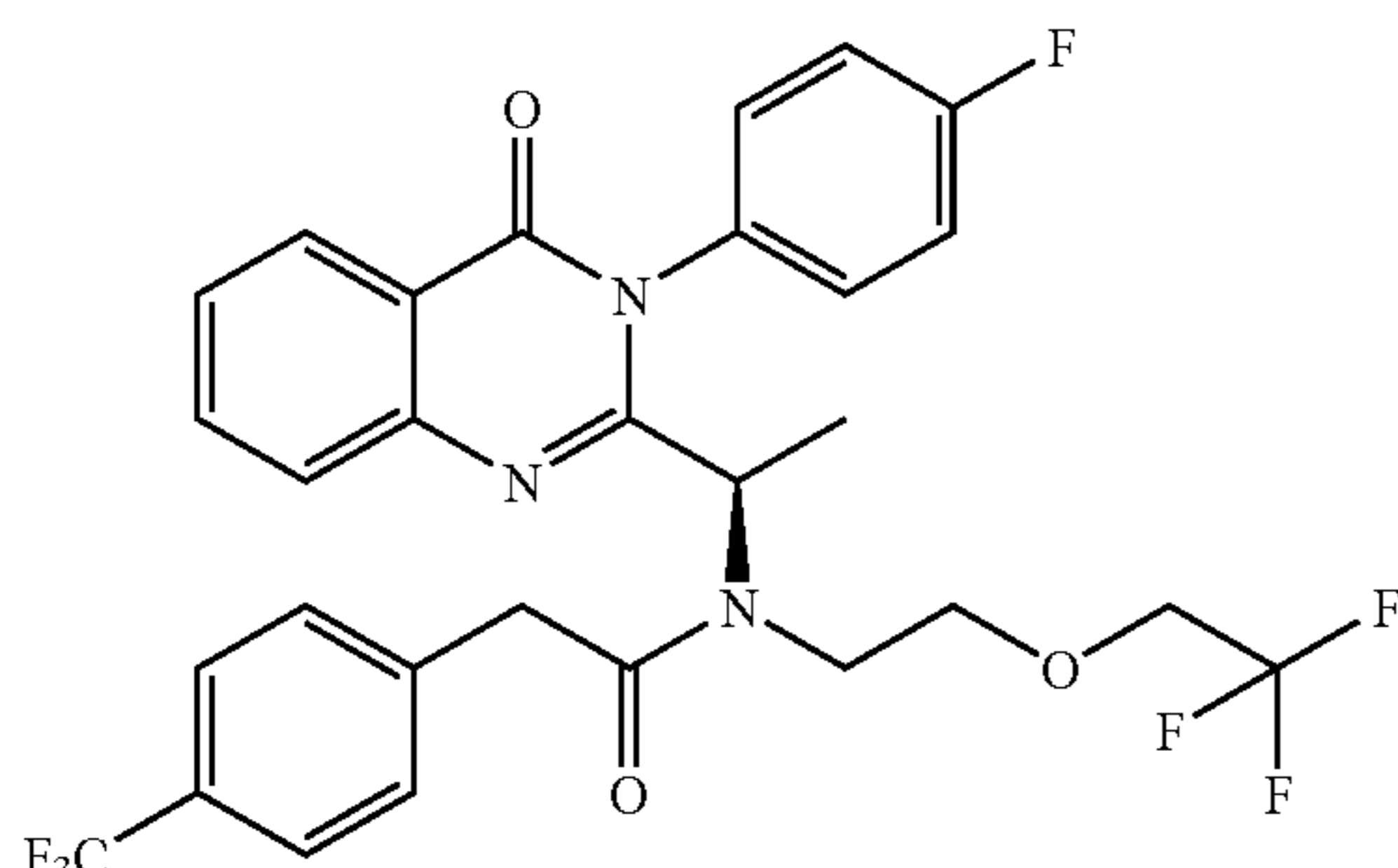
N-(1-[3-(4-Fluoro-phenyl)-4-oxo-3,4-dihydro-quinazolin-2-yl]-ethyl)-N-[2-(2,2,2-trifluoro-ethoxy)-ethyl]-2-(4-trifluoromethyl-phenyl)-acetamide
