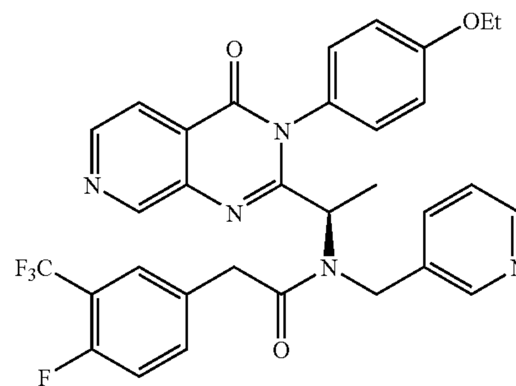
N-{1-[3-(4-Ethoxy-phenyl)-4-oxo-3,4-dihydro-pyrido[3,4-d]pyrimidin-2-yl]-ethyl}-2-(4-fluoro-3-trifluoromethyl-phenyl)-N-pyridin-3-ylmethyl-acetamide 3.56
