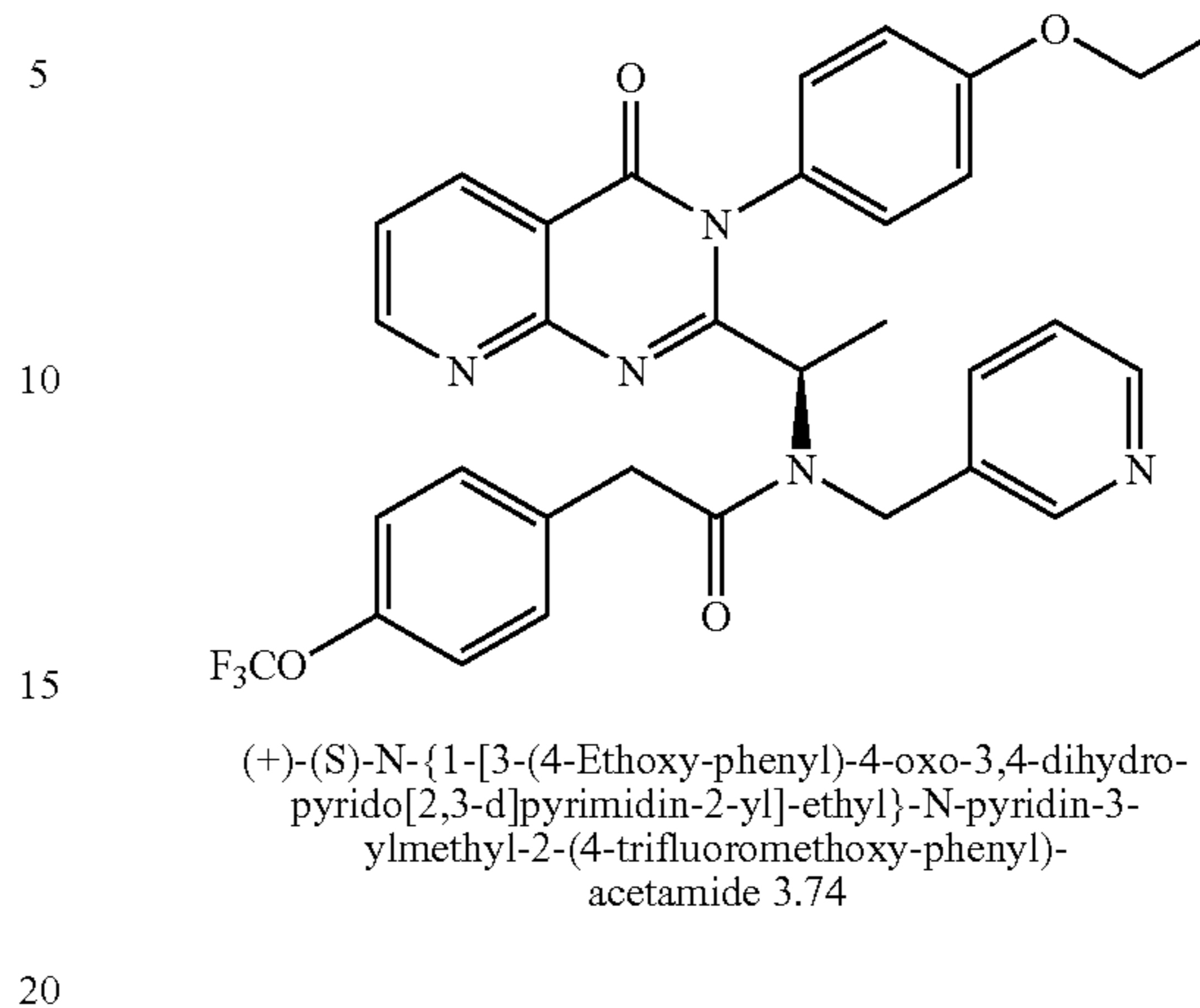
Synthesis of Compound 3.74
