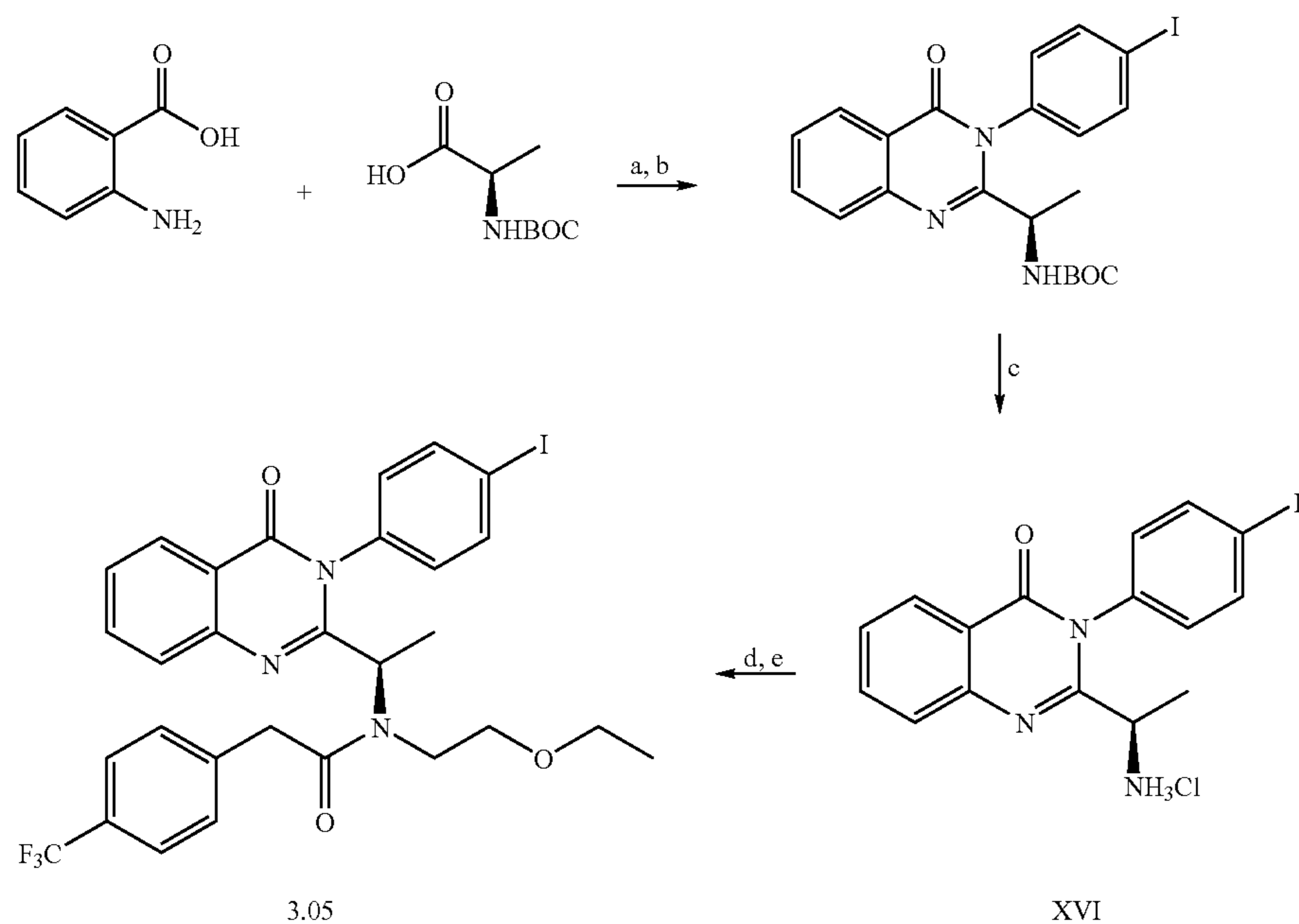
Scheme 5
