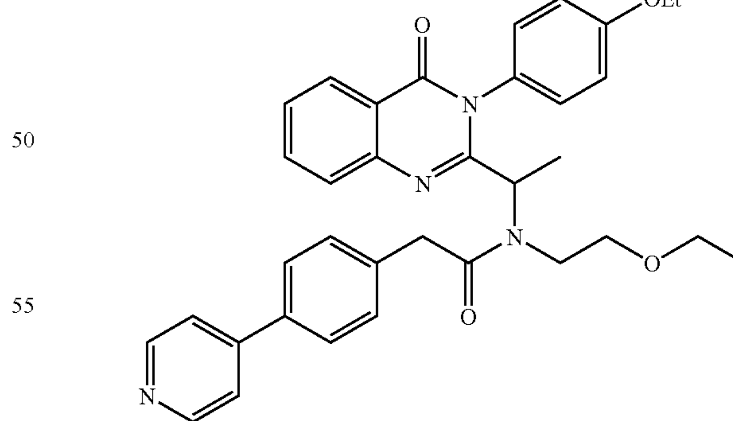
N-(2-Ethoxy-ethyl)-N-{1-[3-(4-ethoxy-phenyl)-4-oxo-3,4-dihydro-quinazolin-2-yl]-ethyl}-2-(4-pyridin-4-yl-phenyl)-acetamide 1.53
