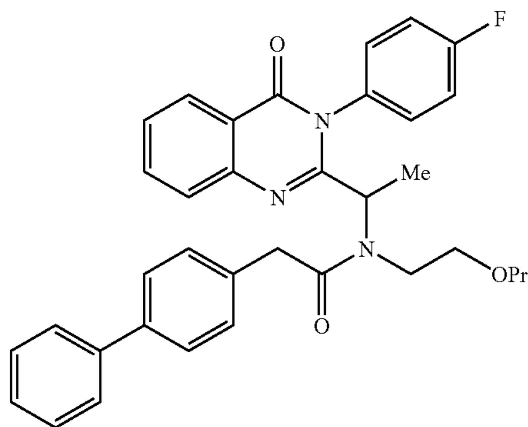
Synthesis of Compound 1.21
