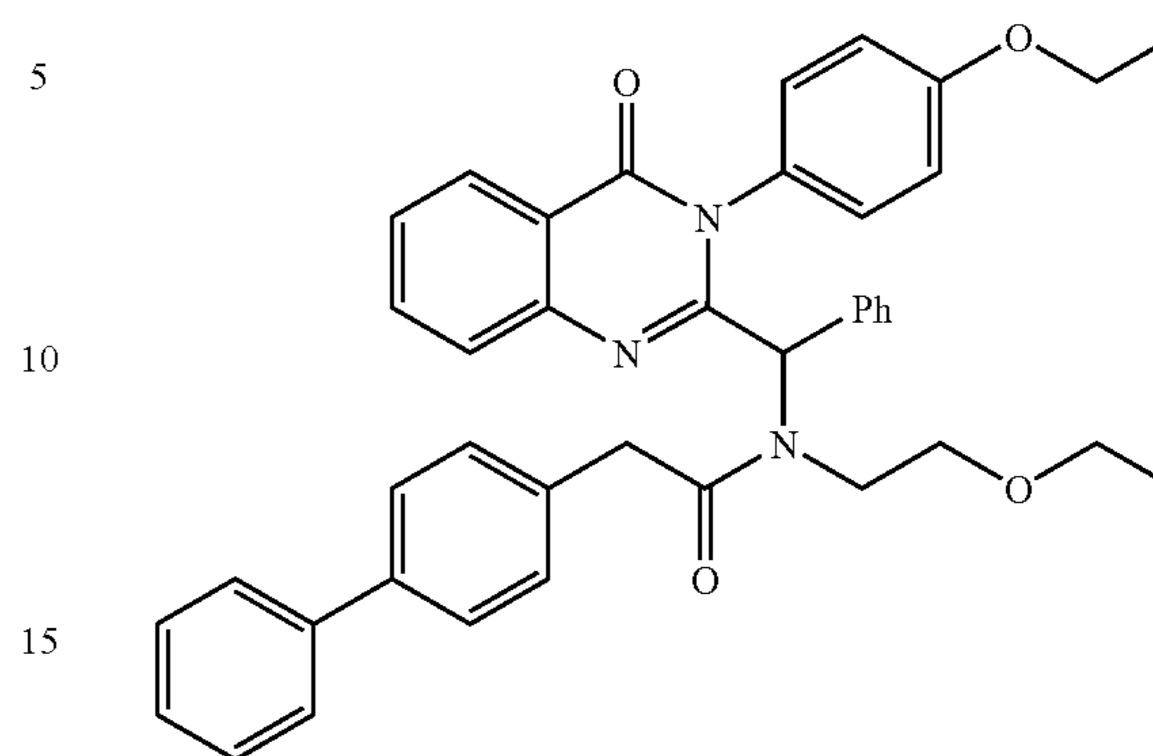
2-Biphenyl-4-yl-N-(2-ethoxy-ethyl)-N-{[3-(4-ethoxy-phenyl)-4-oxo-3,4-dihydro-quinazolin-2-yl]-phenyl-methyl}-acetamide 1.51
