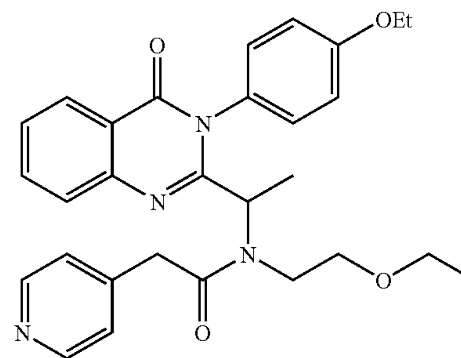
N-(2-Ethoxy-ethyl)-N-{1-[3-(4-ethoxy-phenyl)-4-oxo-3,4-dihydro-quinazolin-2-yl]-ethyl}-2-pyridin-4-yl-acetamide
