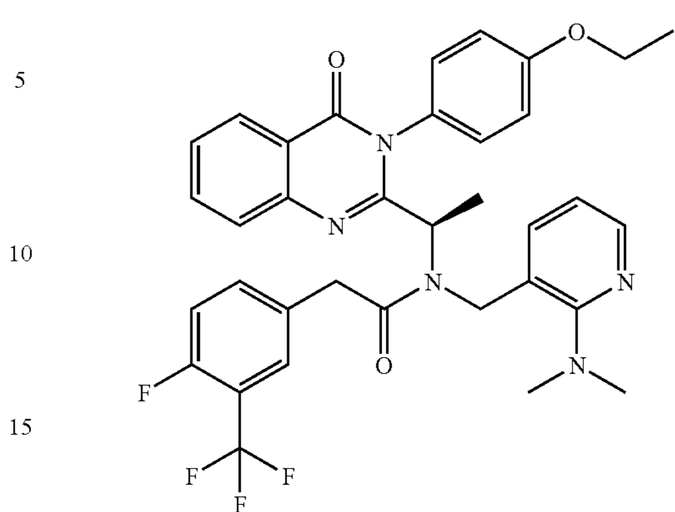
N-(2-Dimethylamino-pyridin-3-ylmethyl)-N-{1-[3-(4-ethoxy-phenyl)-4-oxo-3,4-dihydroquinazolin-2-yl]-ethyl}-2-(4-fluoro-3-trifluoromethyl-phenyl)-acetamide
