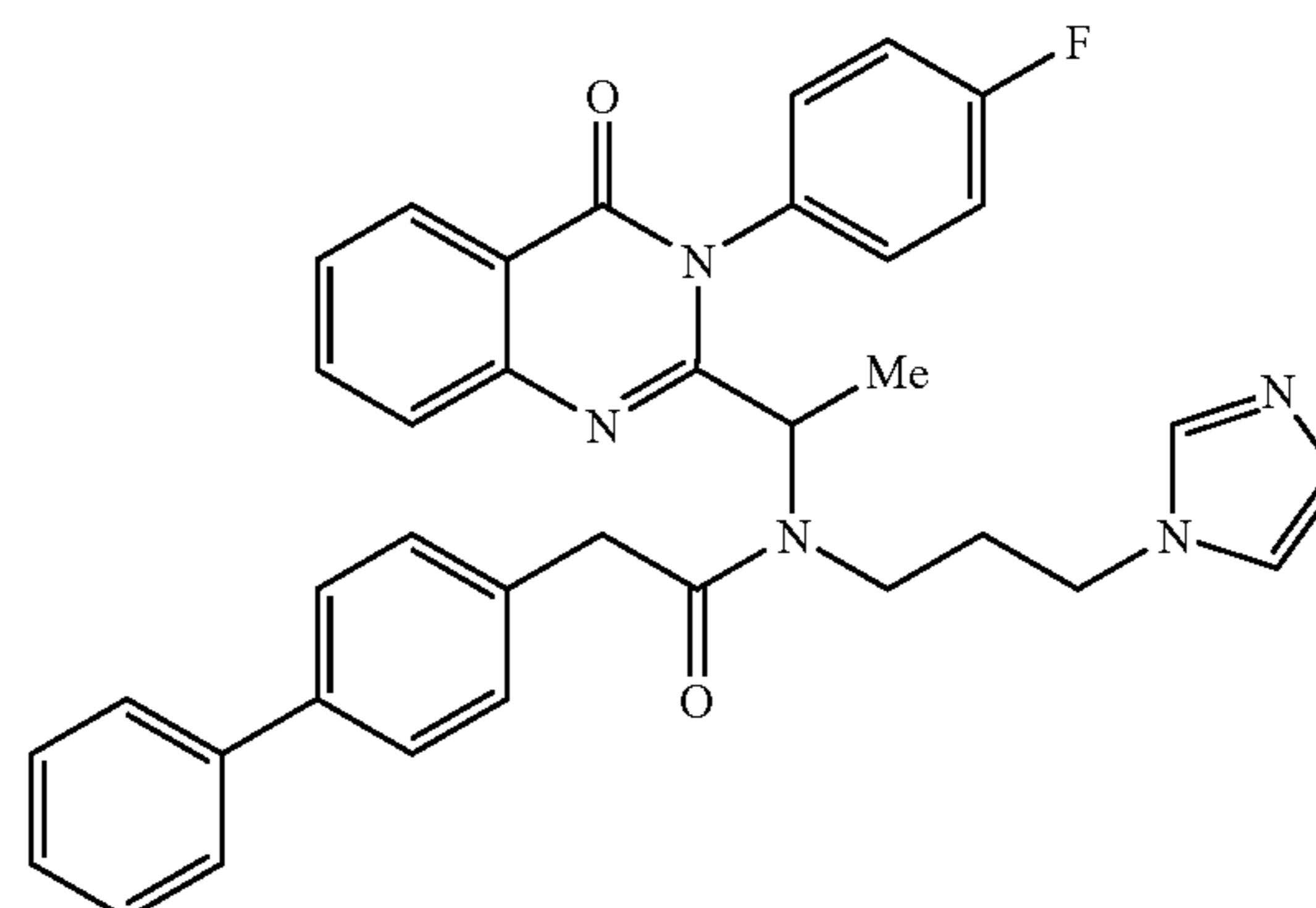
2-Biphenyl-4-yl-N-{1-[3-(4-fluoro-phenyl)-4-oxo-3,4-dihydro-quinazolin-2-yl]-ethyl}-N-(3-imidazol-1-yl-propyl)-acetamide
