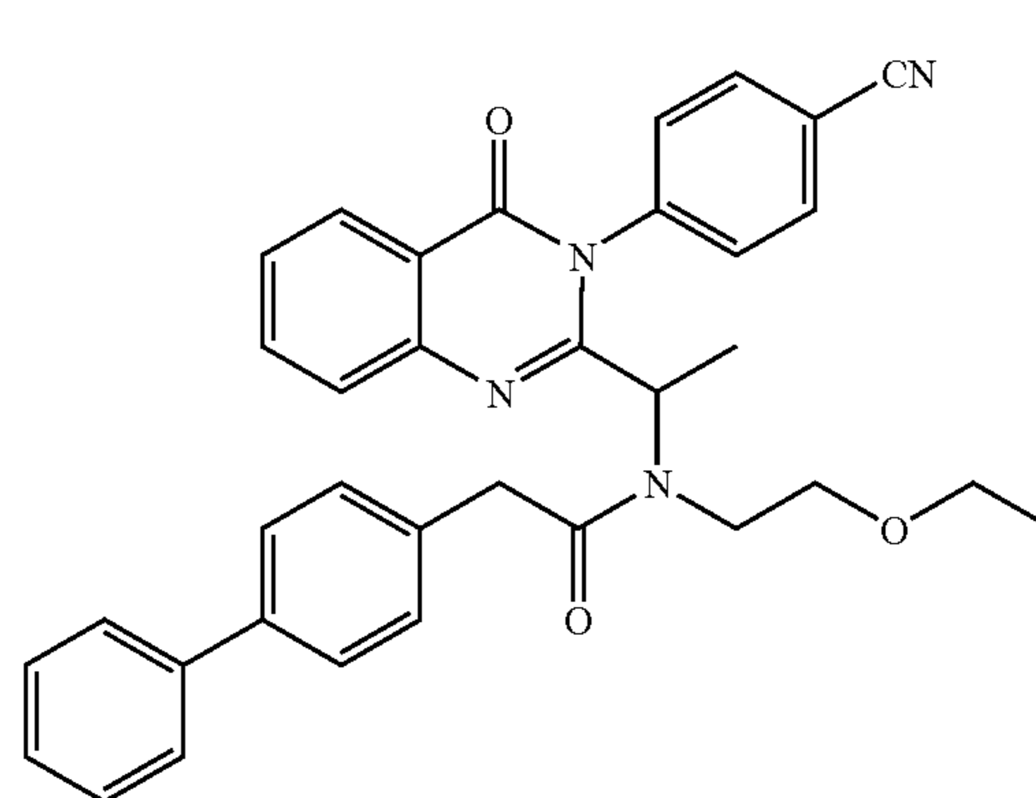
2-Biphenyl-4-yl-N-[1-[3-(4-cyano-phenyl)-4-oxo-3,4-dihydro-quinazolin-2-yl]-ethyl]-N-(2-ethoxy-ethyl)-acetamide
