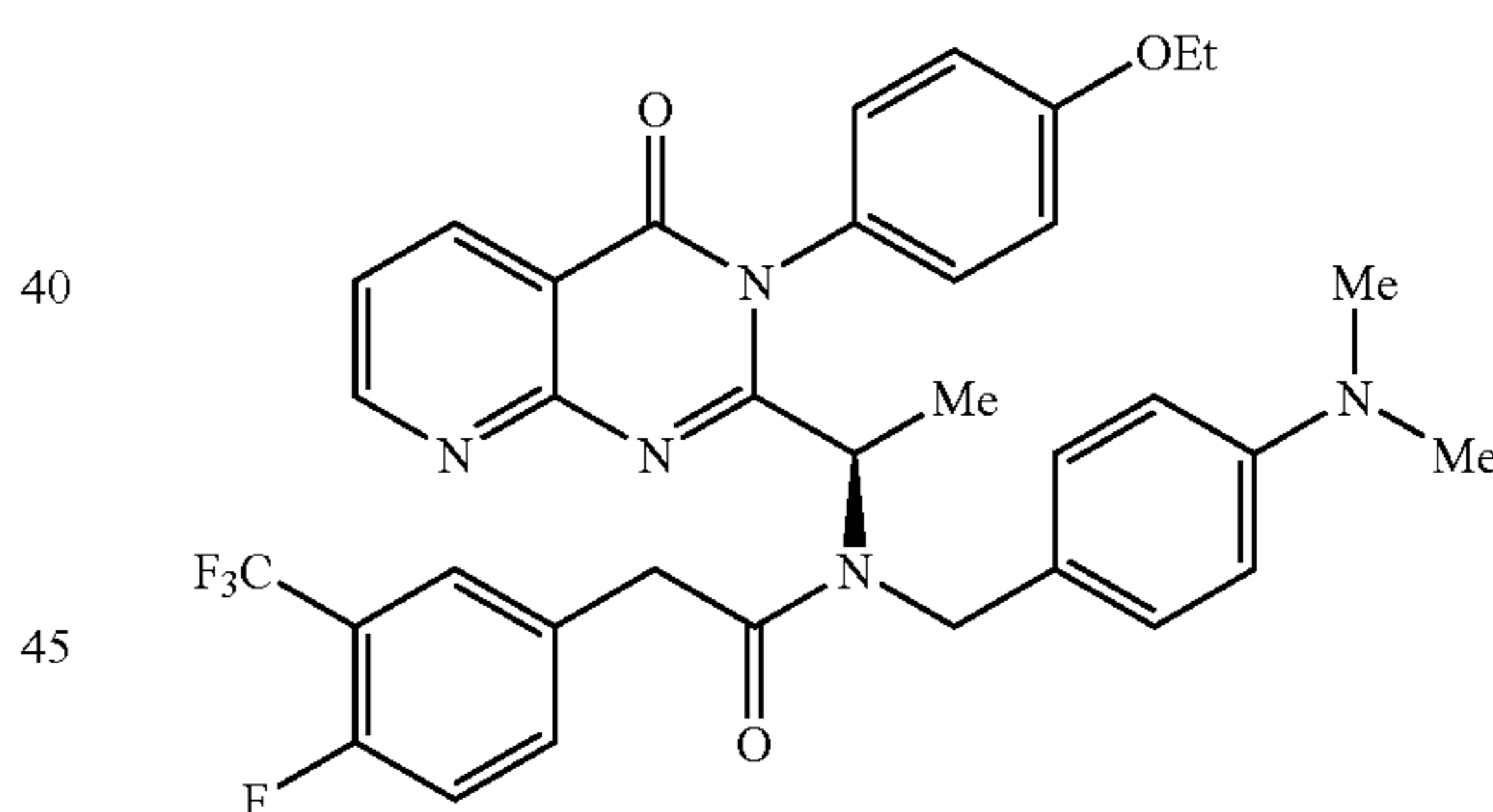
(R)-N-(4-Dimethylamino-benzyl)-N-(1-[3-(4-ethoxy-phenyl)-4-oxo-3,4-dihydro-pyrido[2,3-d]pyrimidin-2-yl]-ethyl)-2-(4-fluoro-3-trifluoromethyl-phenyl)-acetamide 3.68
