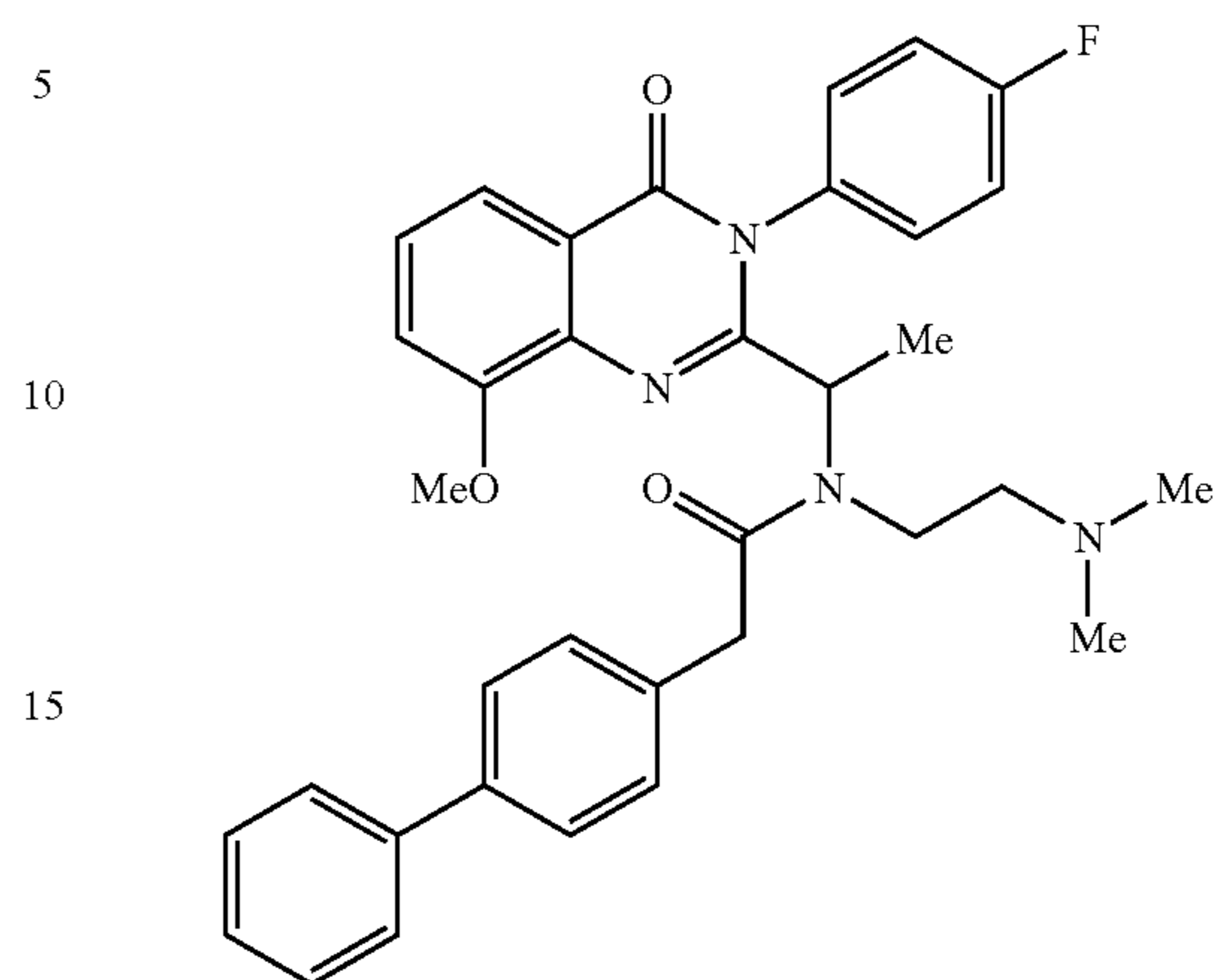
2-Biphenyl-4-yl-N-(2-dimethylamino-ethyl)-N-{1-[3-(4-fluoro-phenyl)-8-methoxy-4-oxo-3,4-dihydro-quinazolin-2-yl]-ethyl}-acetamide 2.02
