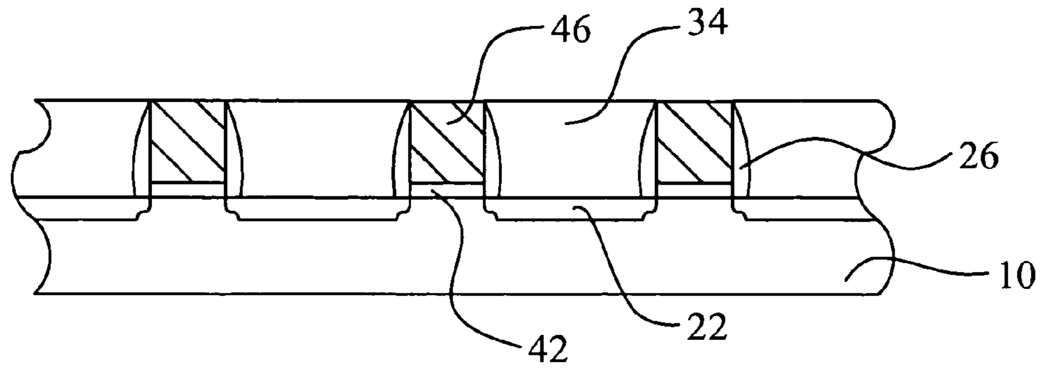
FIG. 4 Prior Art
