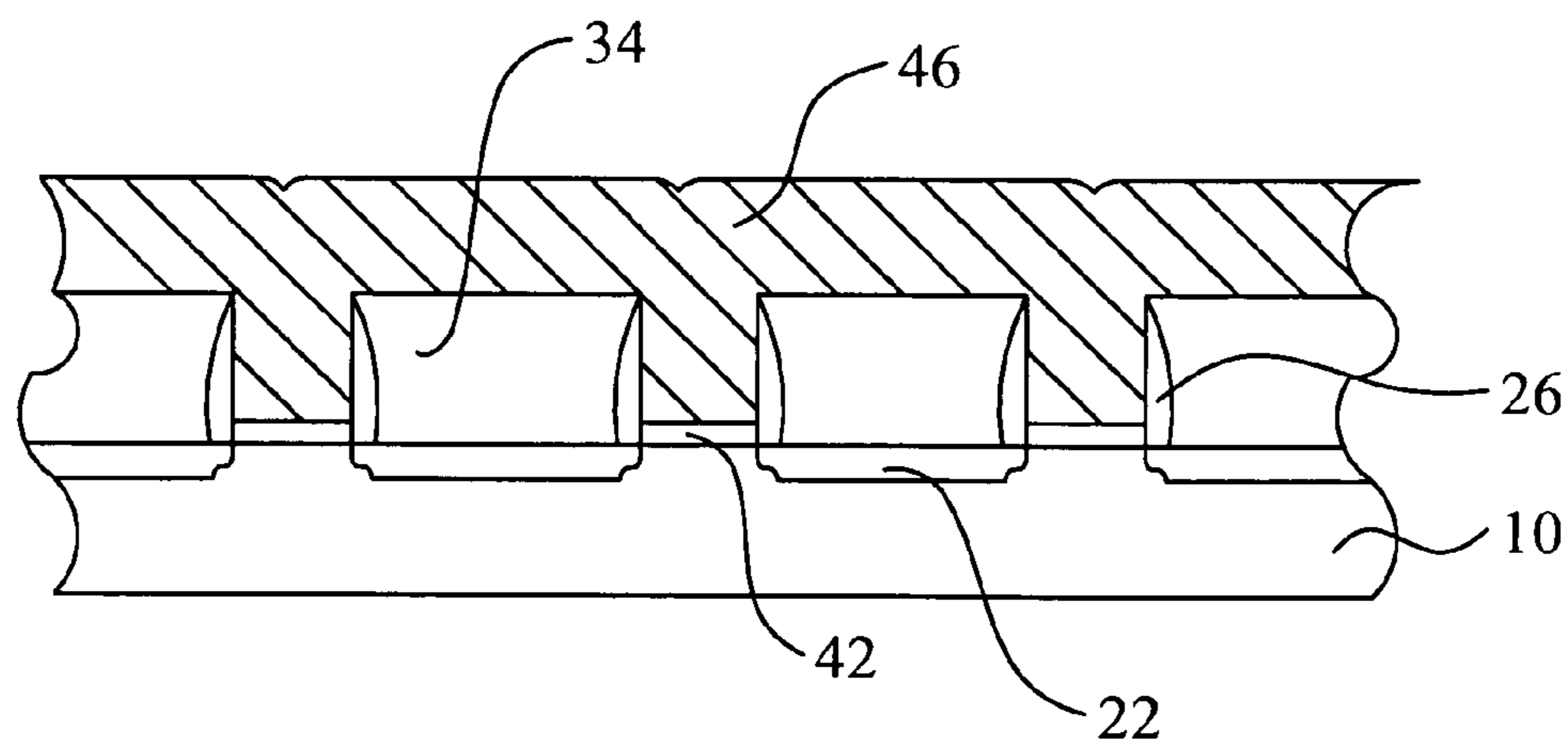
FIG. 3 Prior Art
