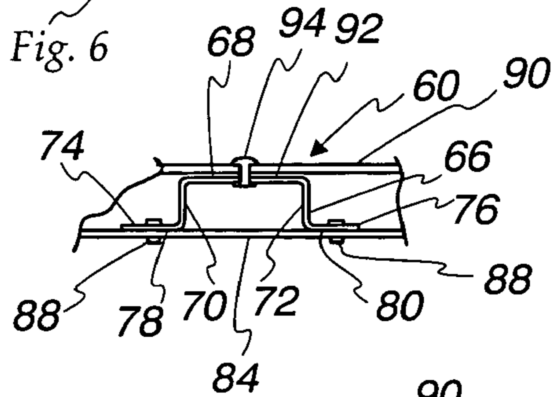
Fig. 6 (PRIOR ART)
