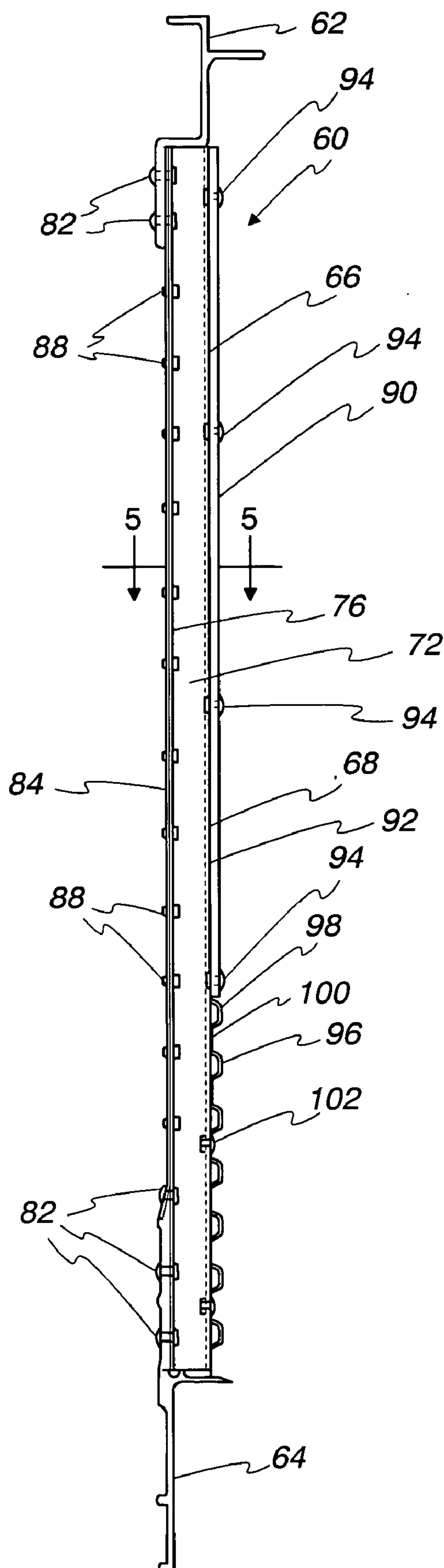
Fig. 4 (PRIOR ART)
