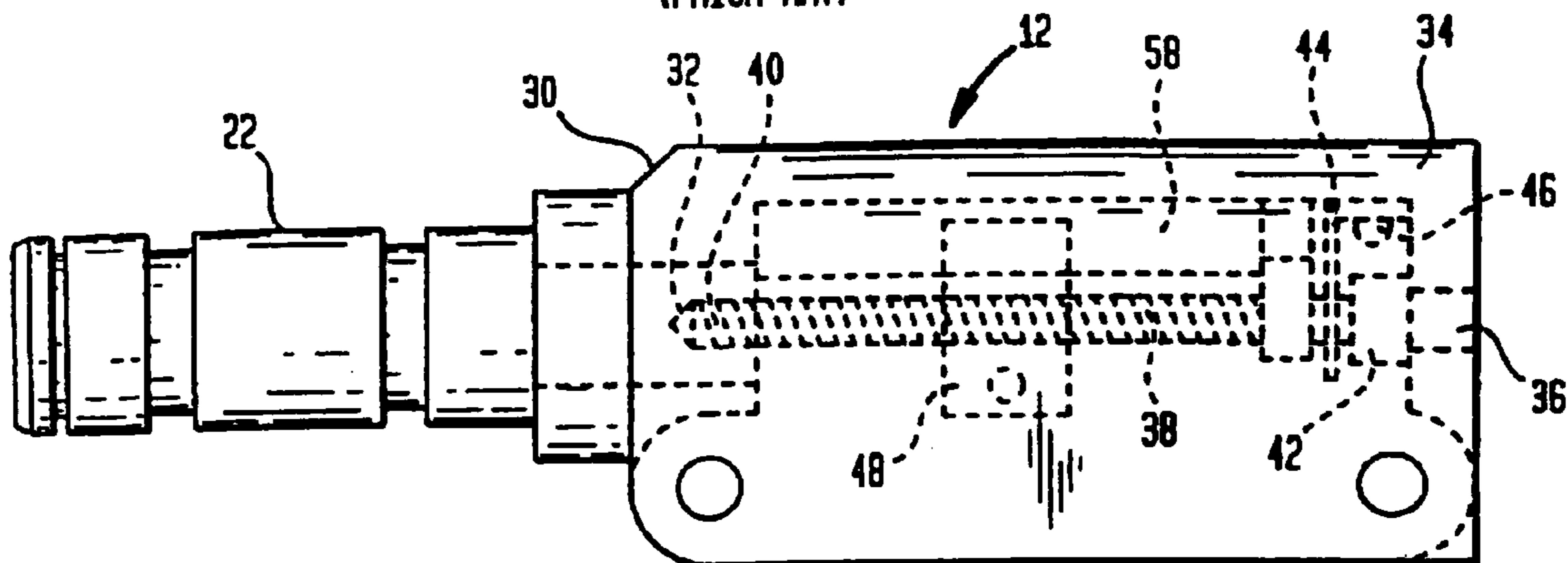
FIG. 2 (PRIOR ART)
