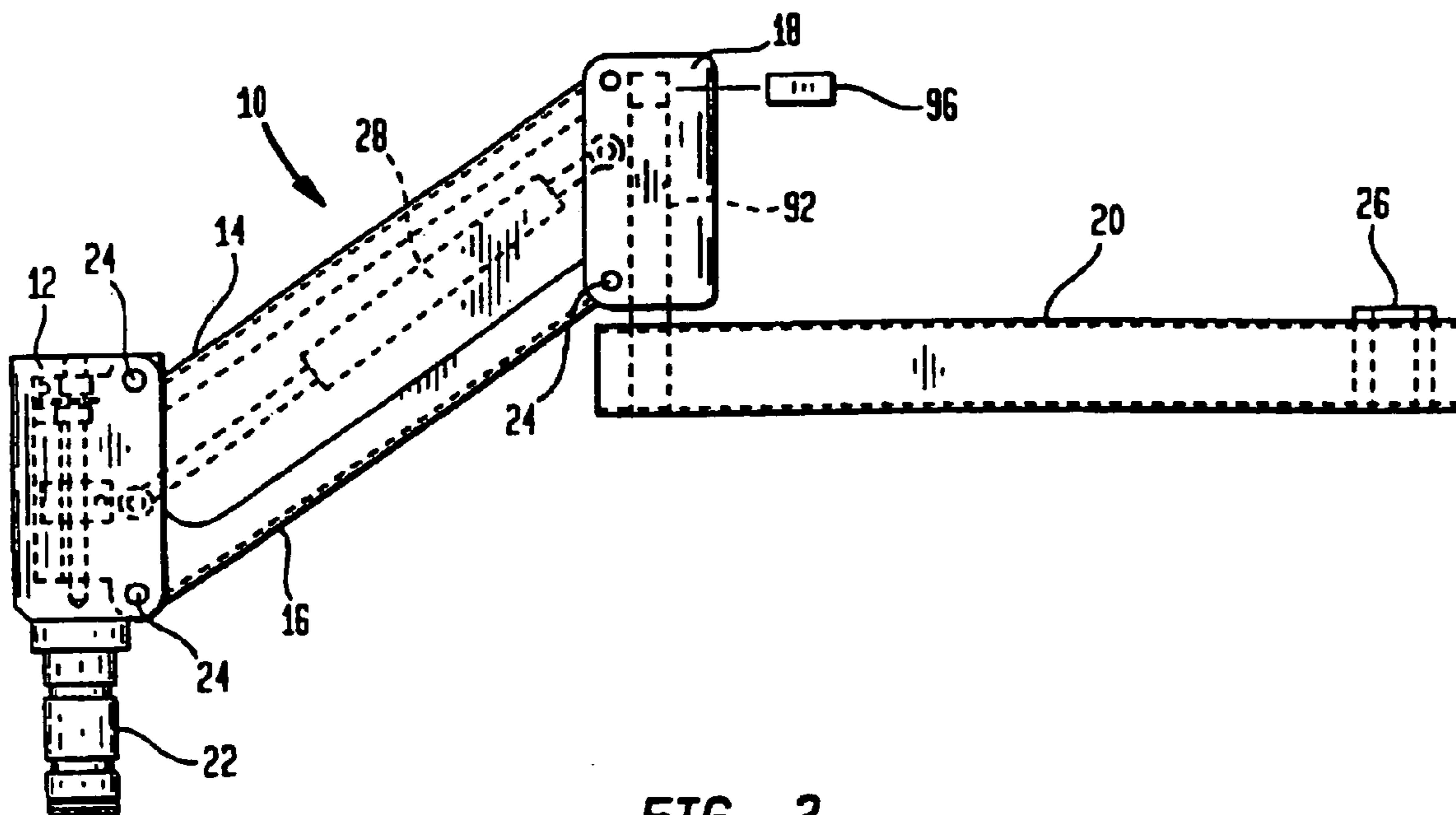
FIG. 1 (PRIOR ART)
