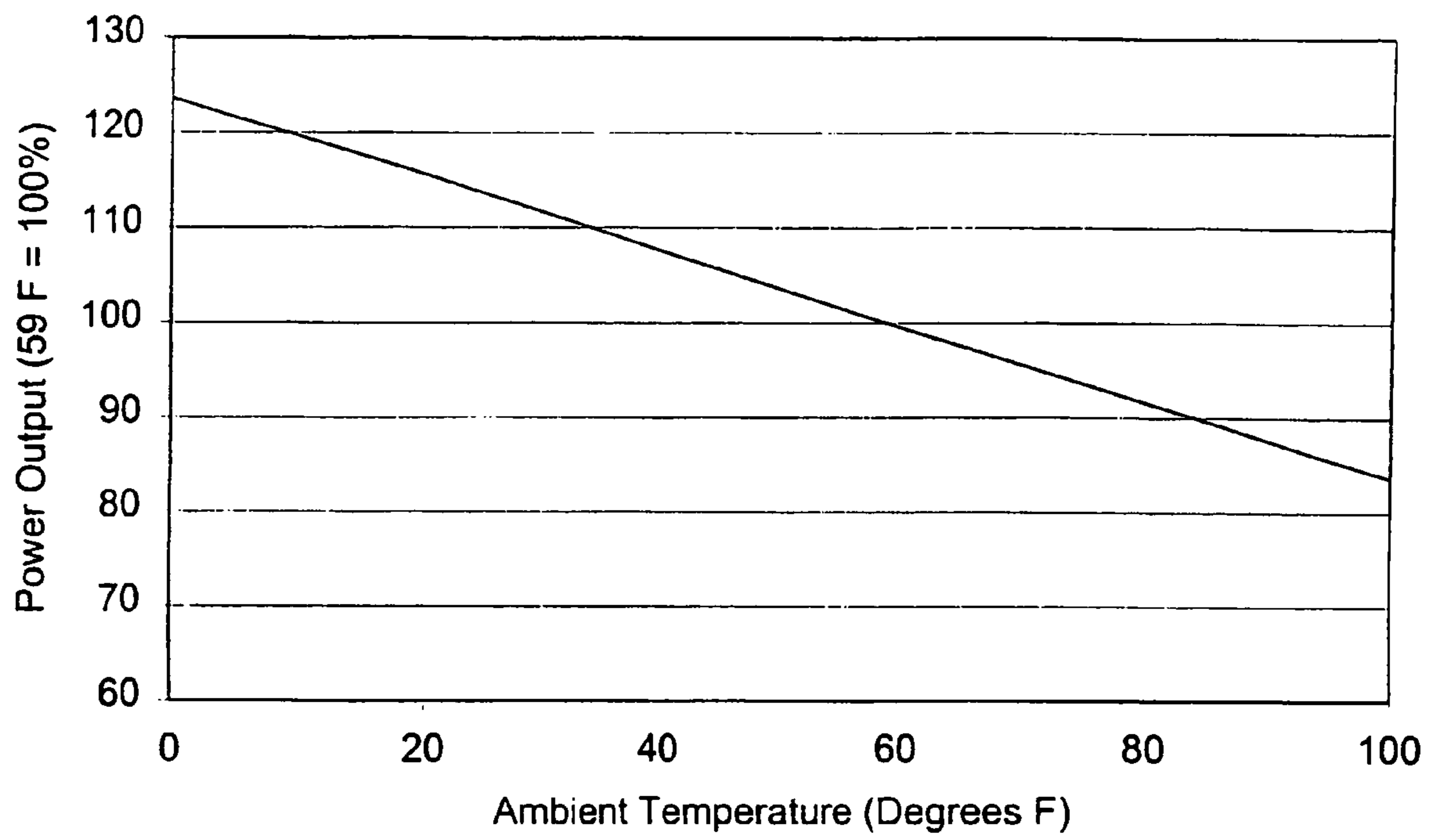
Turbine Capacity Versus Ambient Temperature
