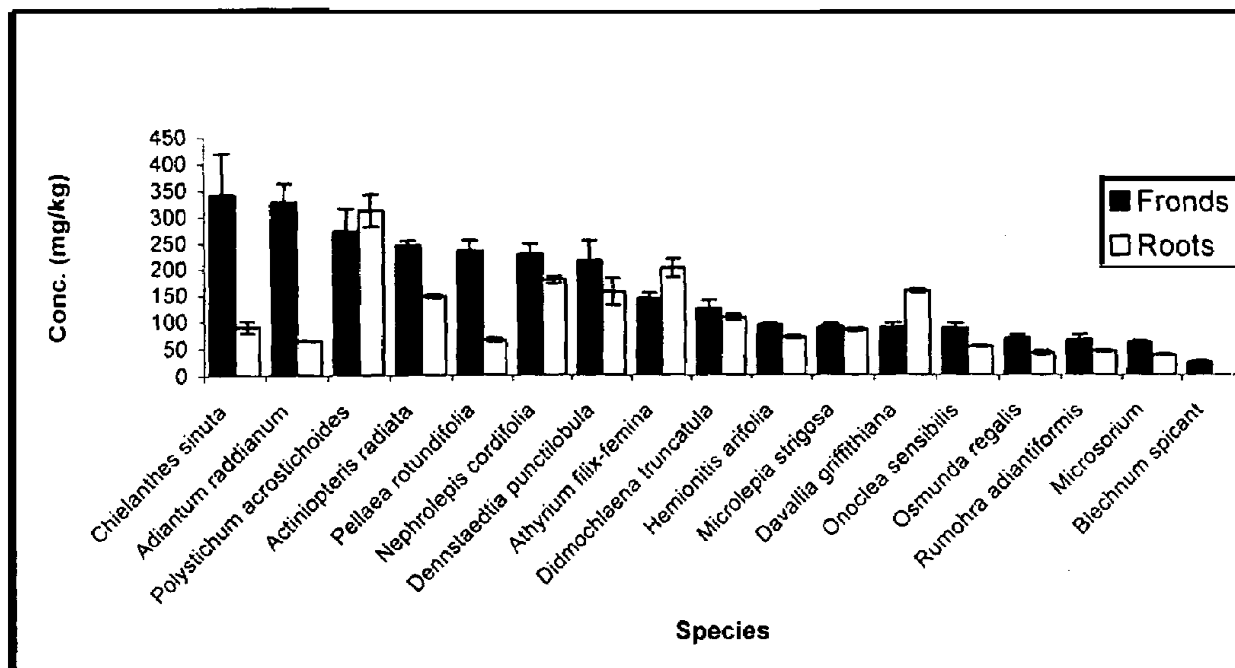
Fig.2. Arsenic concentrations in 17 non- Pteris ferns after exposing to 300 \mu M arsenate for 3d.
