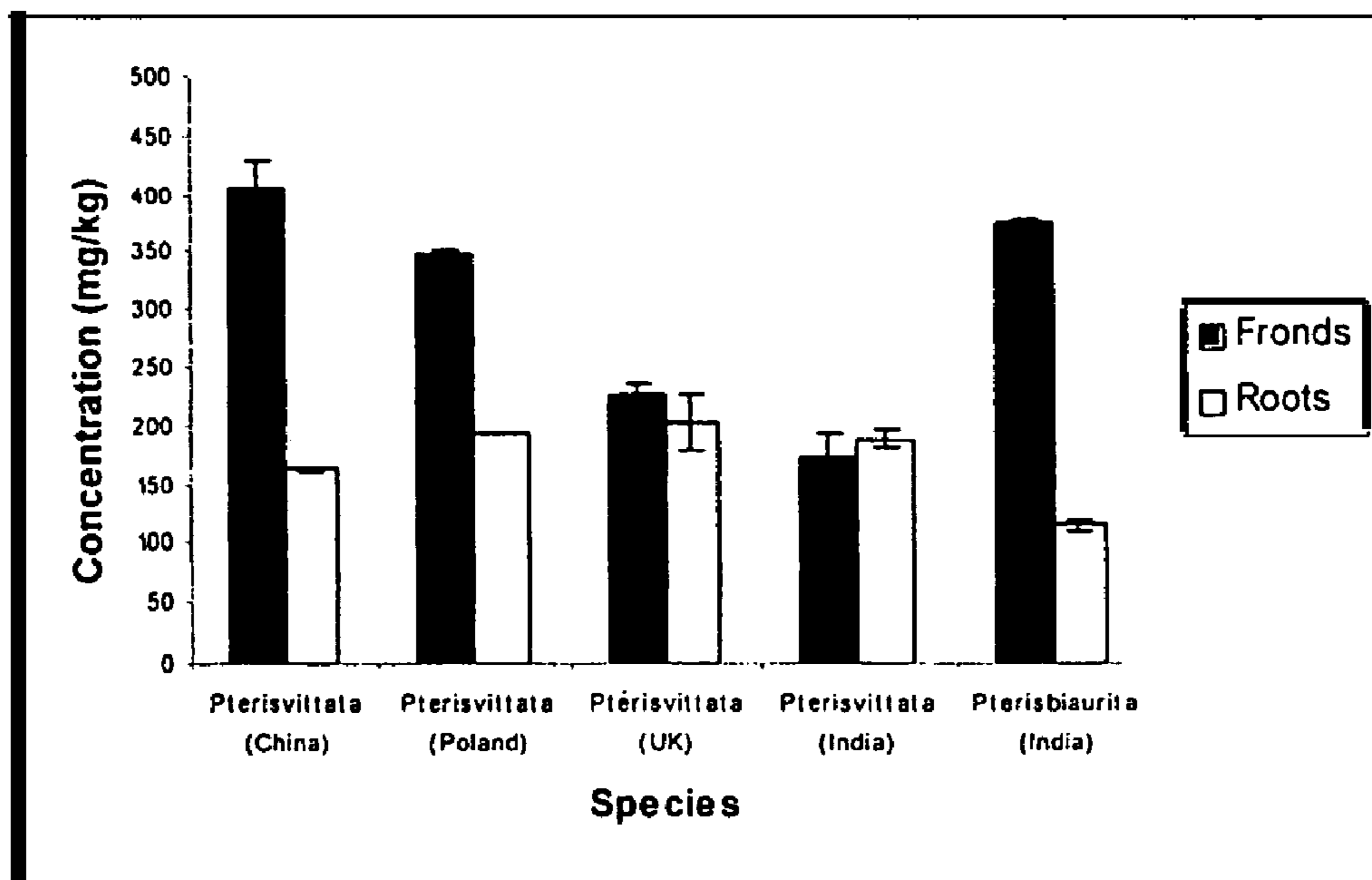
Fig.1. Arsenic concentrations in Pteris ferns from different locations after exposing to 300 \mu M arsenate for 3d.
