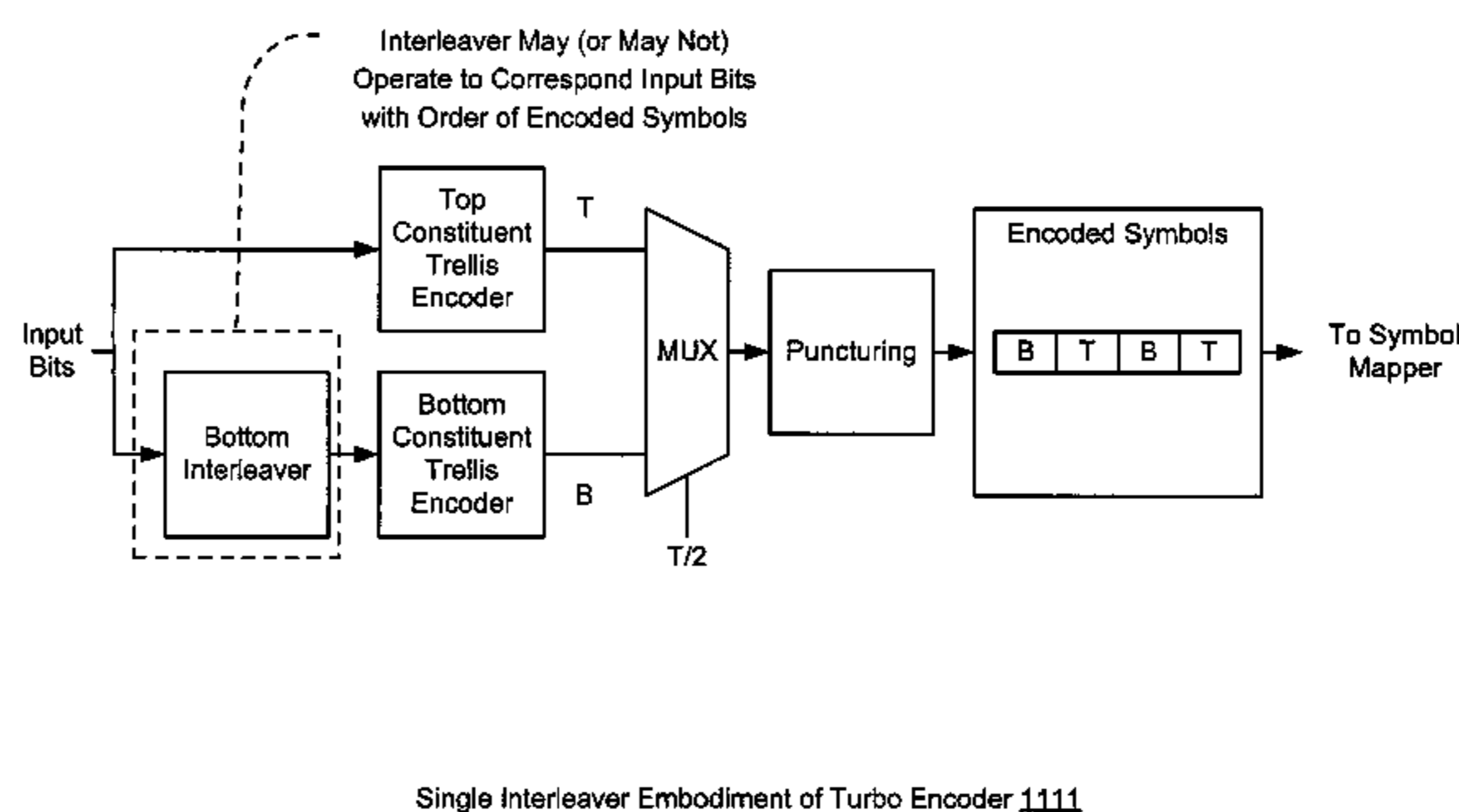
Single Interleaver Embodiment of Turbo Encoder 1111
