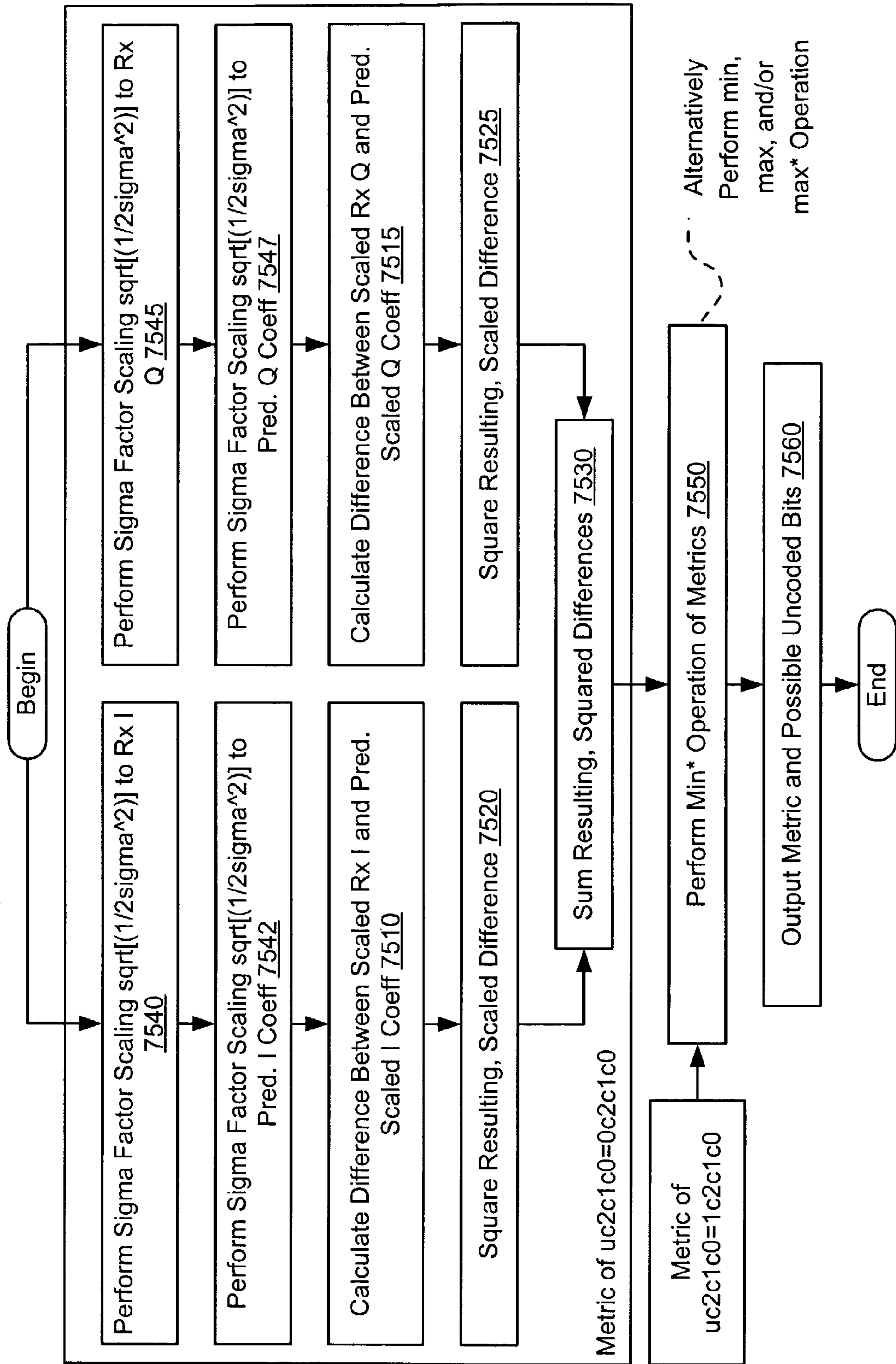
Metric Generator Method 7500
