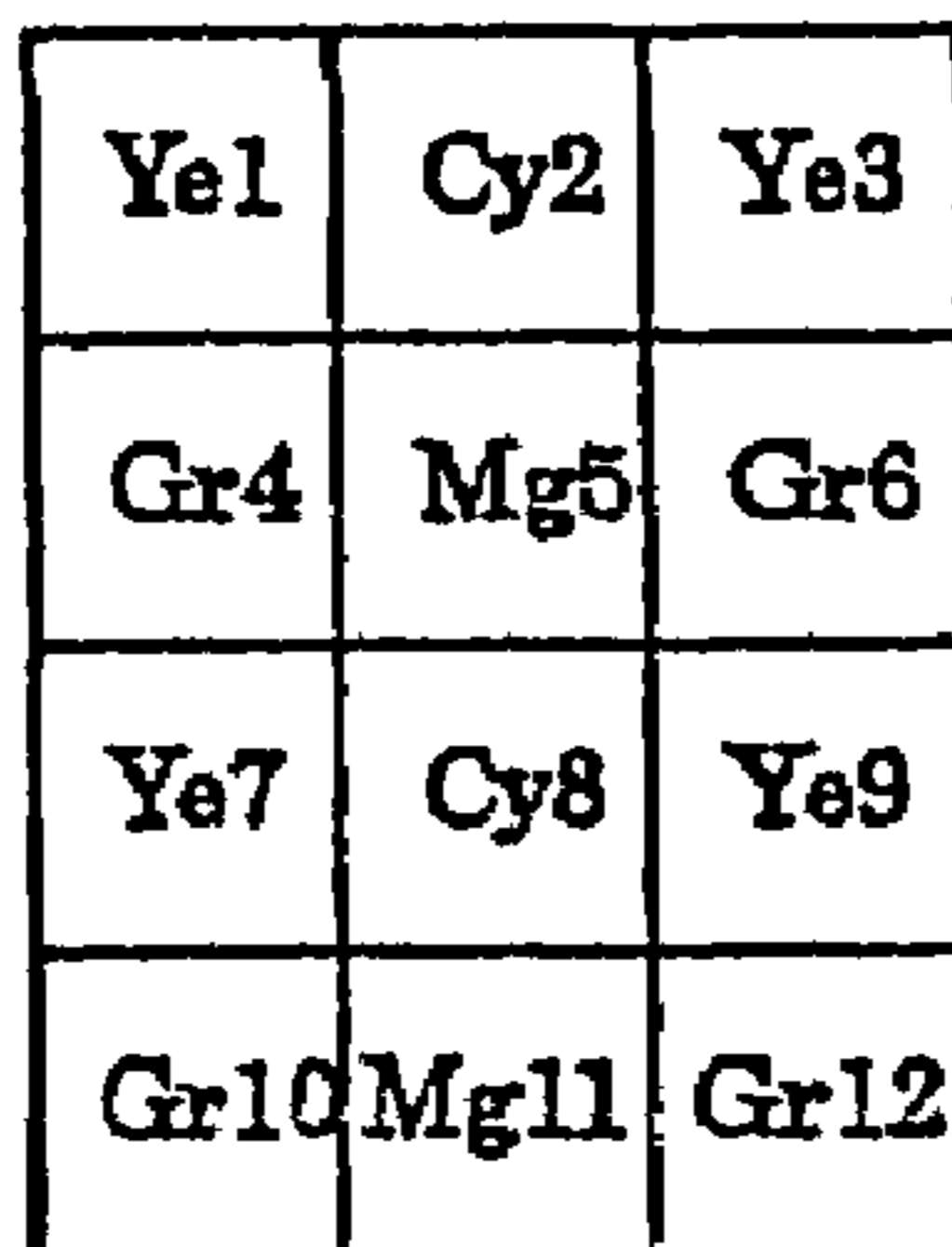
Part of color array of complementary-color filter of Fig.2
