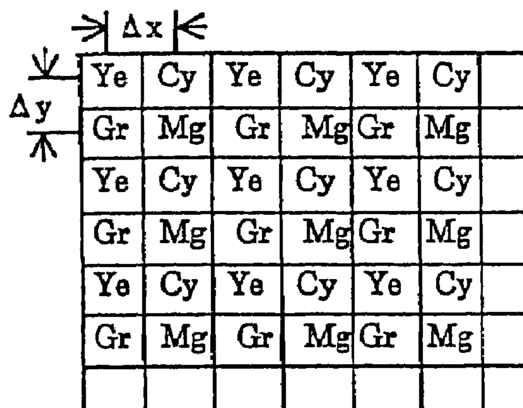
Color array of complementary-color filter
