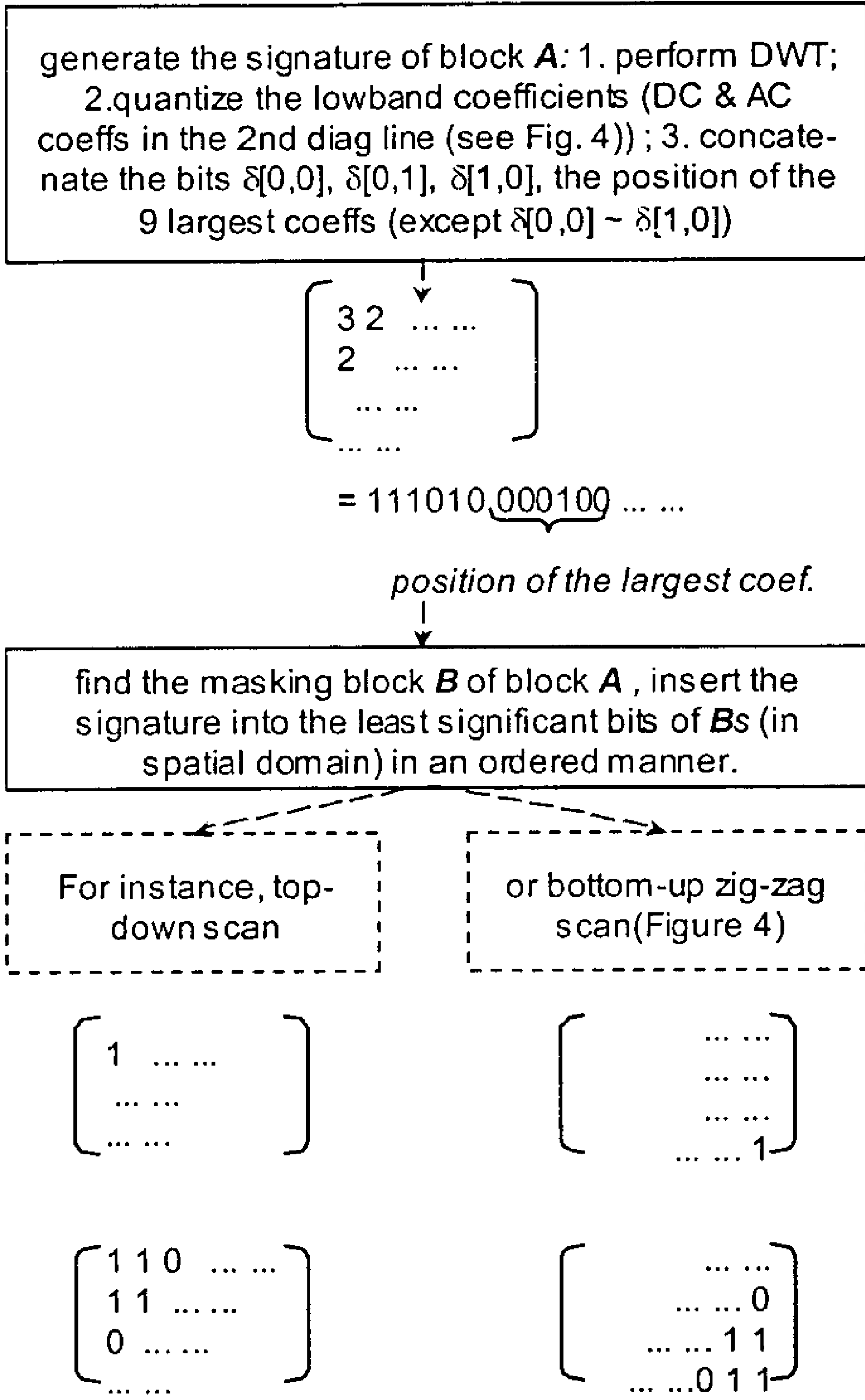
Fig 3. Embedding strategy
