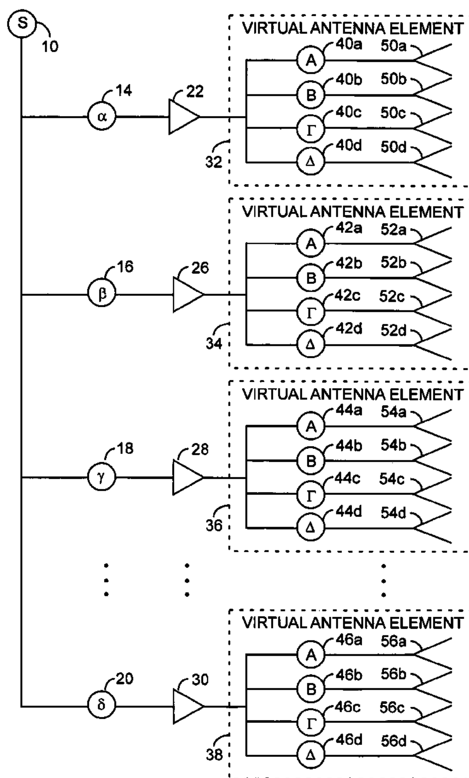
VIRTUAL ELEMENT SUBARRAY PHASED ARRAY ANTENNA SYSTEM
