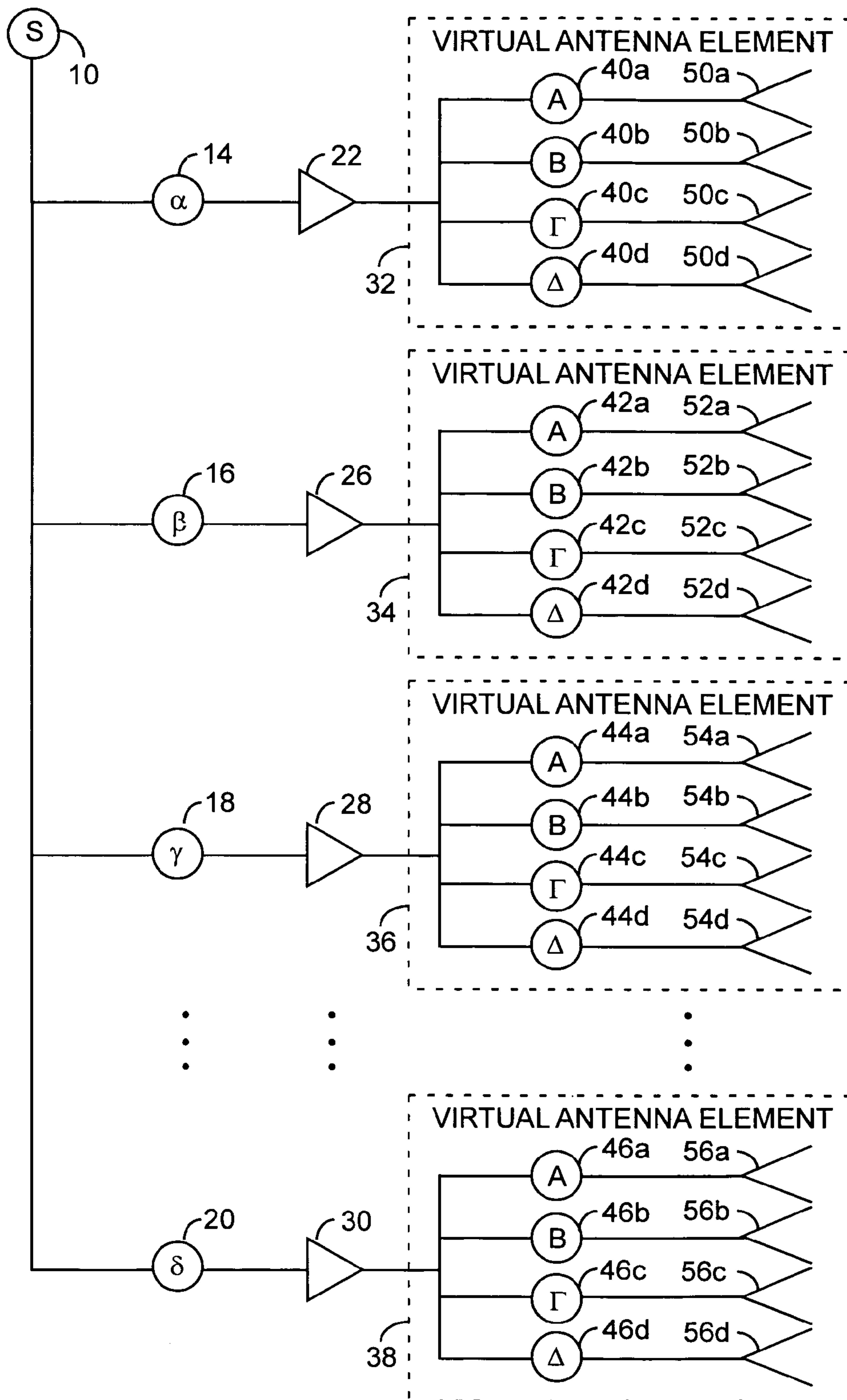
VIRTUAL ELEMENT SUBARRAY PHASED ARRAY ANTENNA SYSTEM
