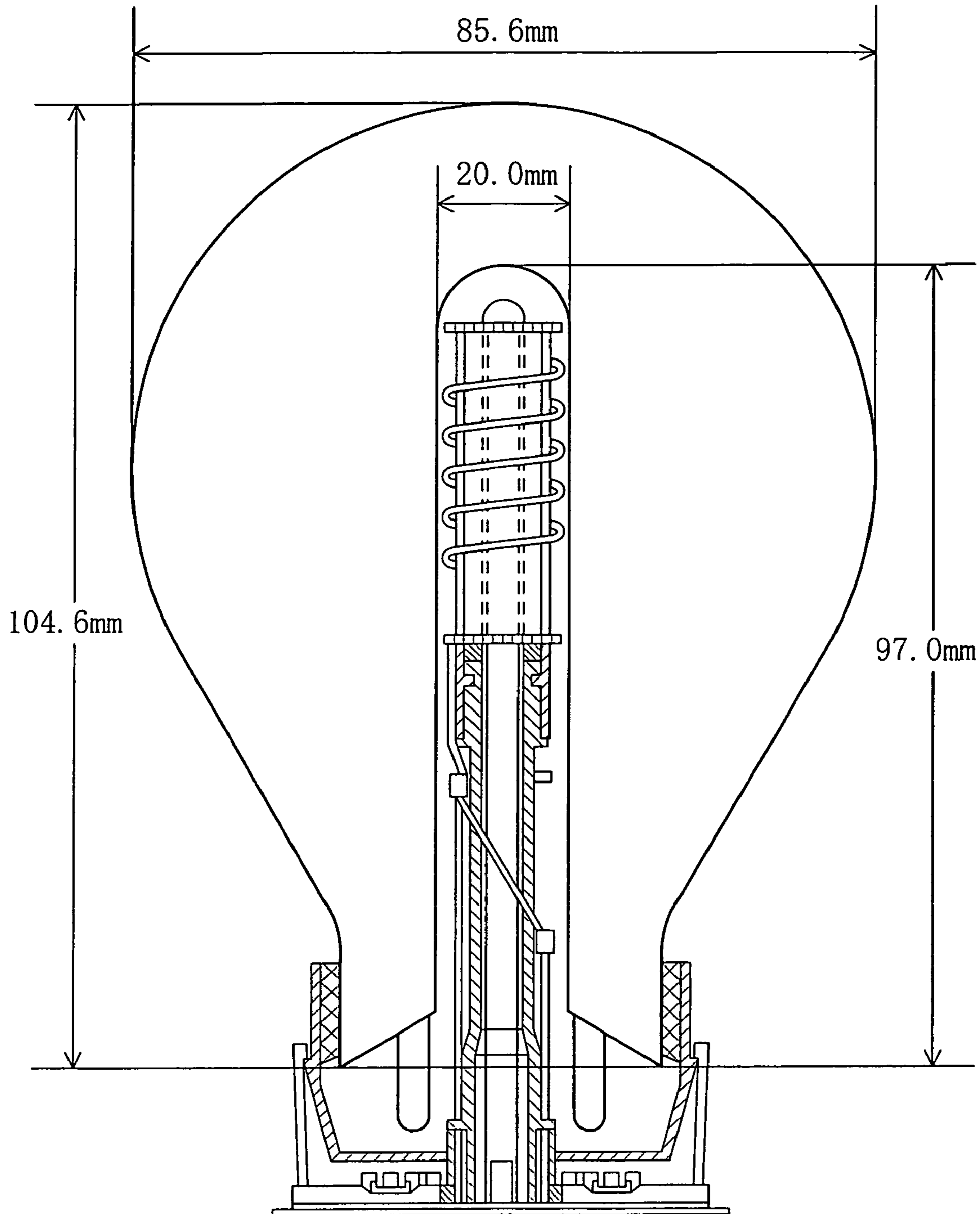
FIG. 12 PRIOR ART
