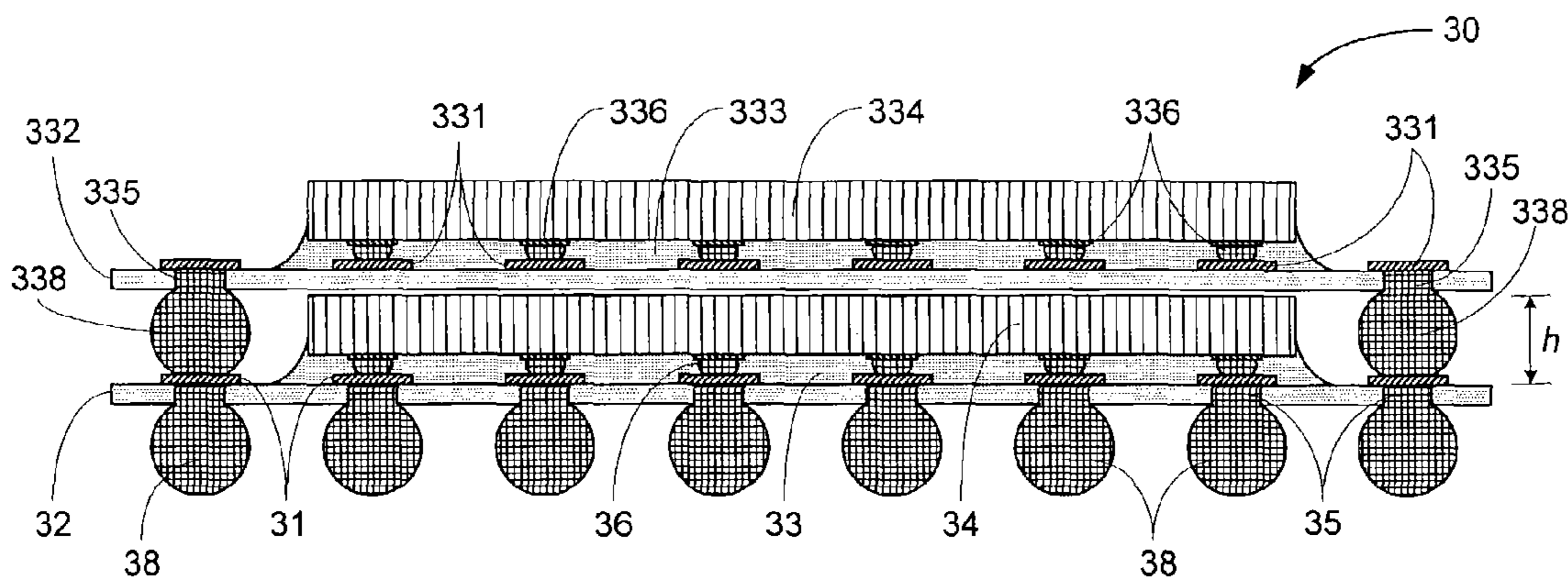
Fig. 3 PRIOR ART
