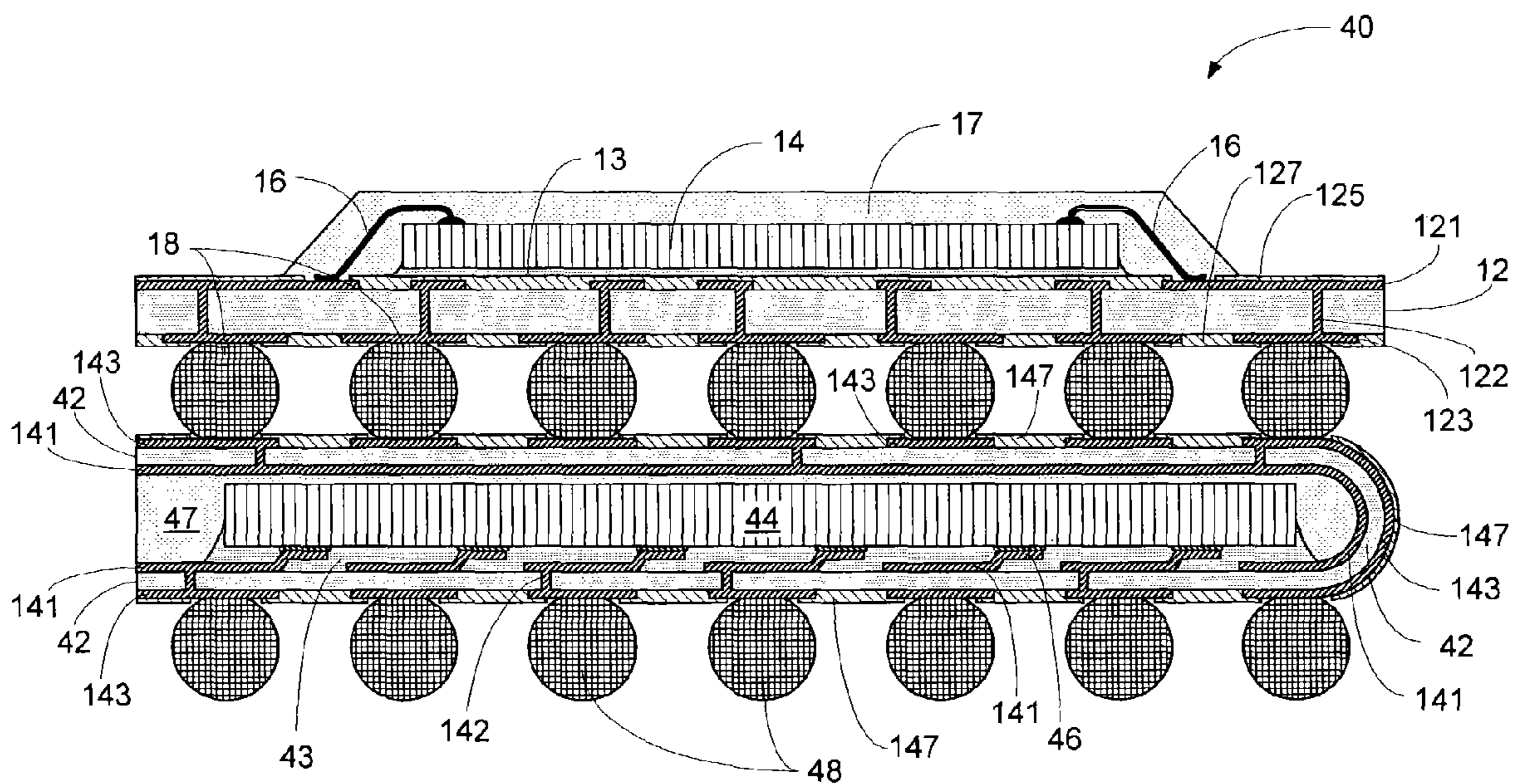
Fig. 4 PRIOR ART
