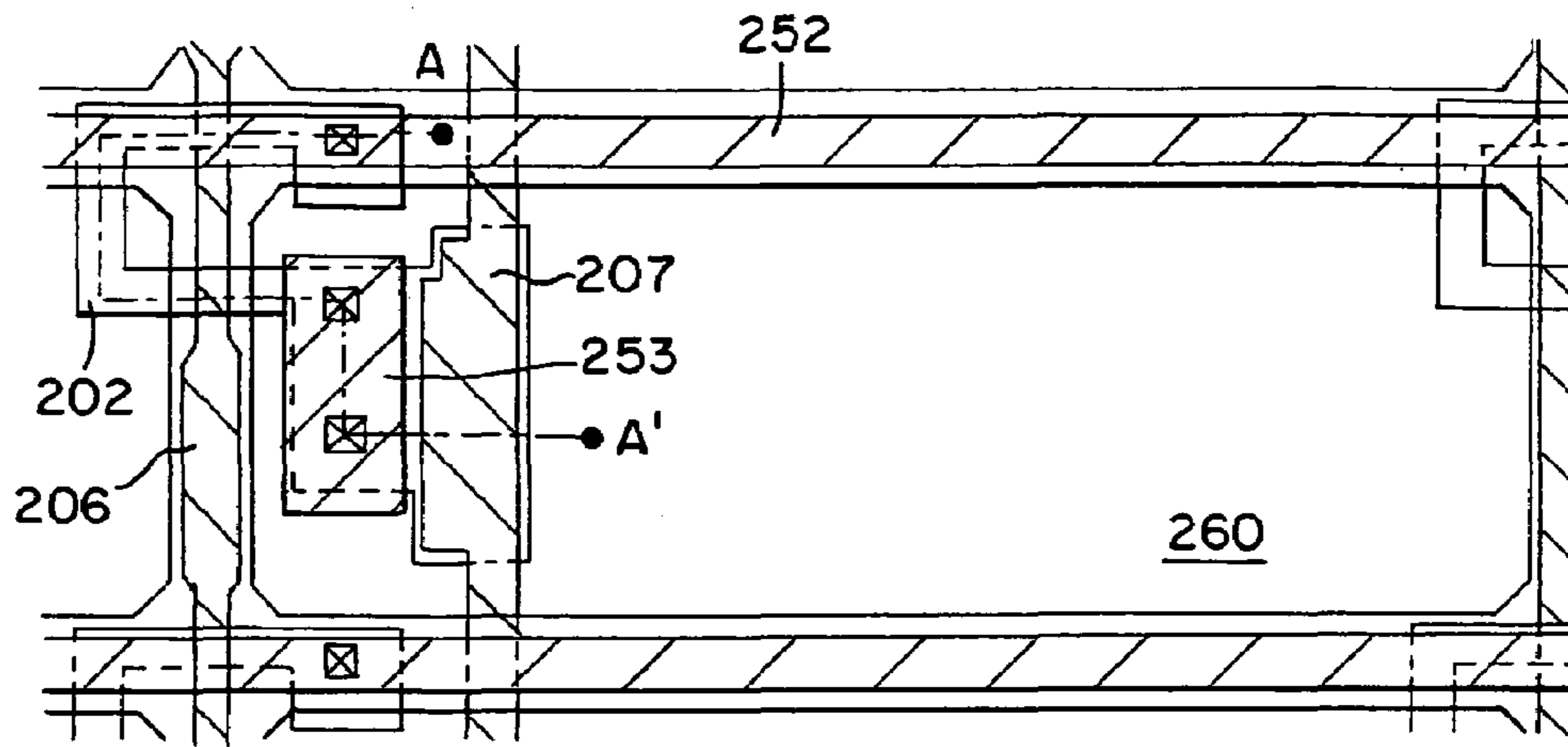
PLAN VIEW OF PIXEL MATRIX CIRCUIT
