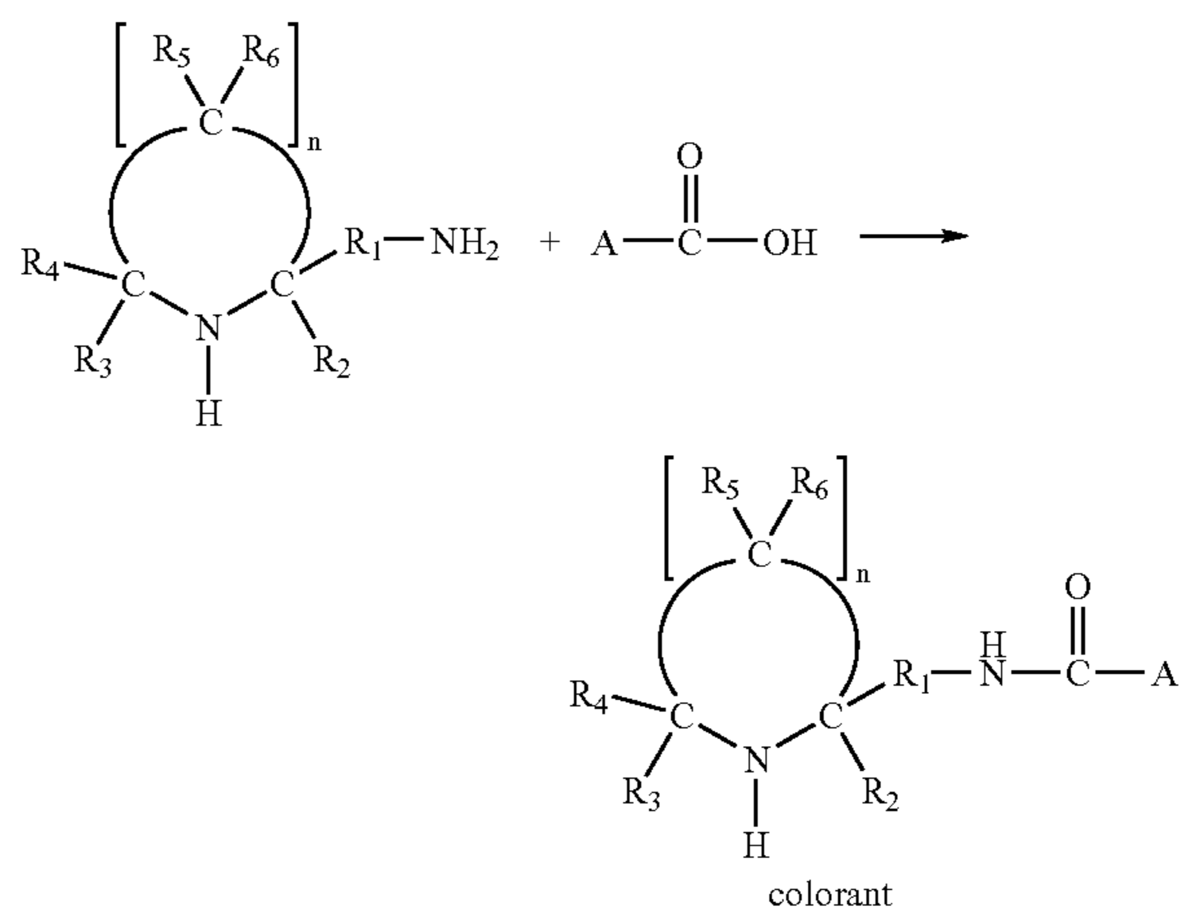
Scheme 3
