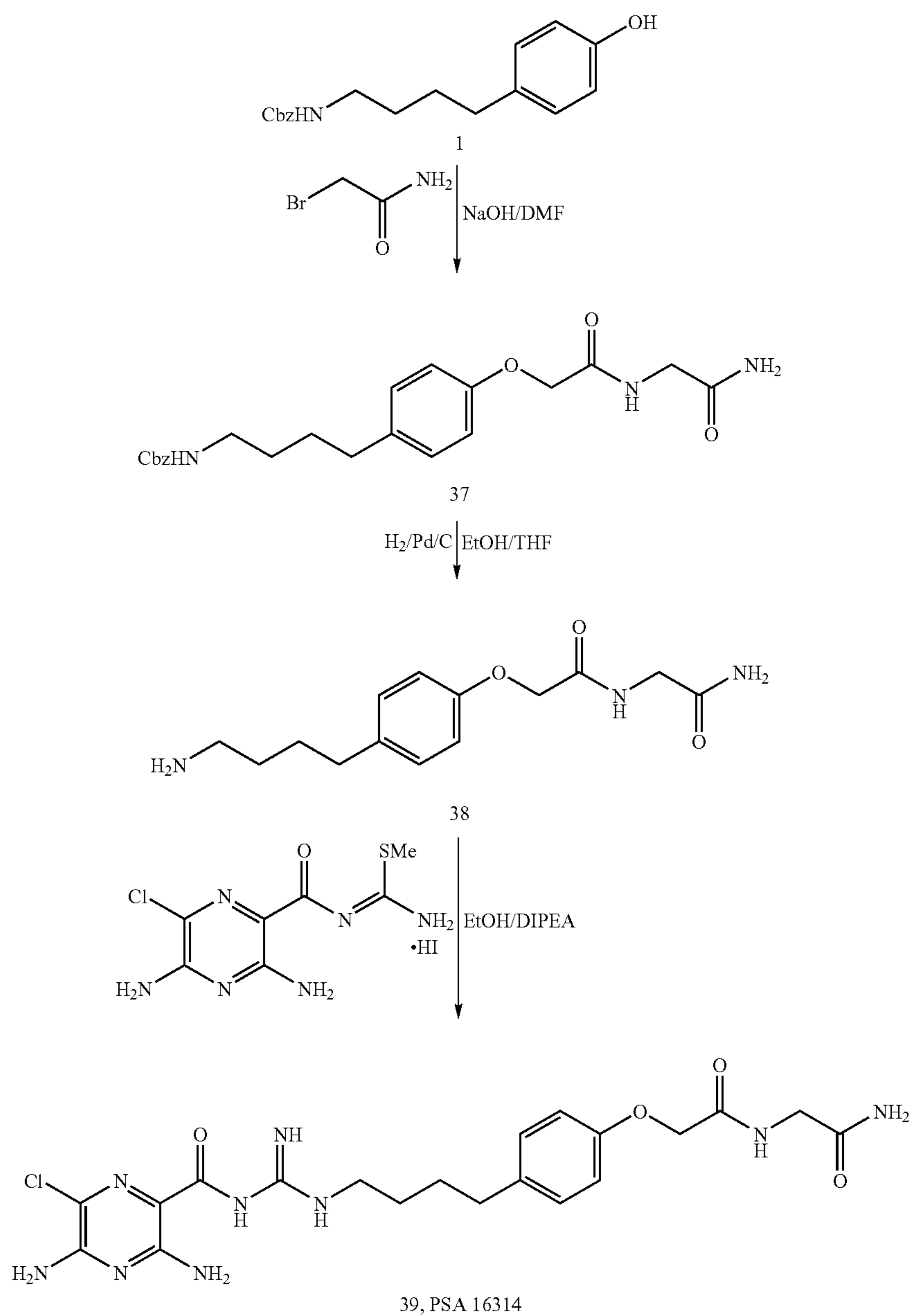
Scheme 9. Synthesis of PSA 16314
