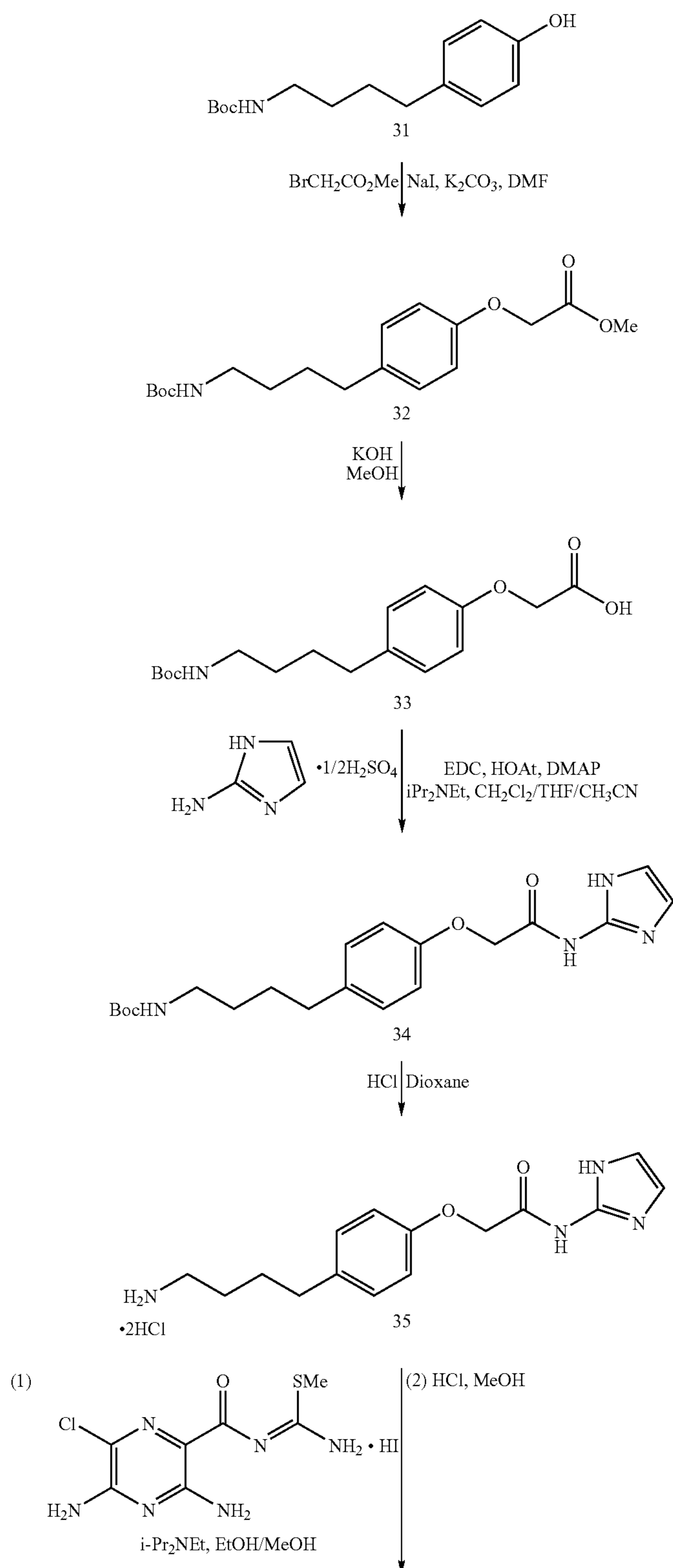
Scheme 8. Synthesis of PSA 16437
