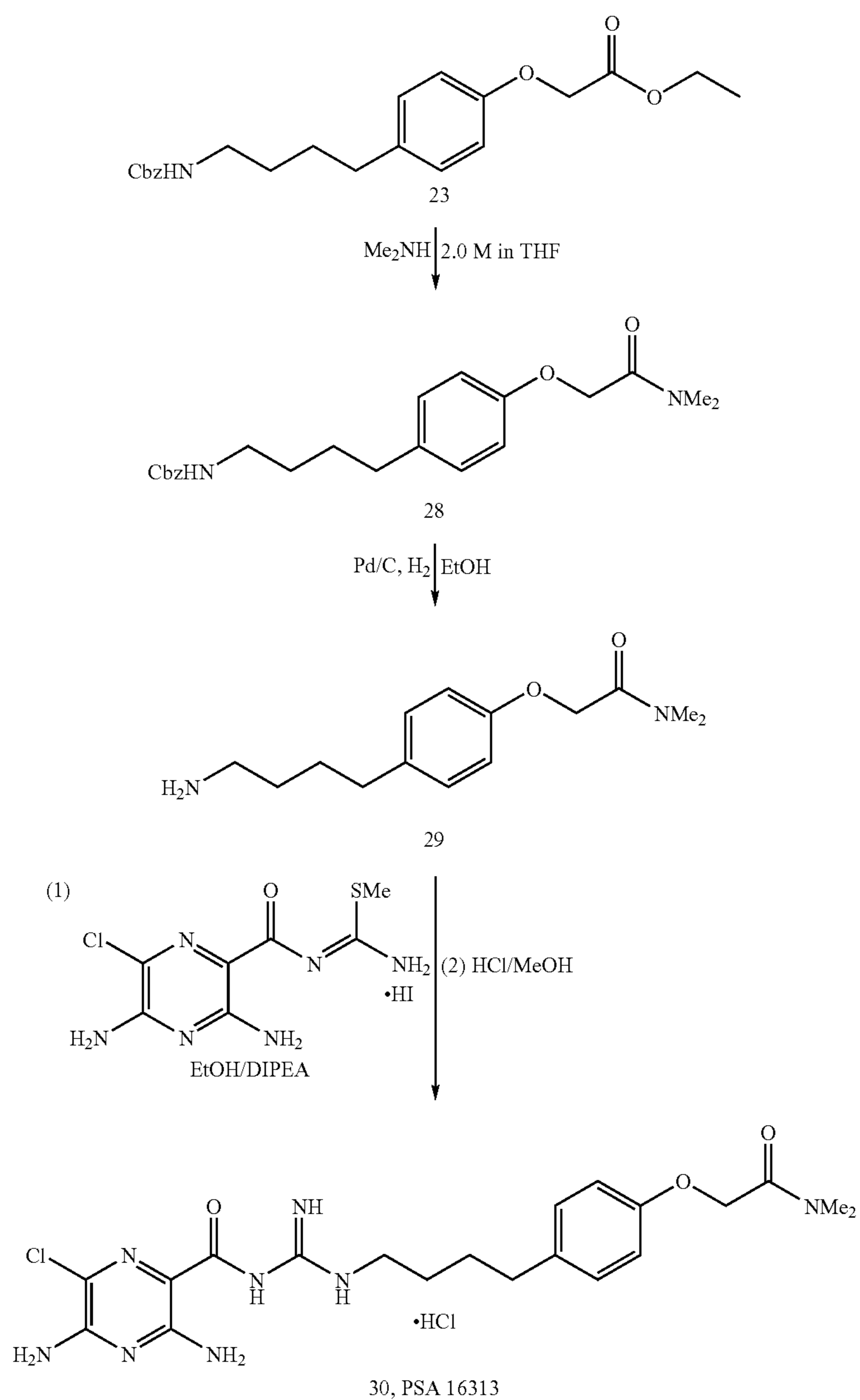
Scheme 7. Synthesis of PSA 16313
