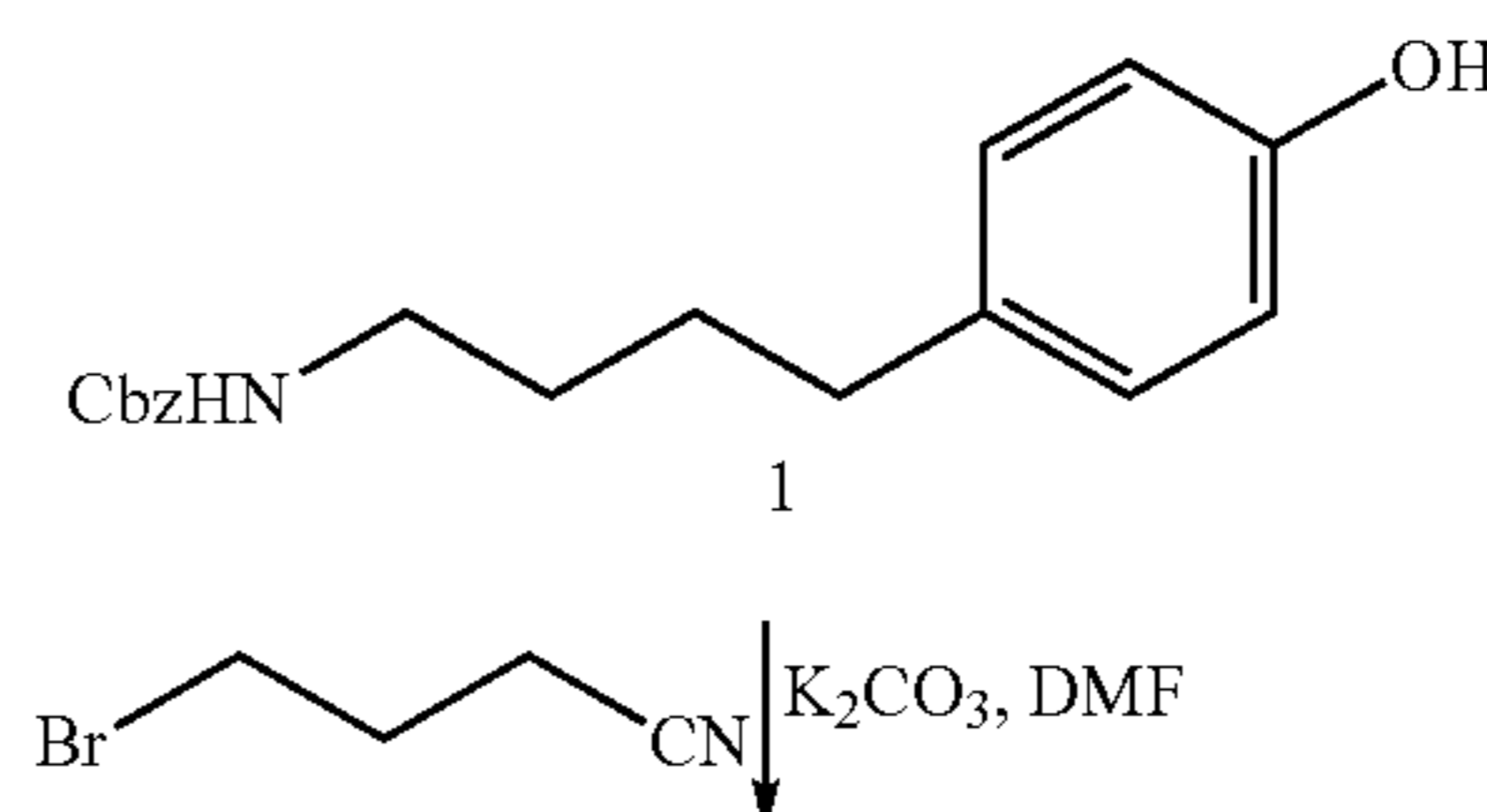
Scheme 1. Synthesis of PSA 17926
