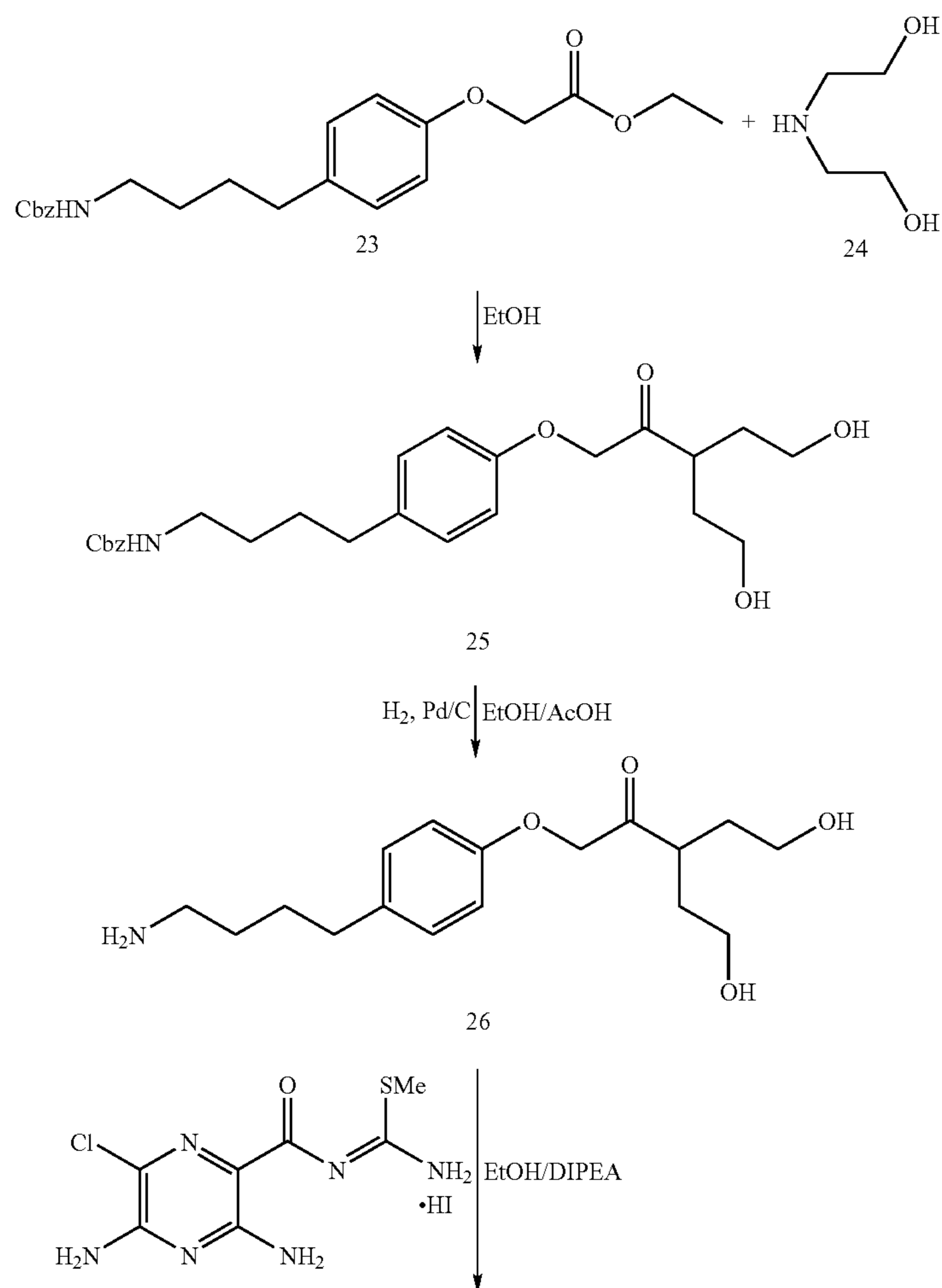
Scheme 6. Synthesis of PSA 16826
