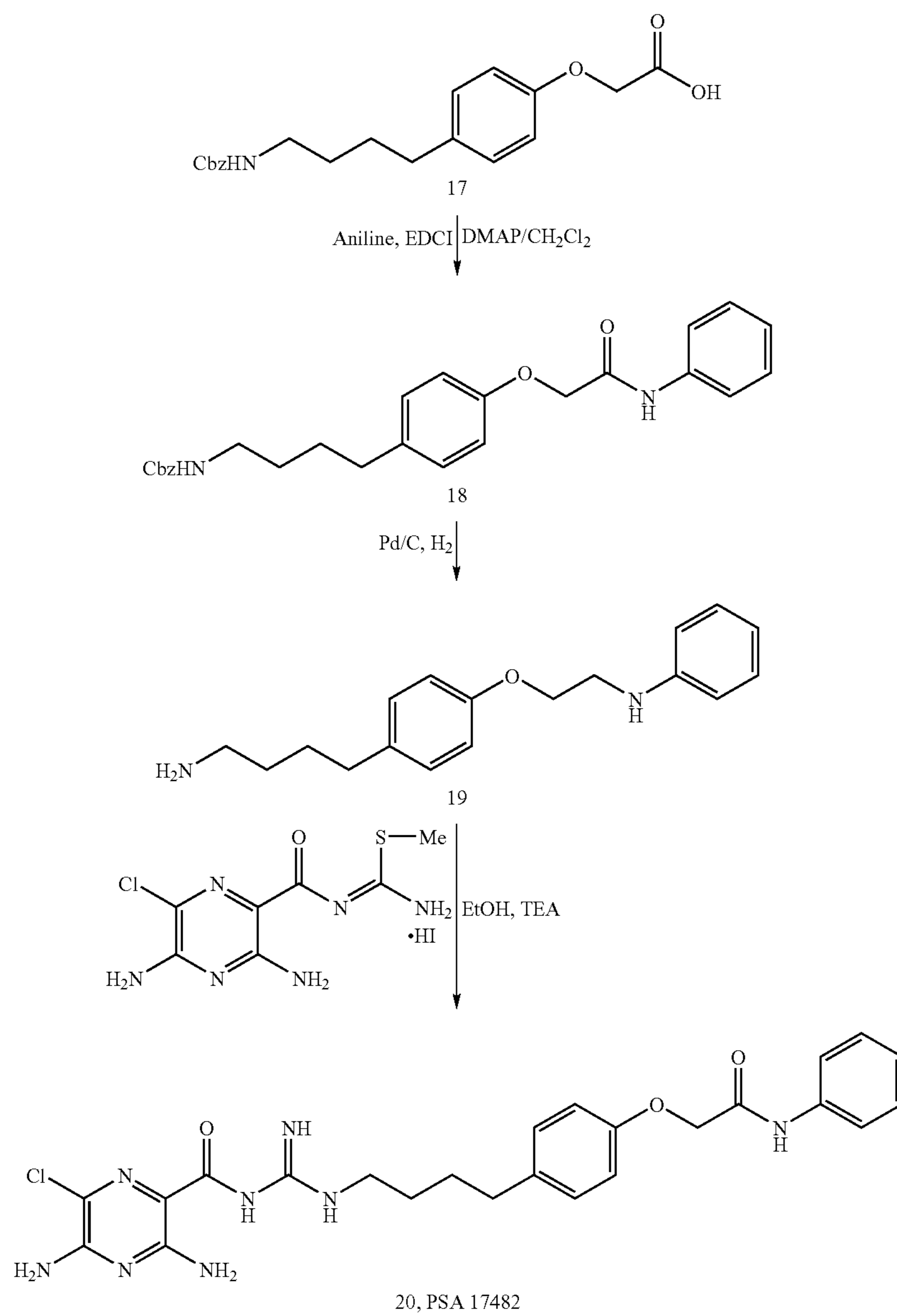
Scheme 4. Synthesis of PSA 17482
