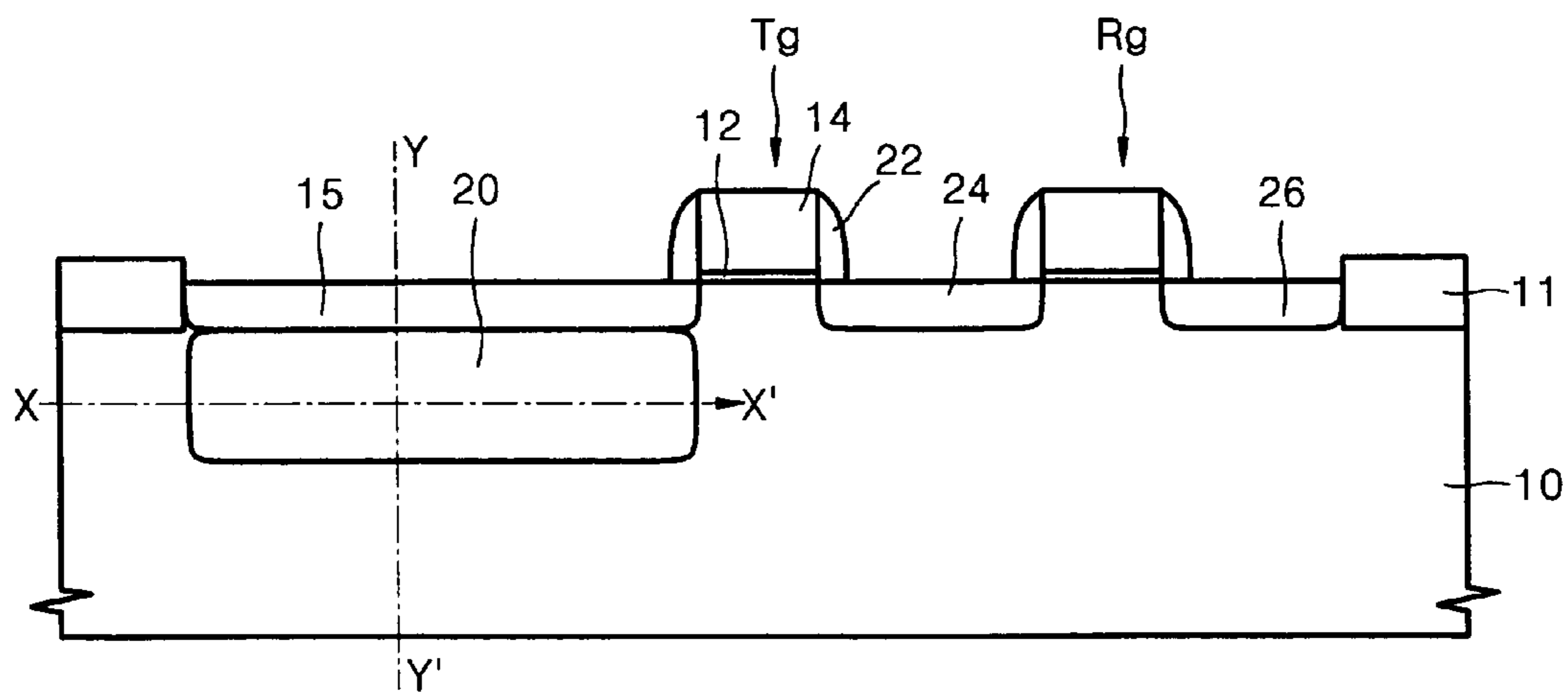
FIG. 2 (PRIOR ART)
