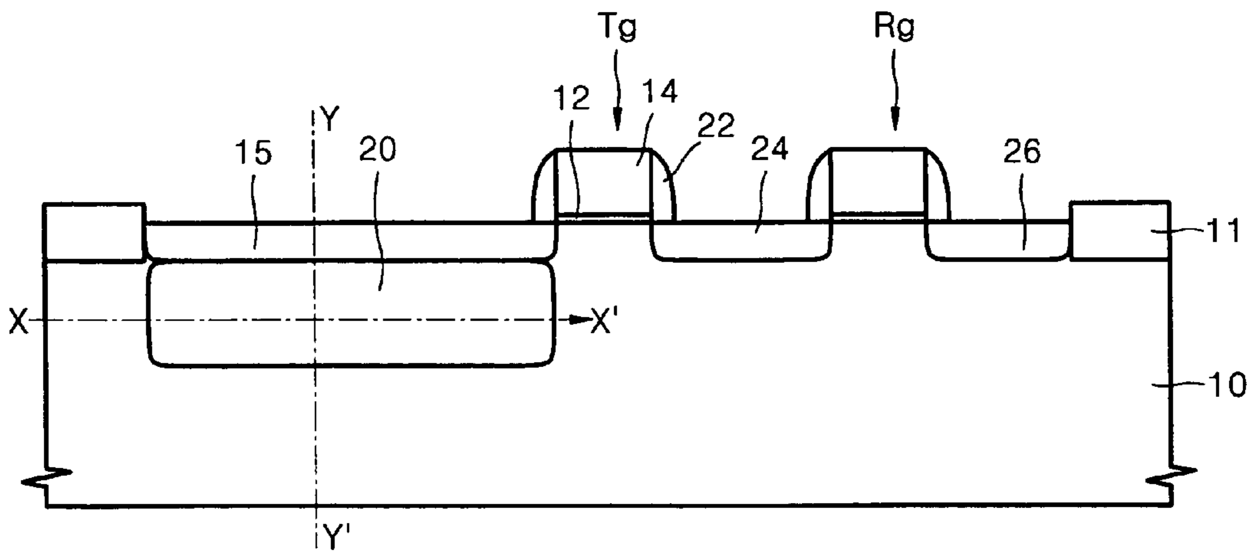
FIG. 2 (PRIOR ART)
