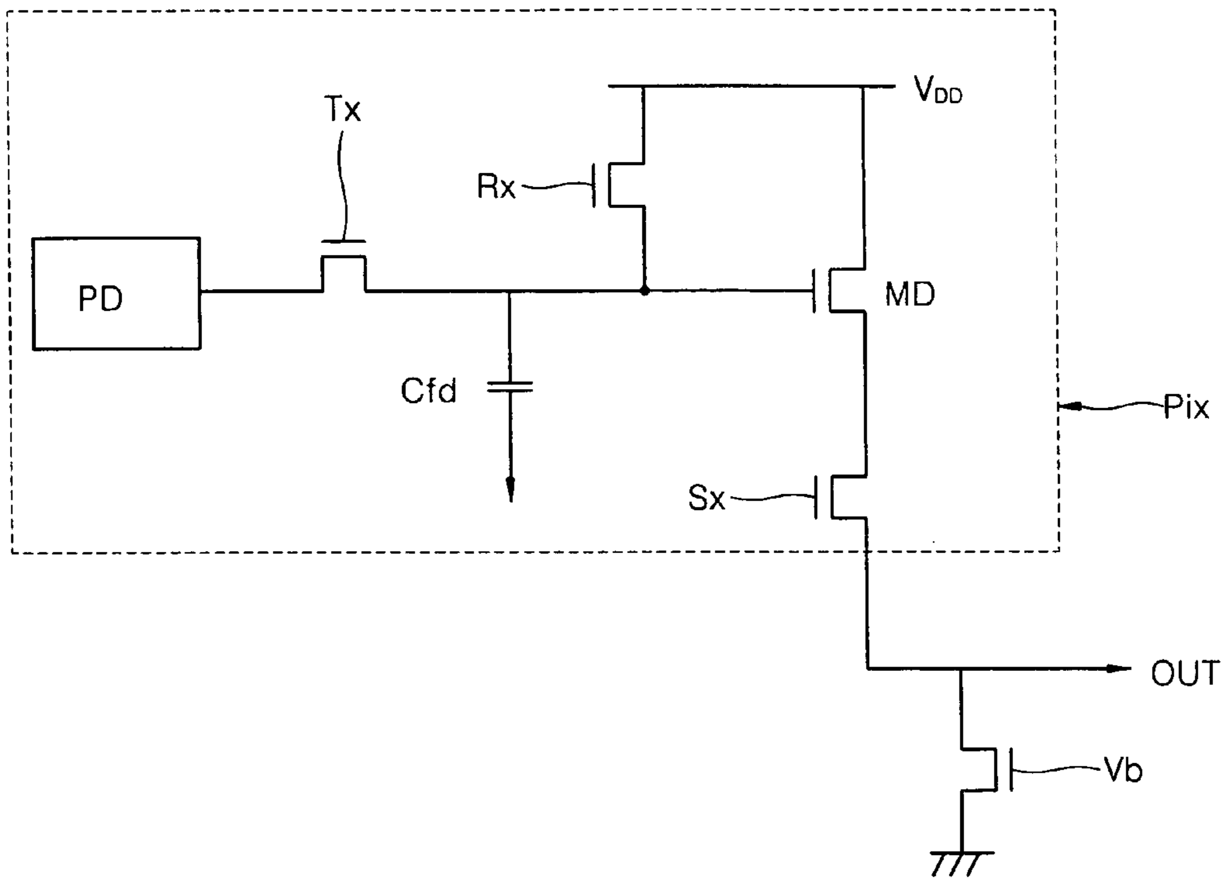
FIG. 2 (PRIOR ART)
