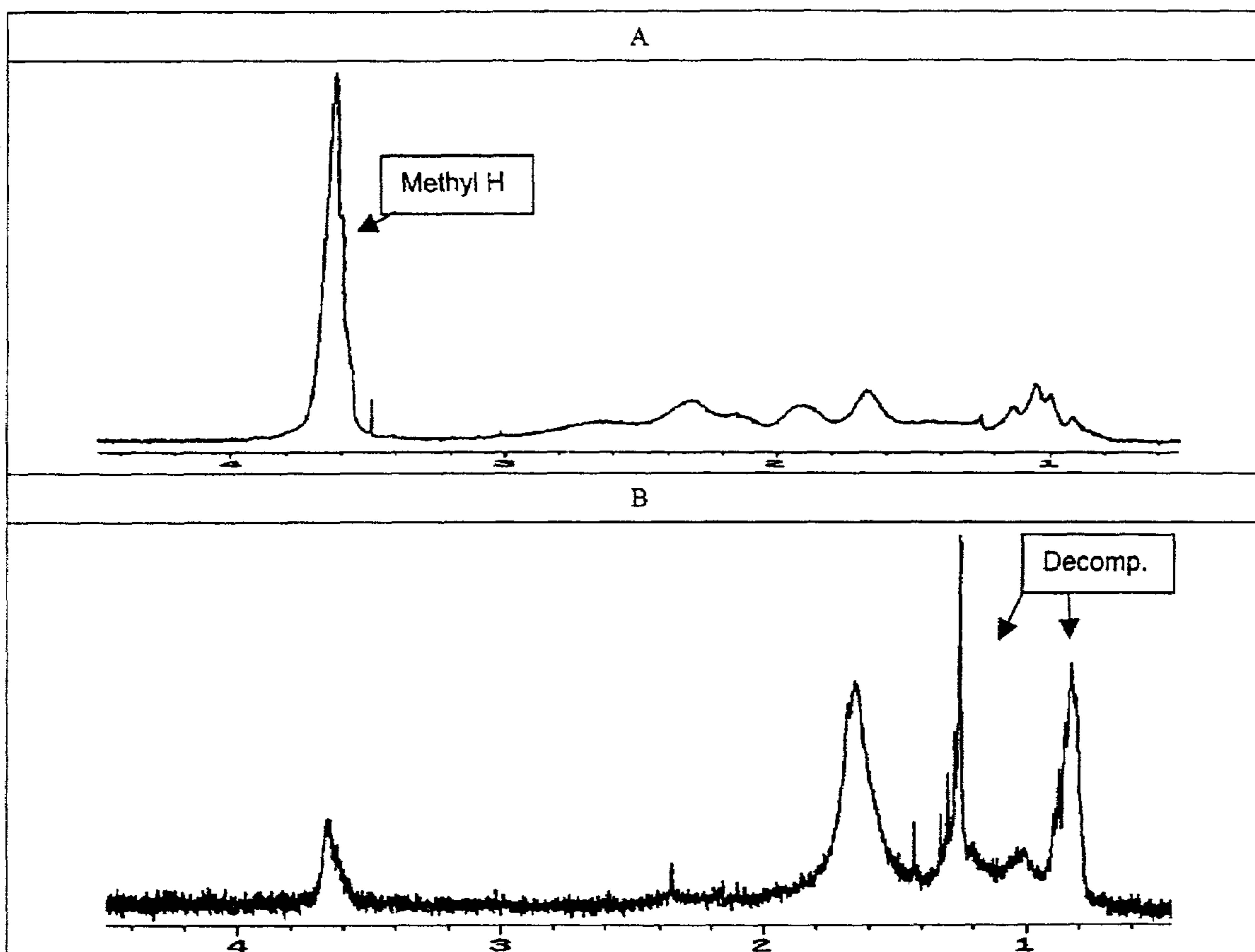
Figure 14 1 H-NMR spectra of A) original Eudragit 4135, B) deposited Eudragit at 200 mJ near atmospheric pressure (10 Torr).
