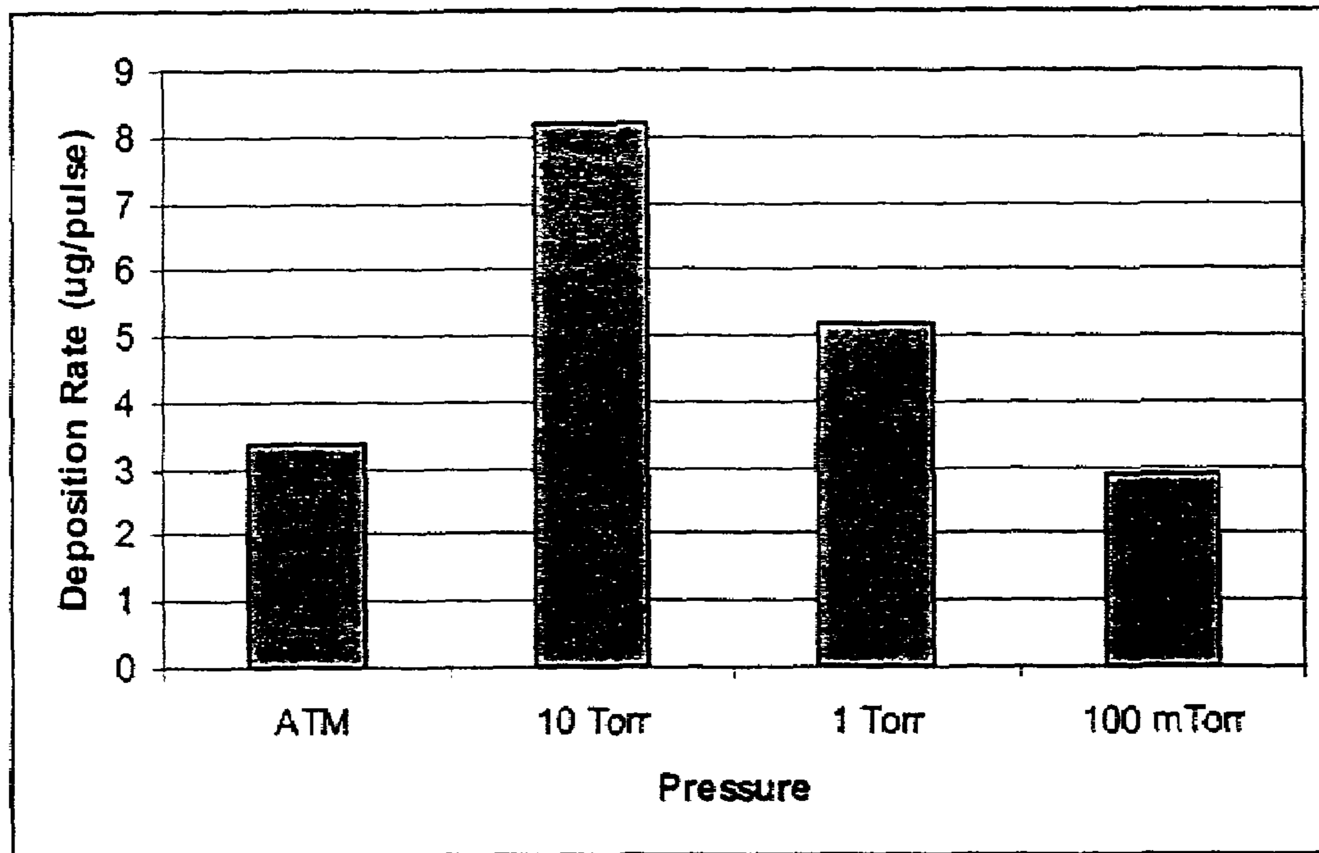
Figure 6 PLGA deposition rate at different pressures.
