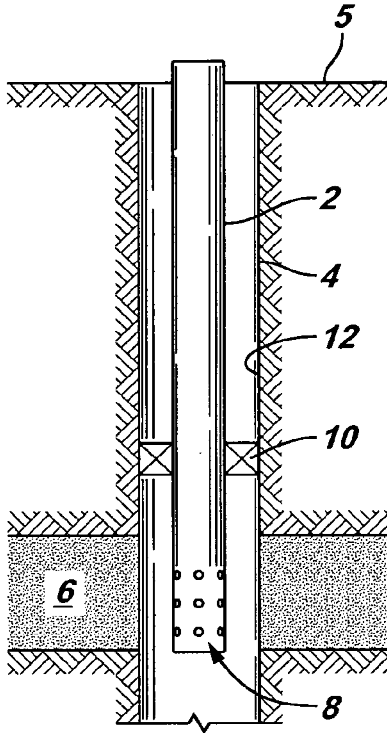
FIG. 1 (Prior Art)
