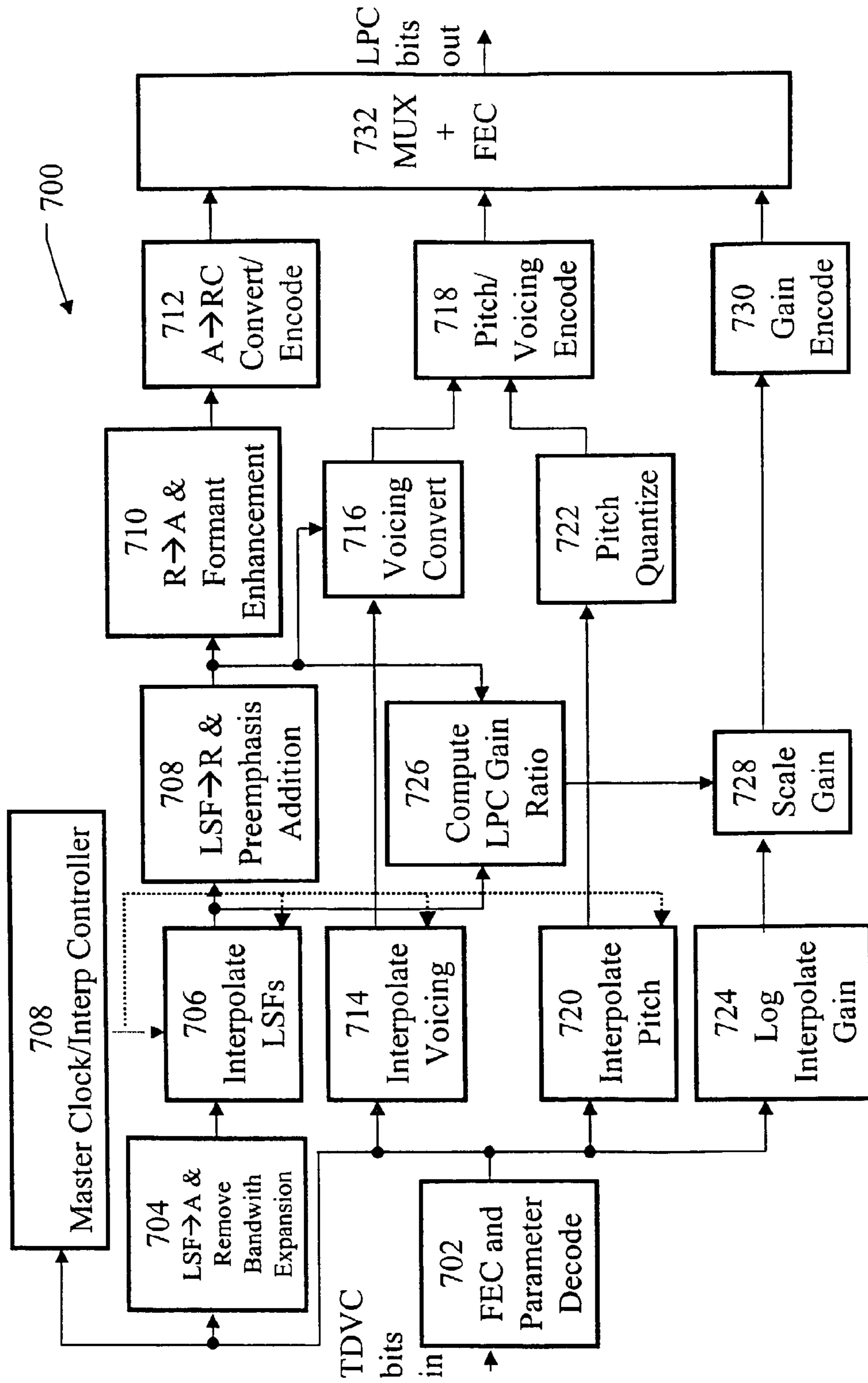
Figure 7: TDVC to LPC-10 Transcoder
