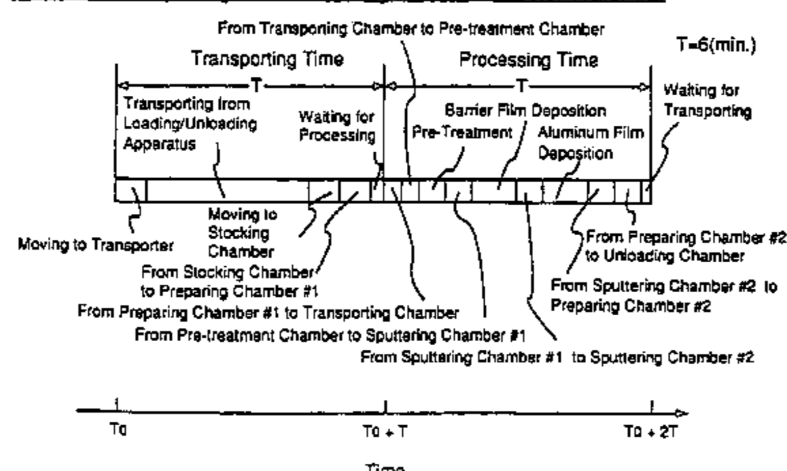
Details of Transporting and Processing of Semiconductor Wafer #2.
