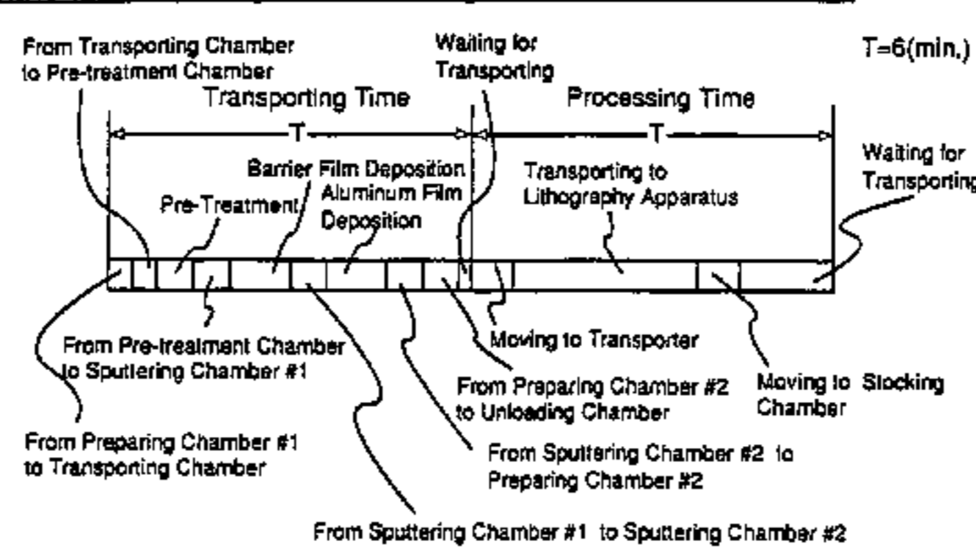
Details of Transporting and Processing of Semiconductor Wafer #2.
