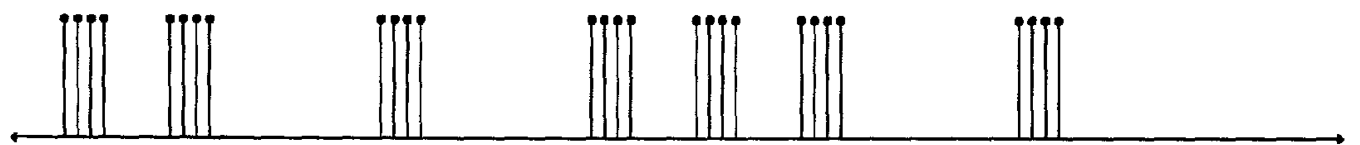
FIGURE 2g - Sample of Fixed Burst Time, Off Time Modulated Waveform
