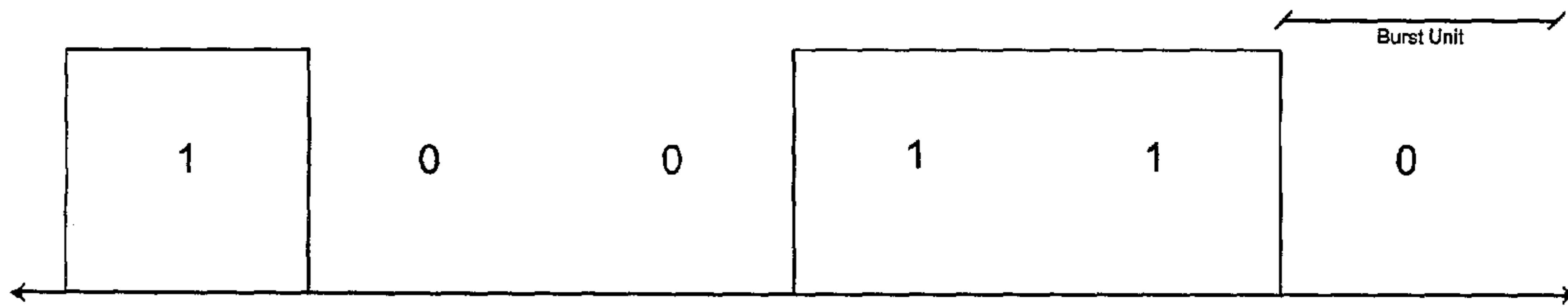
FIGURE 2a - Fixed Bit Time, Full Width Burst
