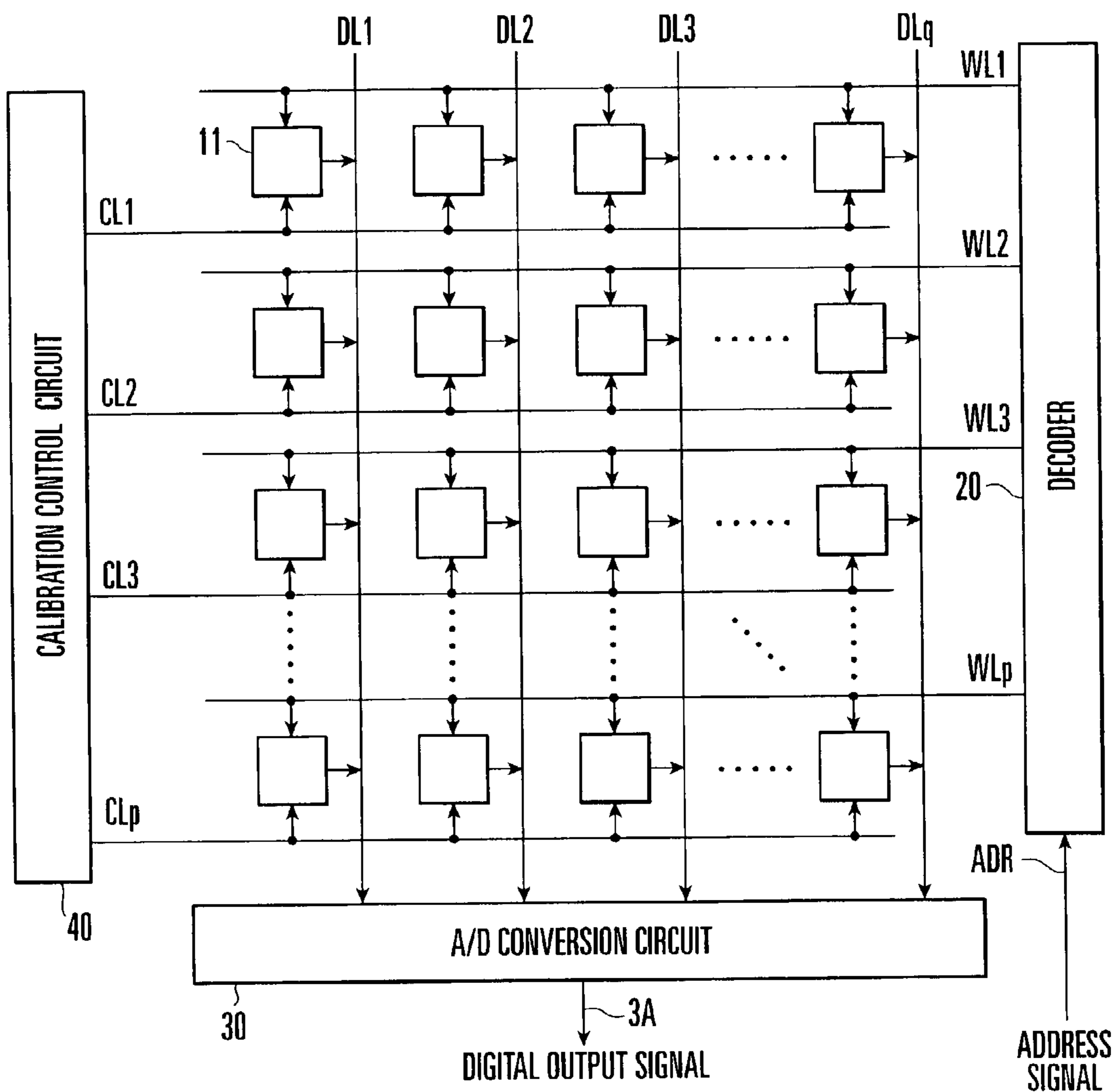
FIG. 11 PRIOR ART
