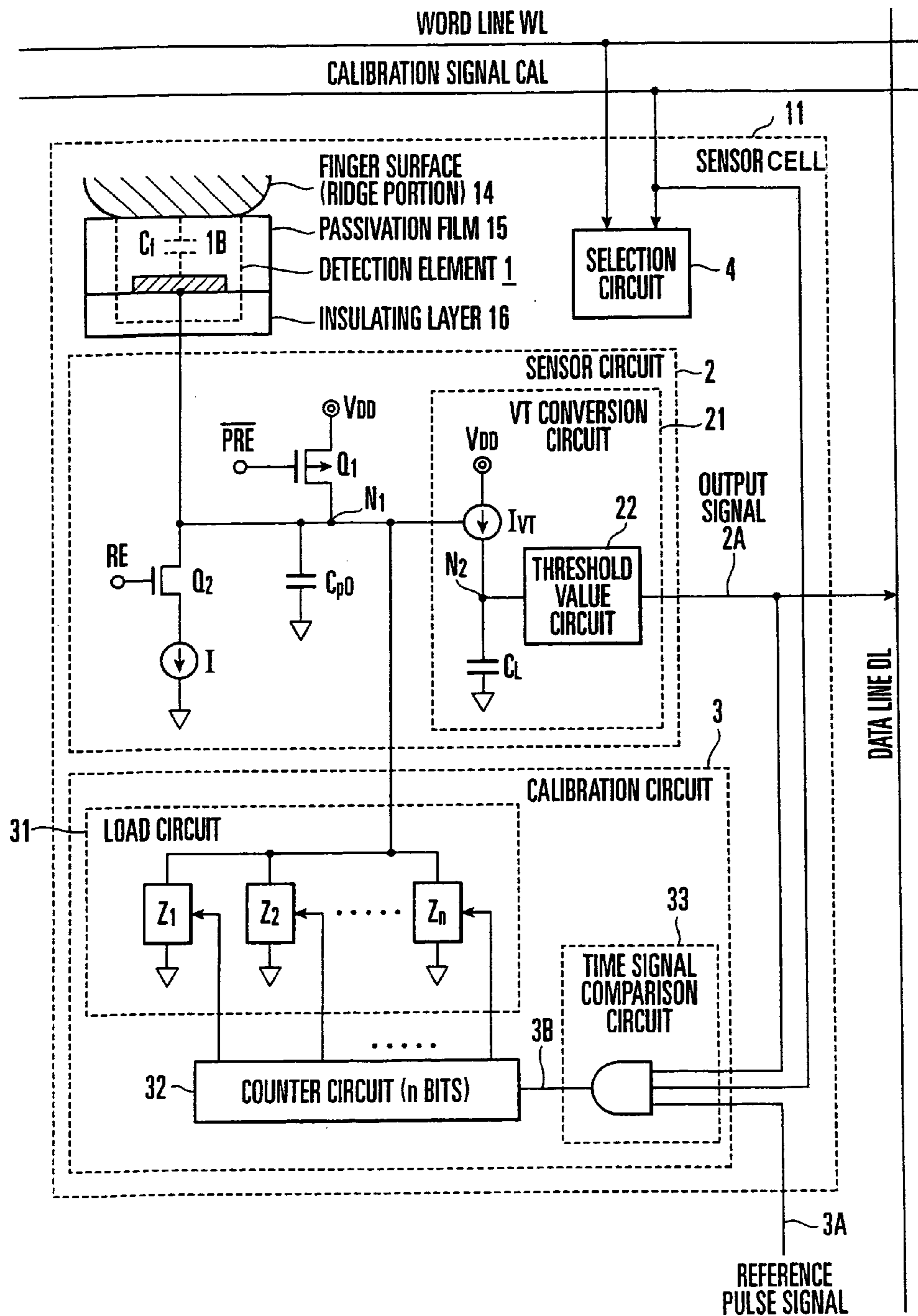
FIG. 12 PRIOR ART
