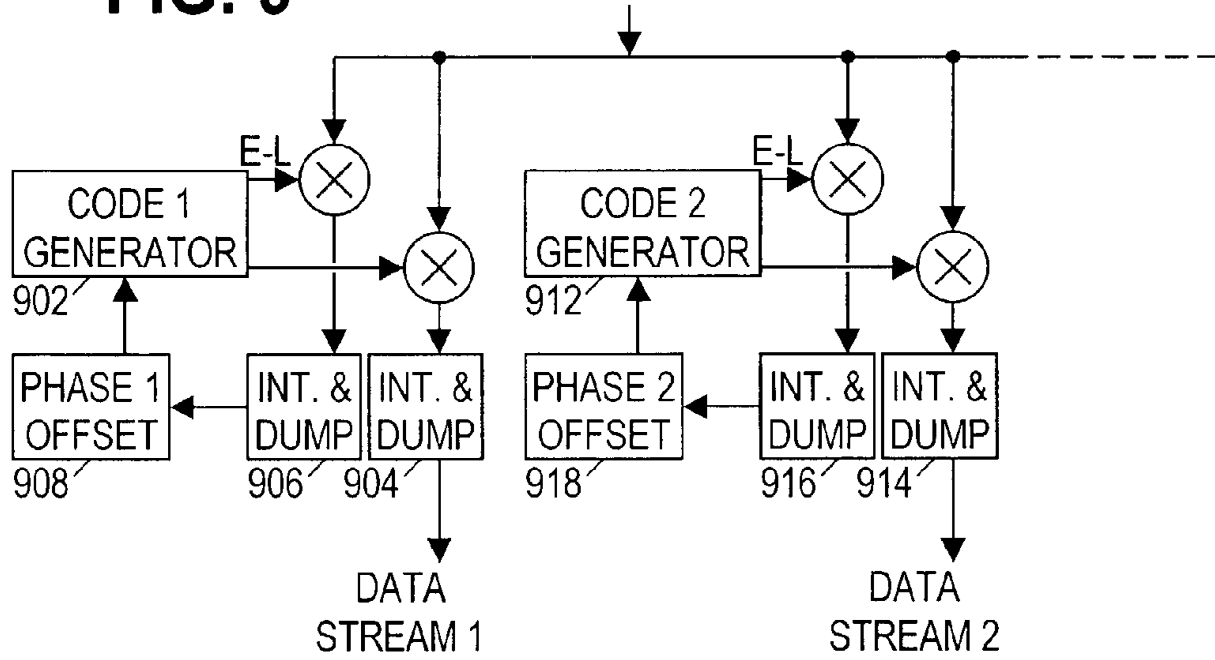
FIG. 9 COMPOSITE BASEBAND SIGNAL
