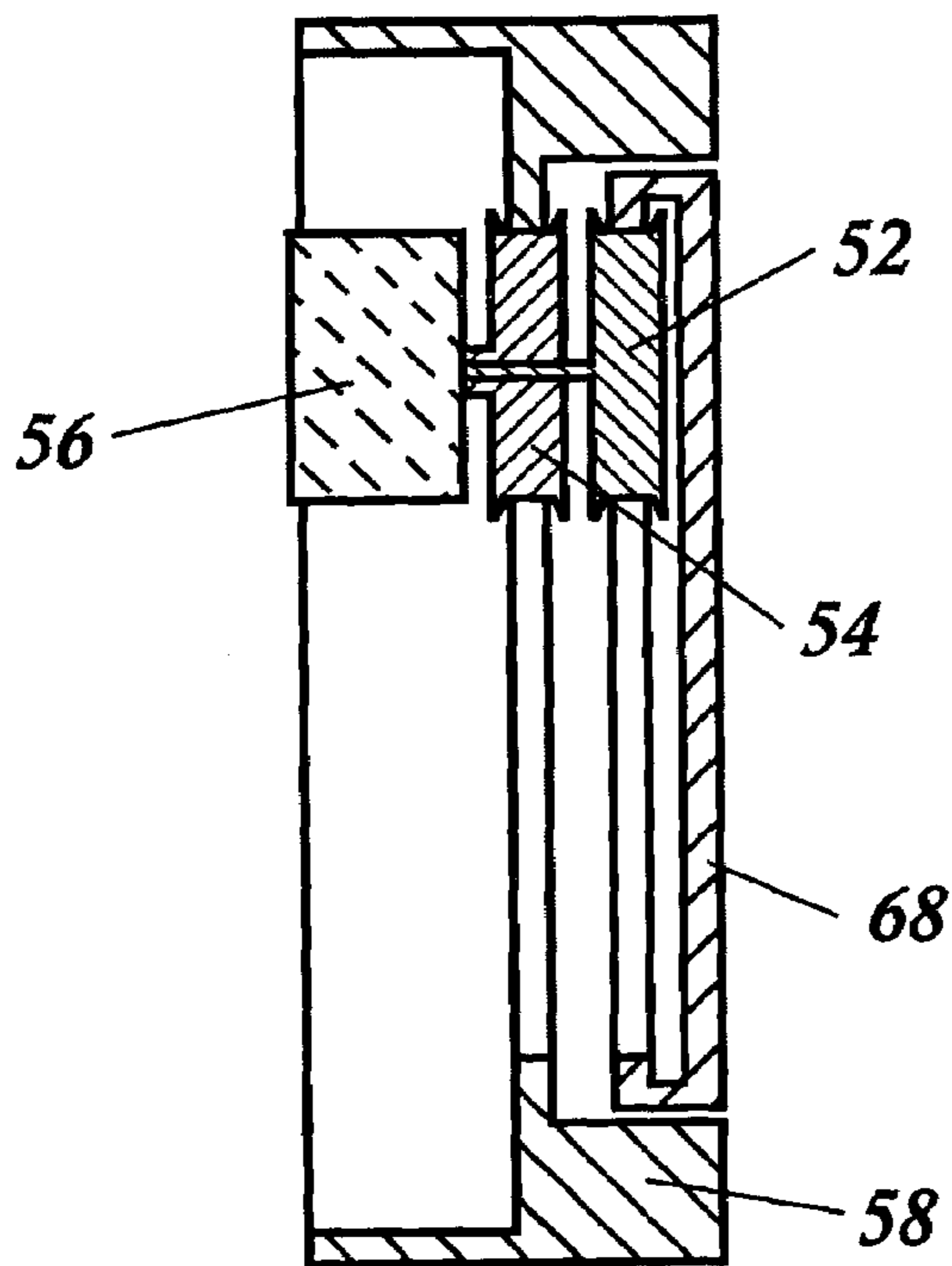
Section F-F FIG. 12
