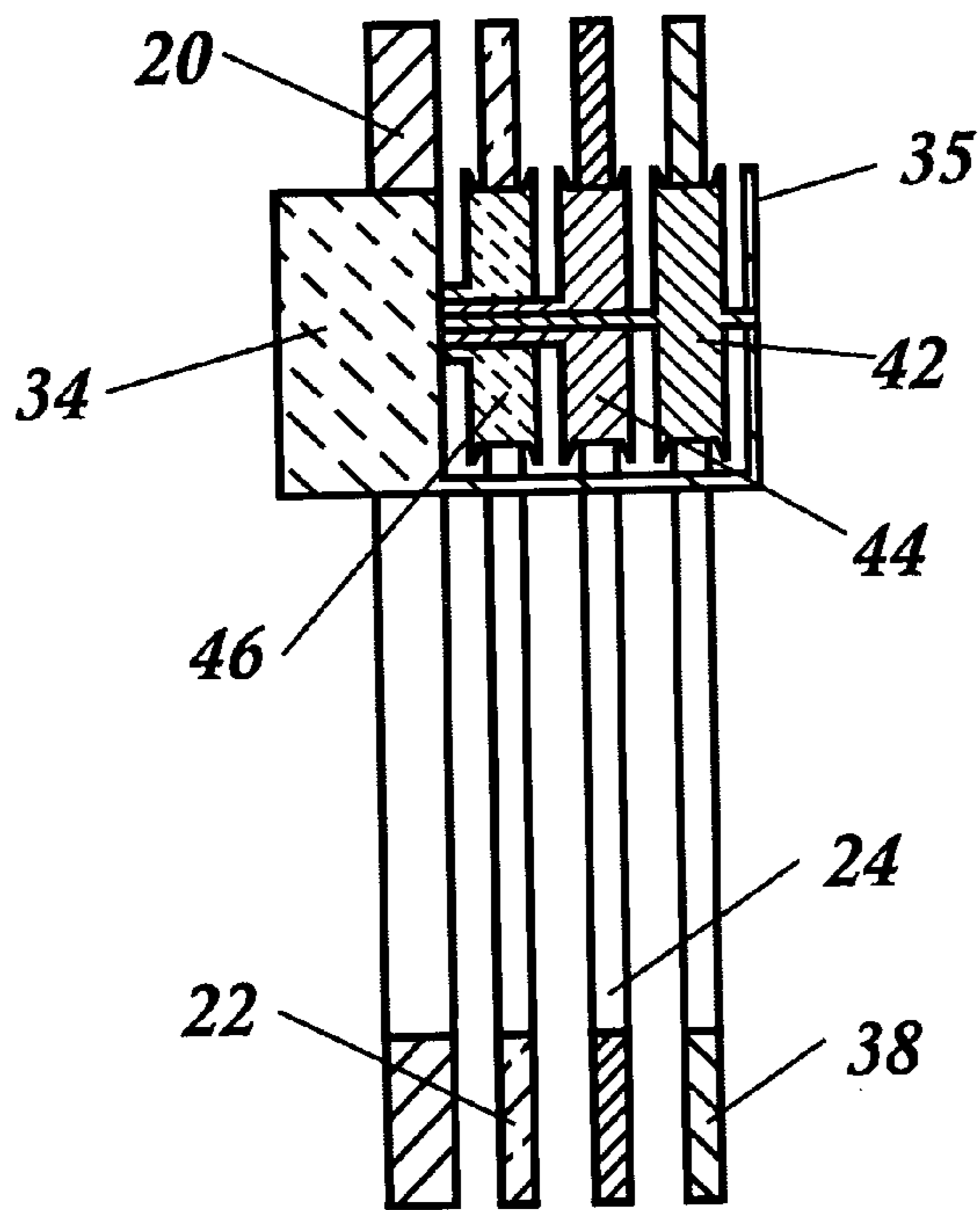
Section B-B
