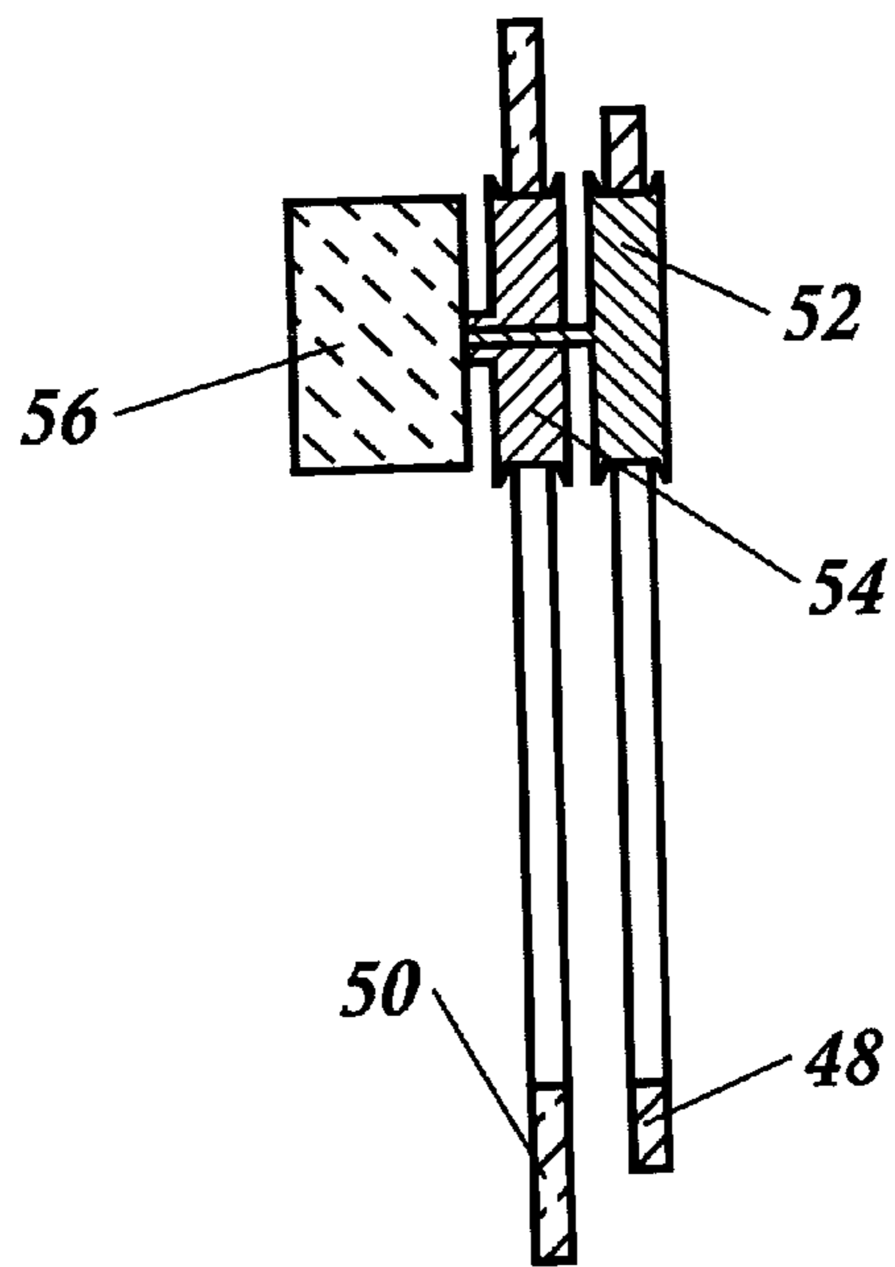
Section C-C
