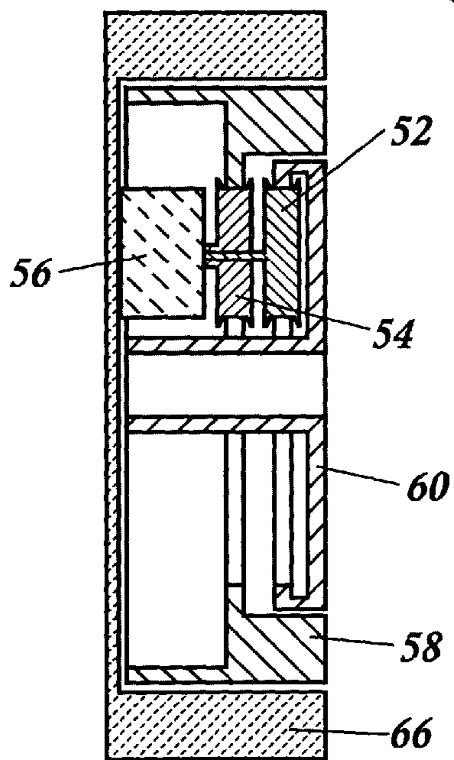
Section E-E
