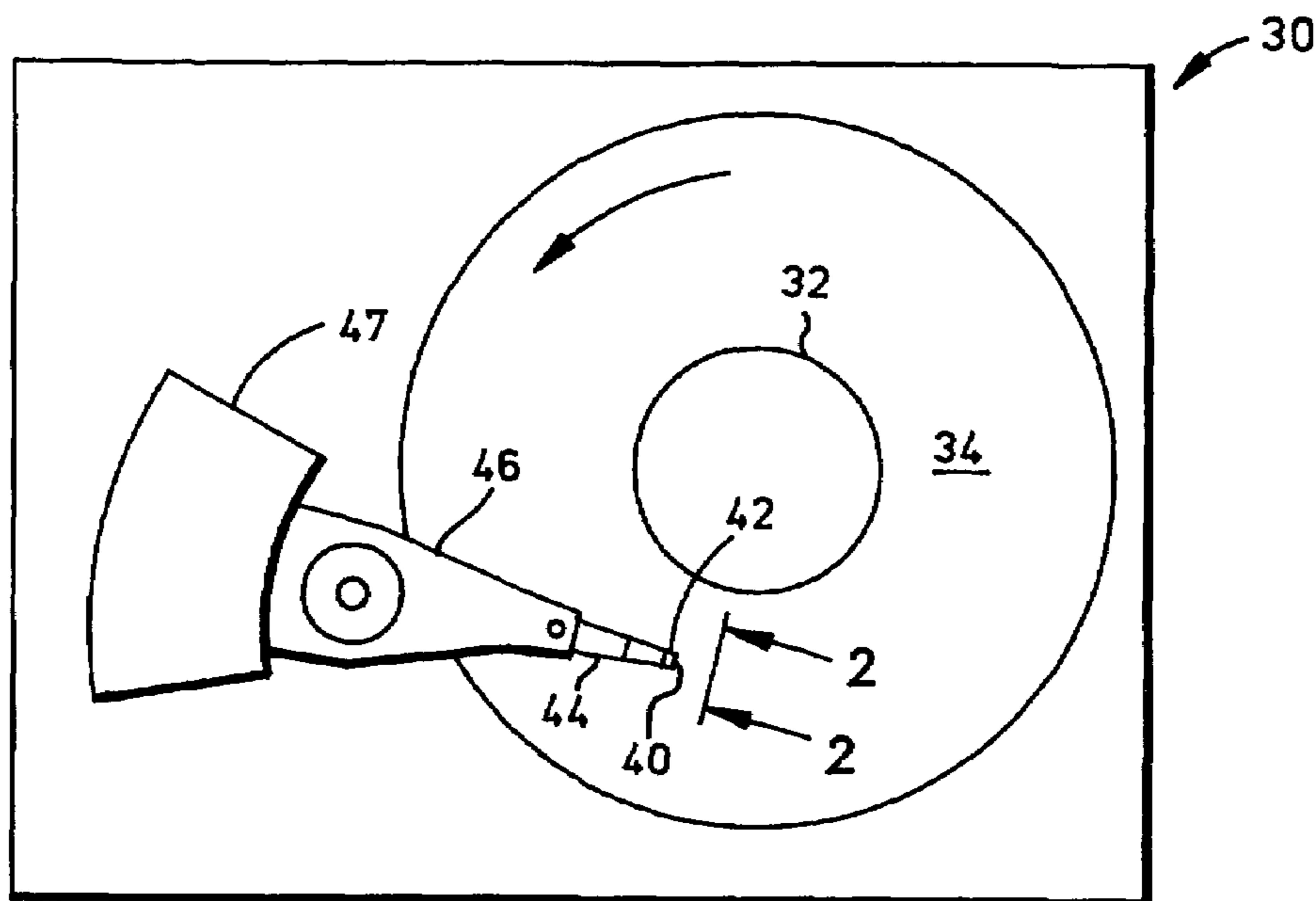
FIG. 1 (PRIOR ART)
