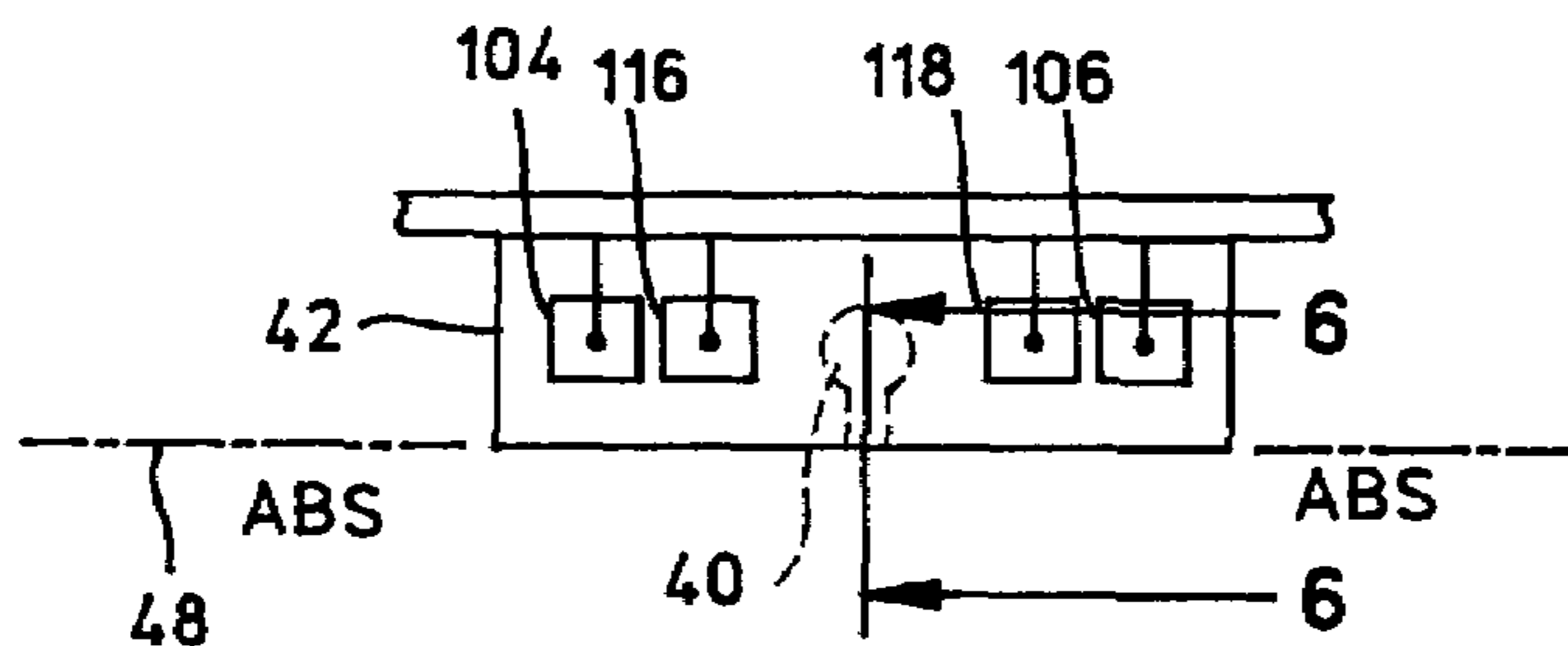
FIG. 1 (PRIOR ART)
