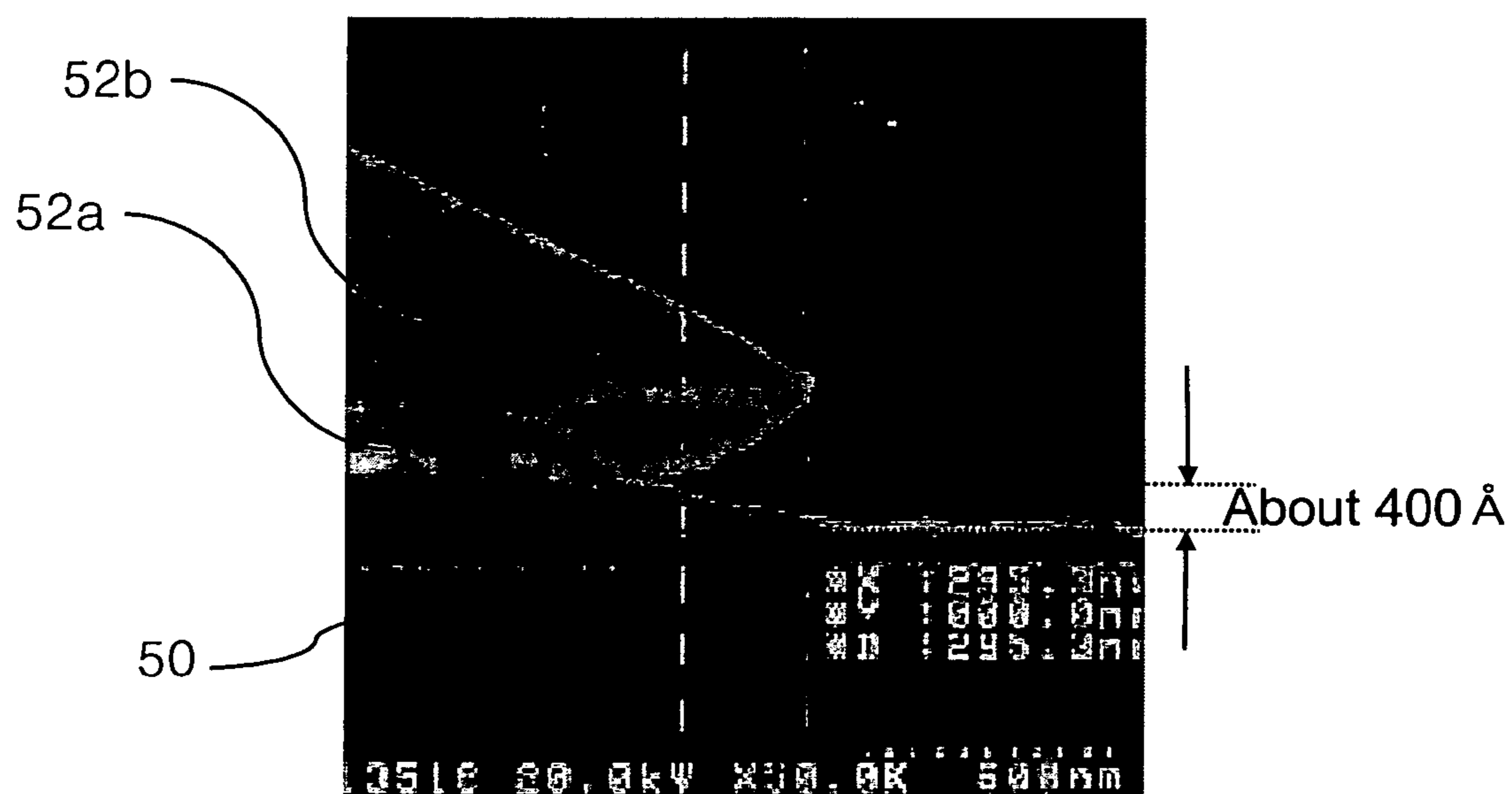
FIG. 4 (RELATED ART)
