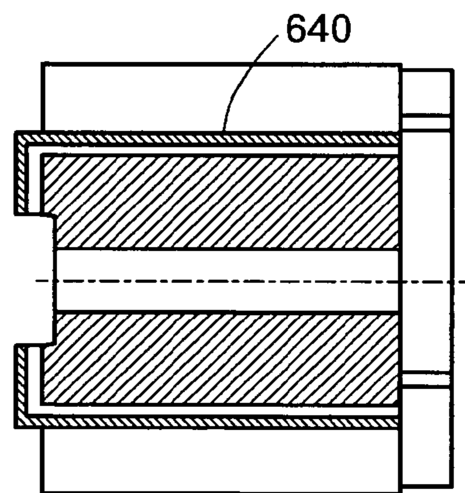
SECTION B-B
