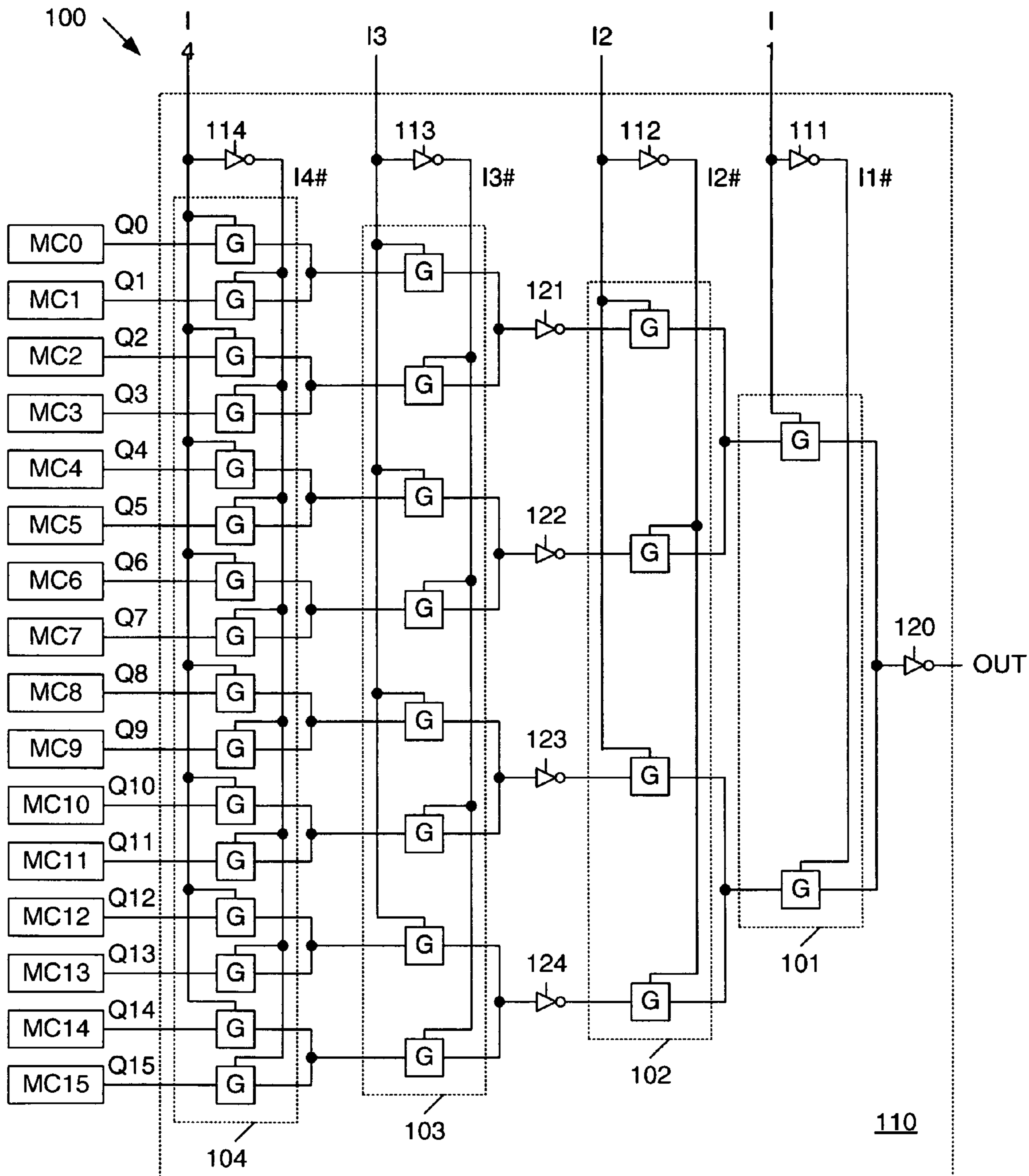
FIG. 1 (PRIOR ART)
