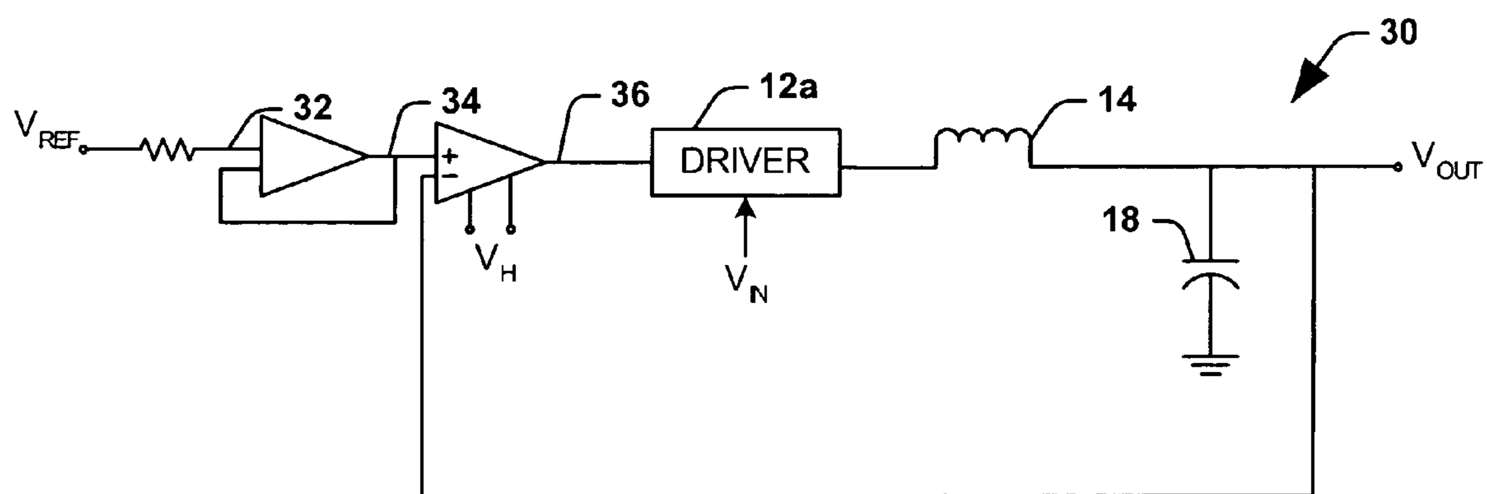
FIG. 3 (PRIOR ART)
