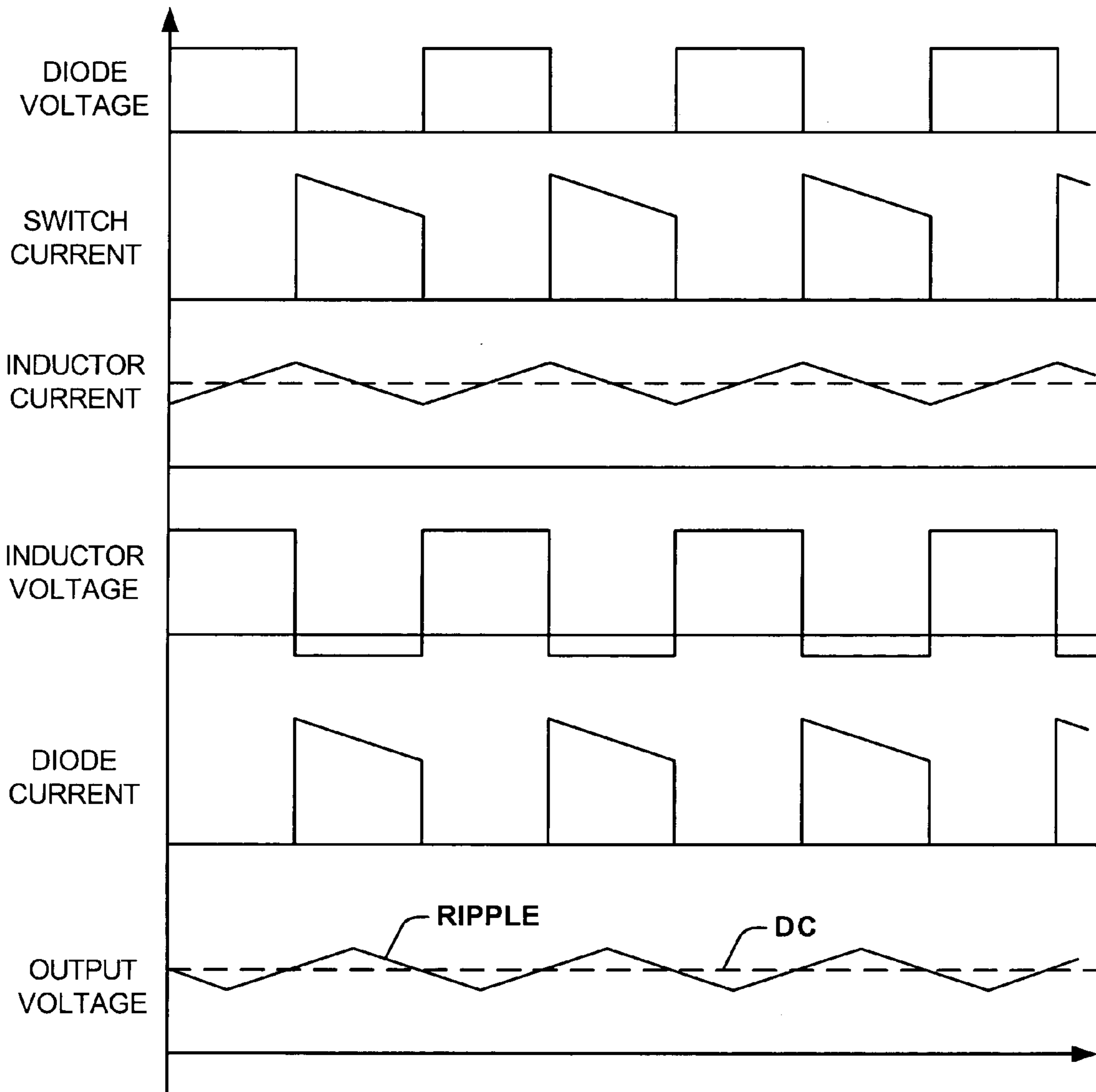
FIG. 2 (PRIOR ART)
