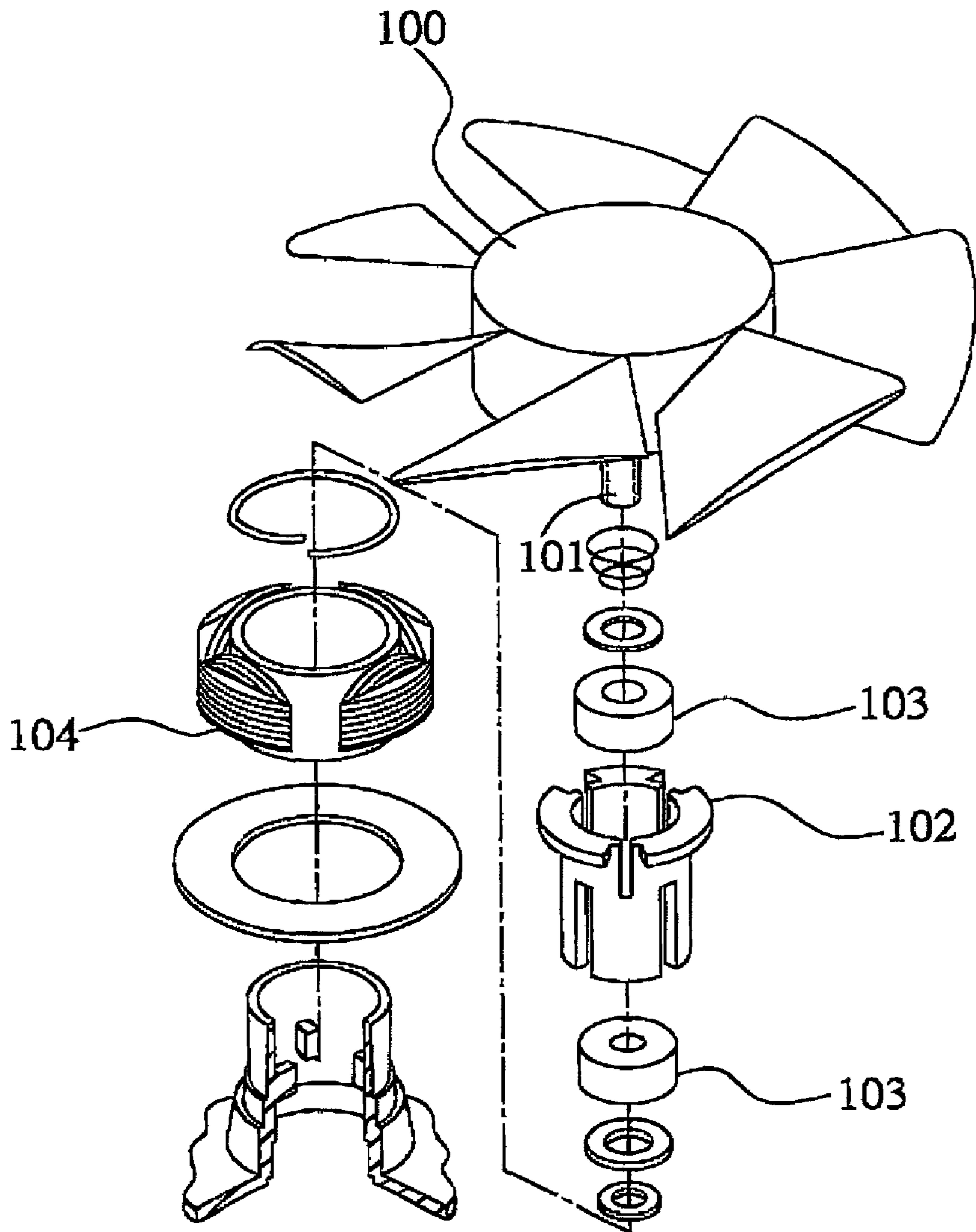
FIG. 1 PRIOR ART
