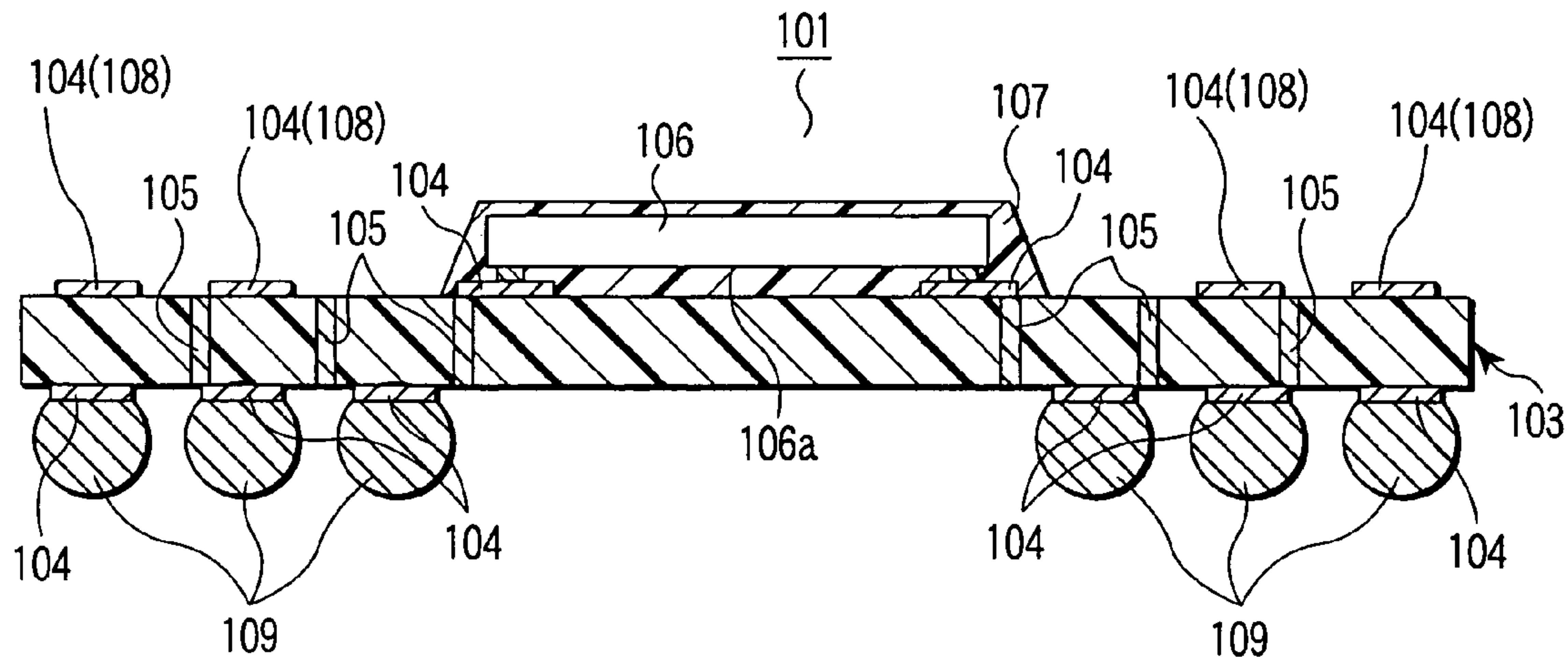
FIG. 24 PRIOR ART
