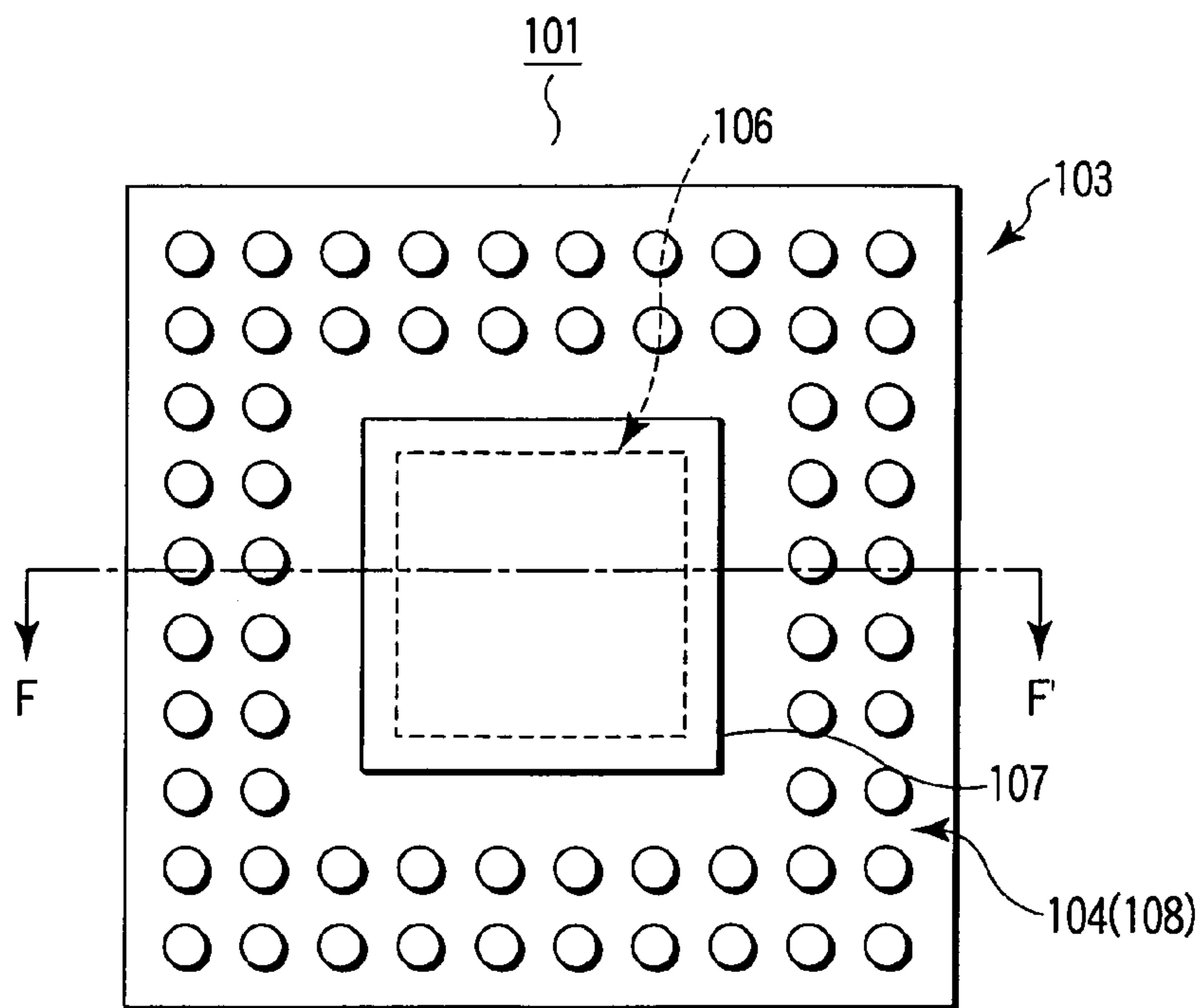
FIG. 25 PRIOR ART
