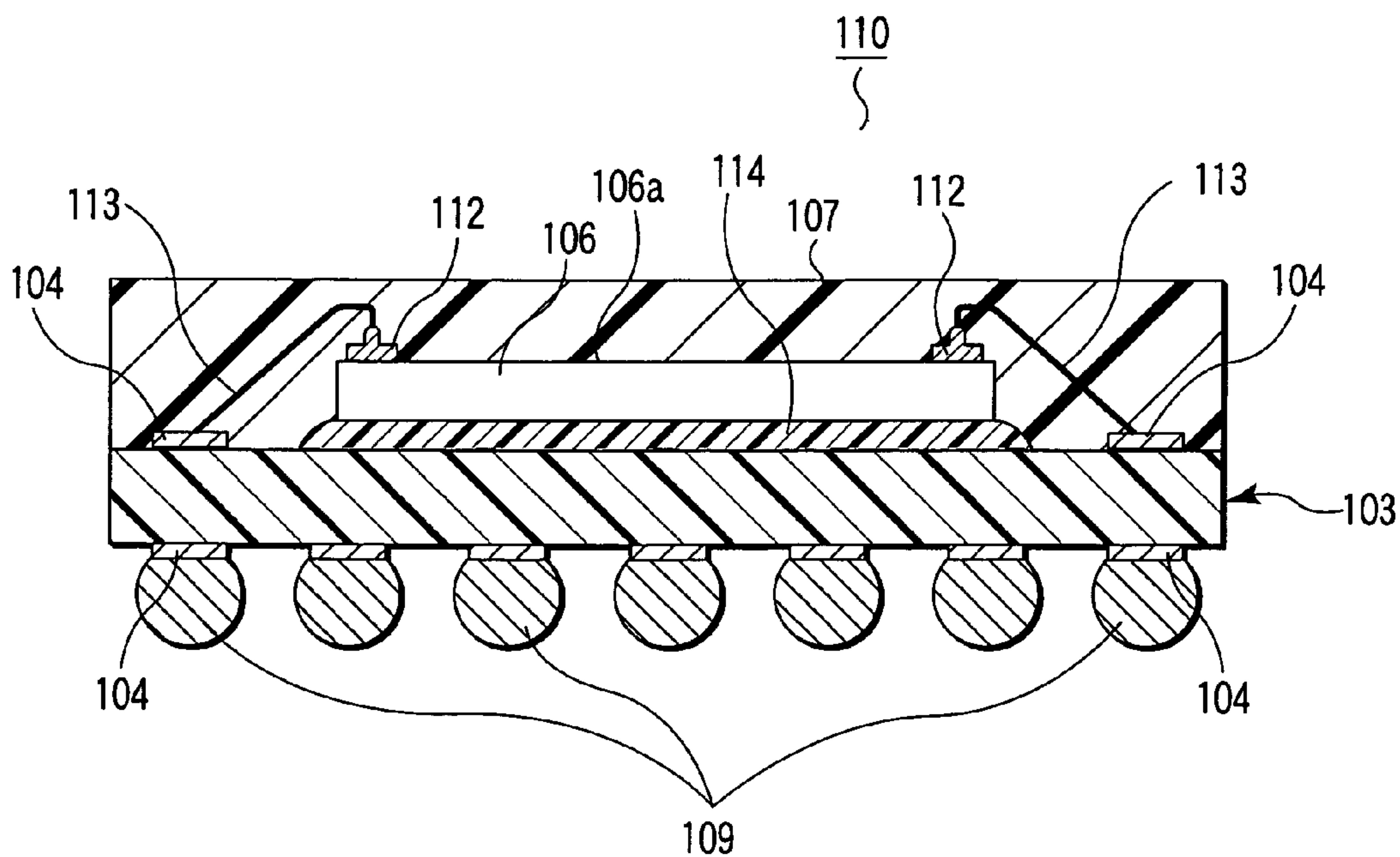
FIG. 27 PRIOR ART
