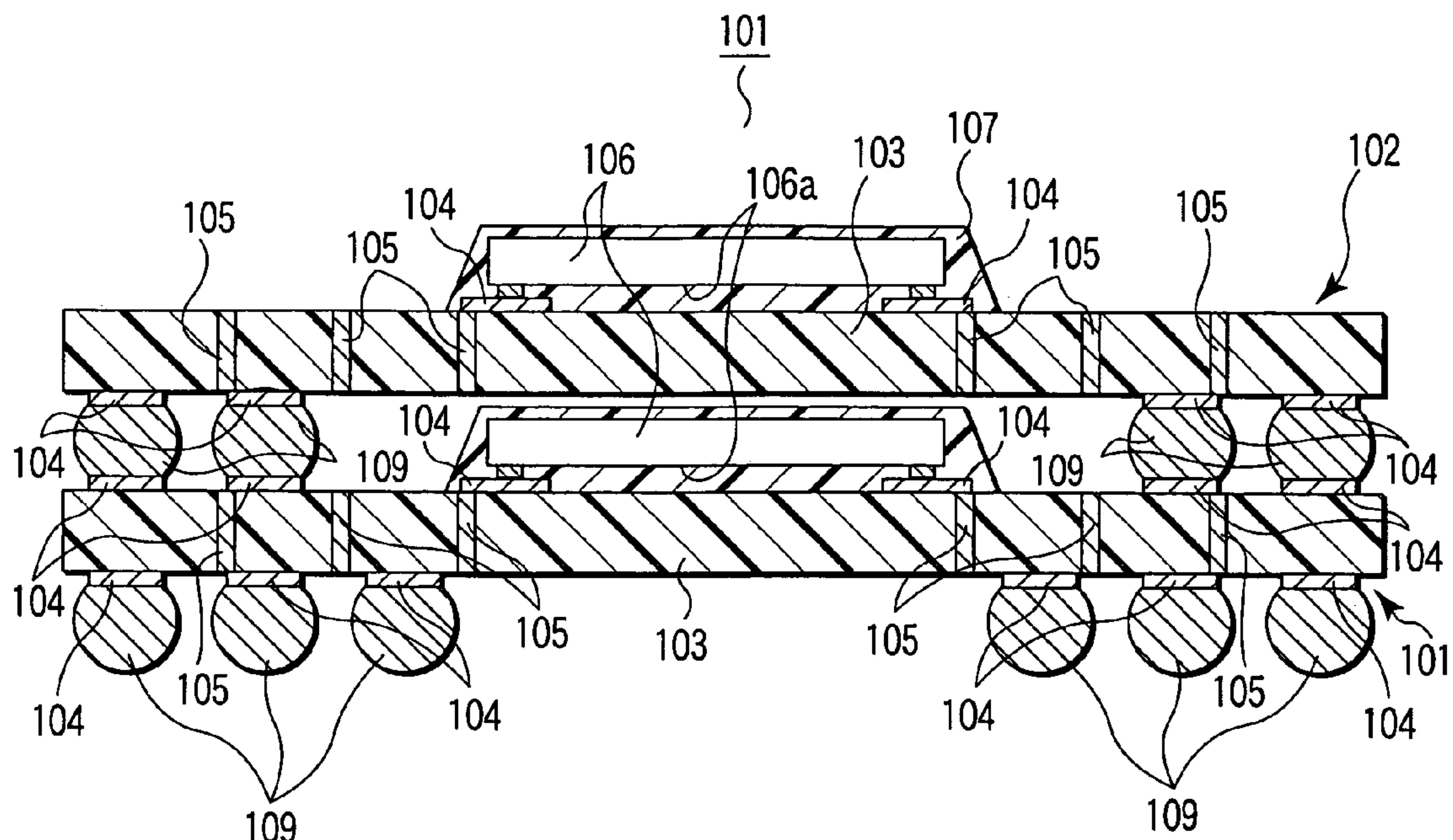
FIG. 26 PRIOR ART
