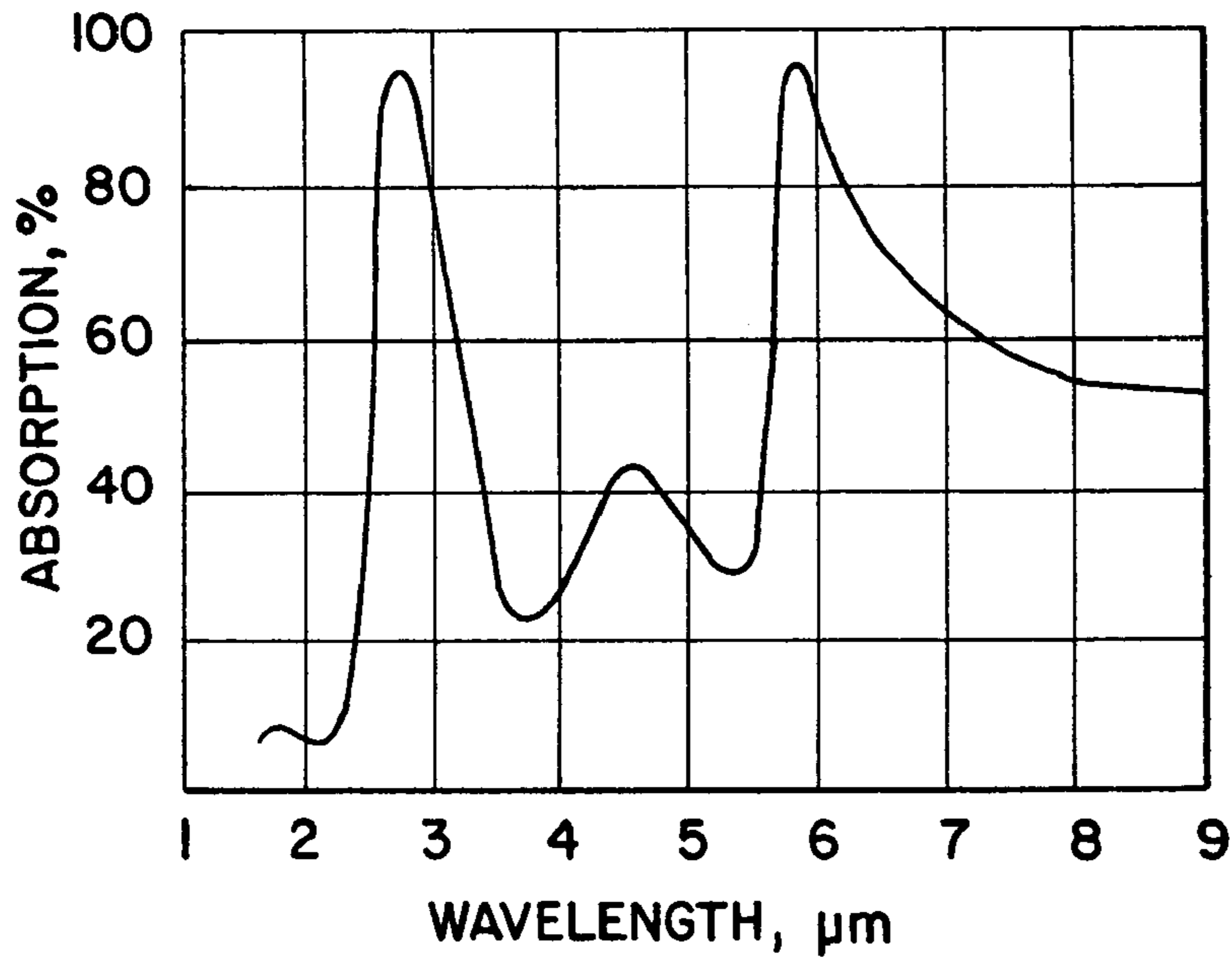
SPECTRAL ABSORPTION CURVE FOR WATER
